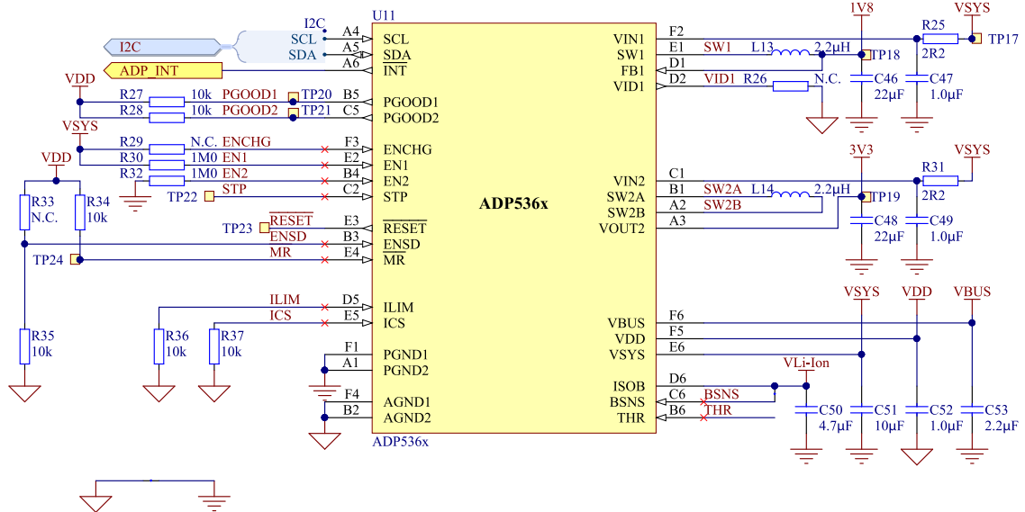
Figure 27: PMIC schematic
