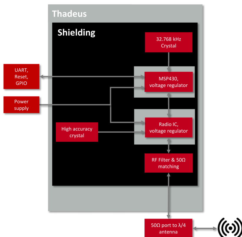
Figure 1: Block diagram
