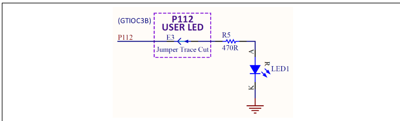
Figure 14. LED1 Control Circuit
