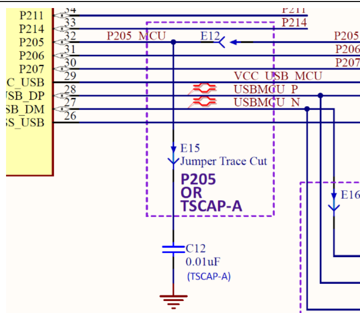
Figure 31. P205 Circuit
