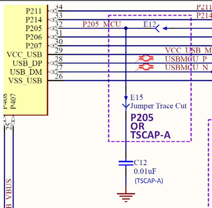
Figure 20. Capacitive Touch TSCAP Circuit
