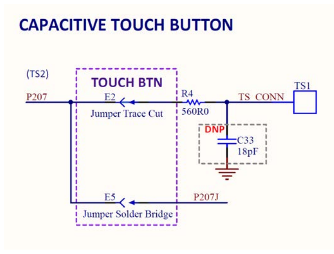
Figure 19. Capacitive Touch Button Circuit
