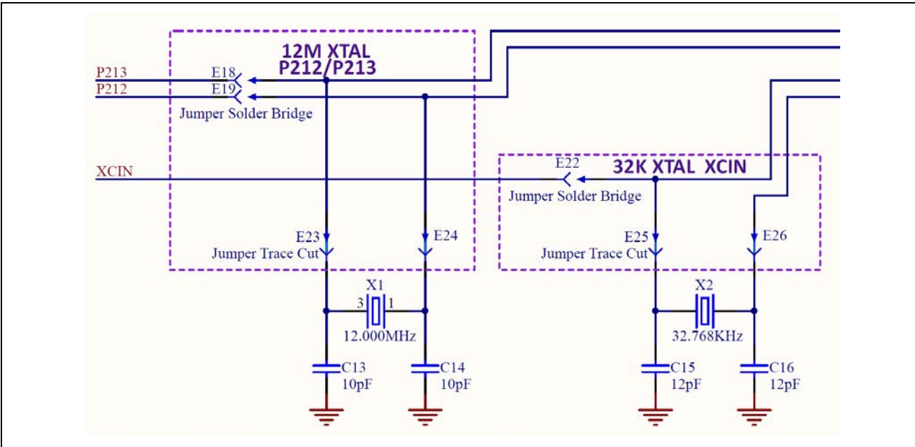
Figure 25. Crystal Clock Sources
