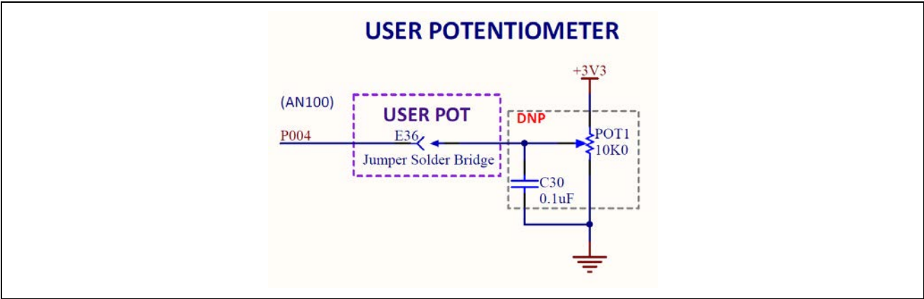
Figure 26. User Potentiometer Circuit
