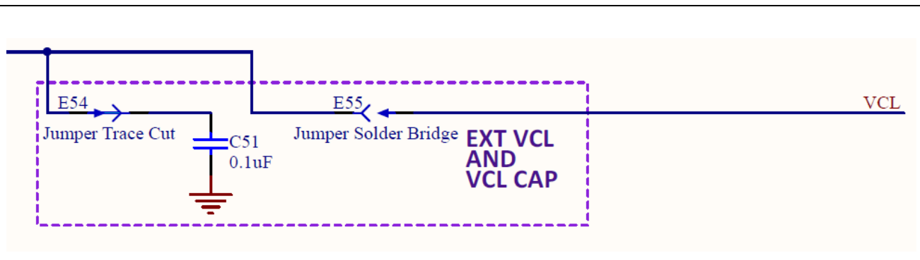
Figure 29. VCL and VCL Capacitor
