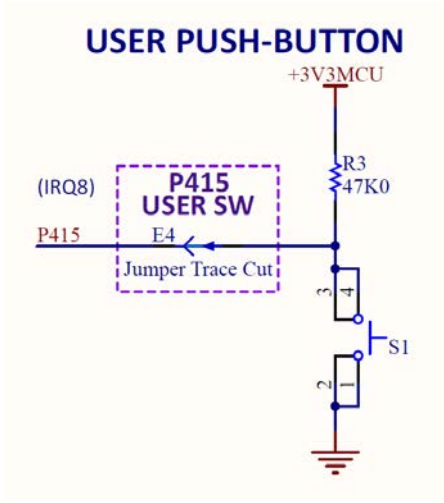
Figure 15. User Switch Circuit
