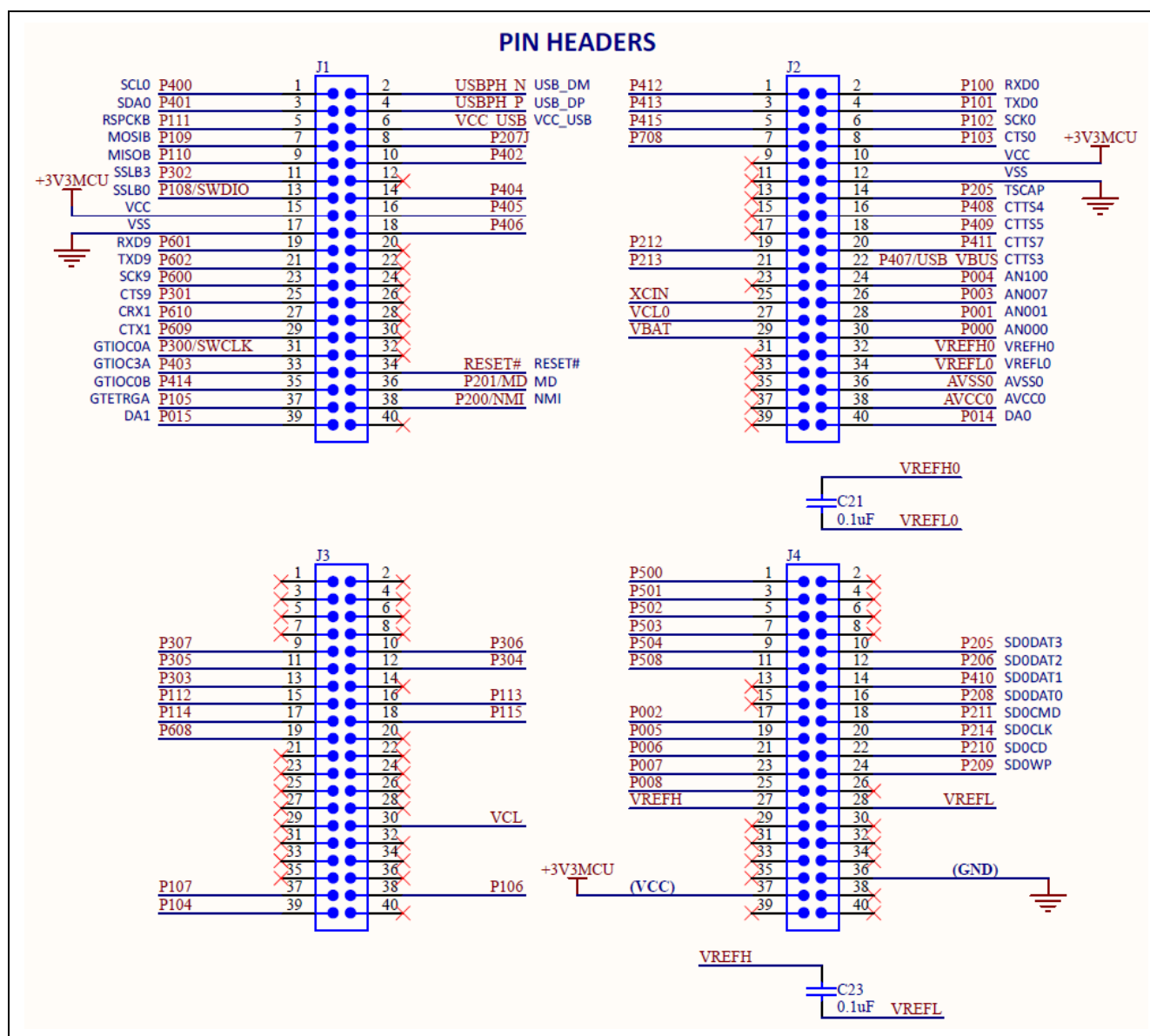
Figure 23. TB-S5D3 Pin Headers Circuit
