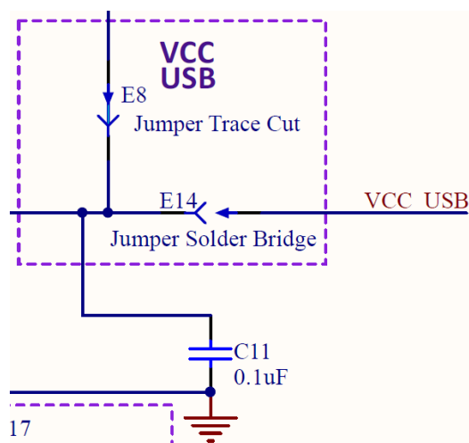
Figure 30. VCC_USB Circuit
