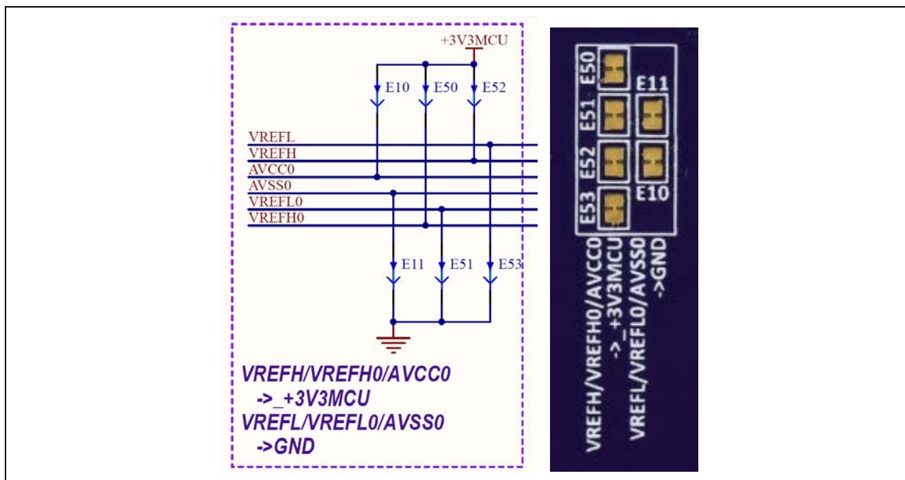
Figure 24. Analog and Reference Voltages
