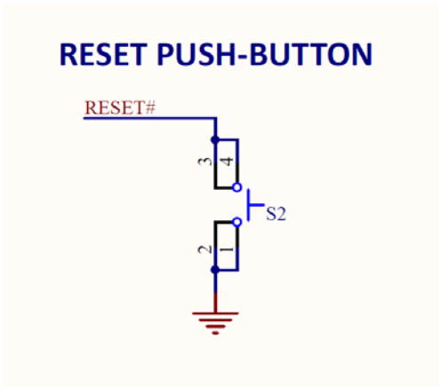
Figure 17. Reset Switch Circuit
