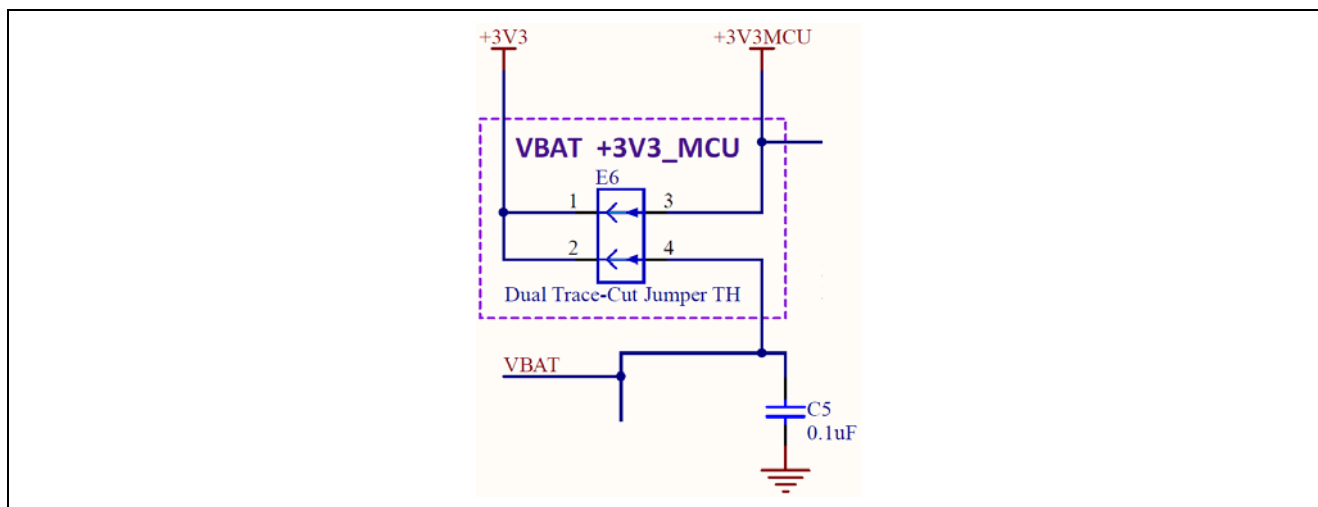
Figure 11. MCU Current Measurement Circuit
