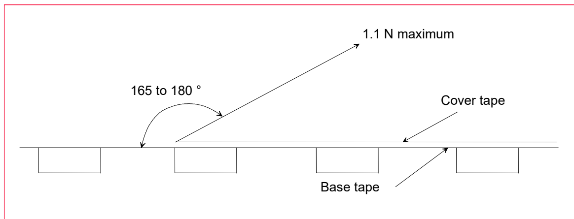
Figure 9: Peeling Force
