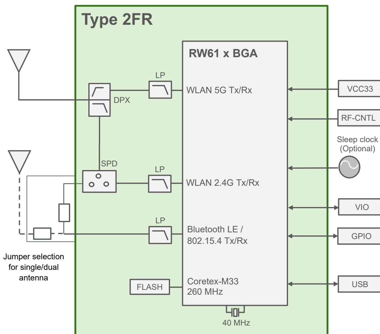
Figure 1: Block Diagram
