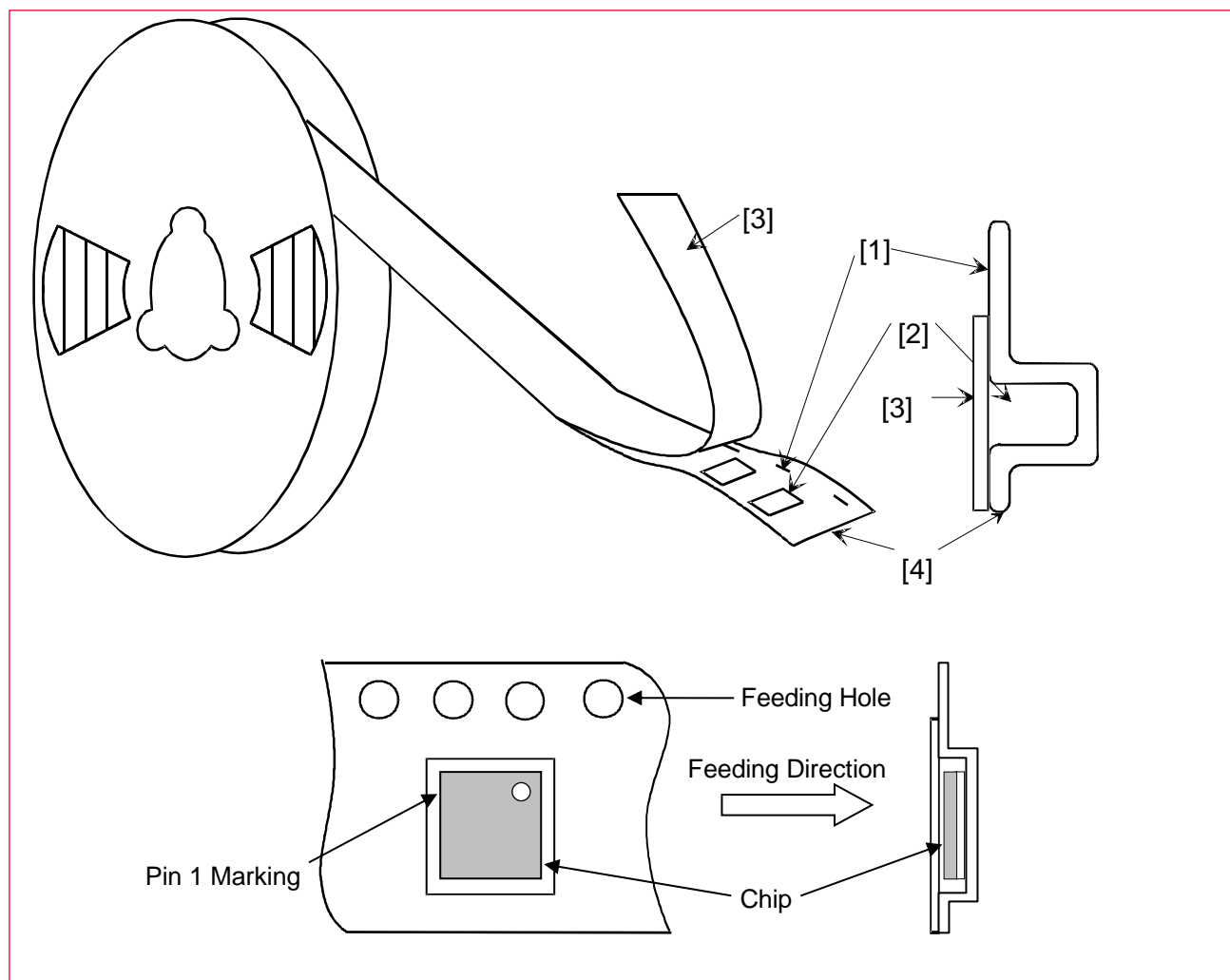
Figure 11: Taping Diagrams
