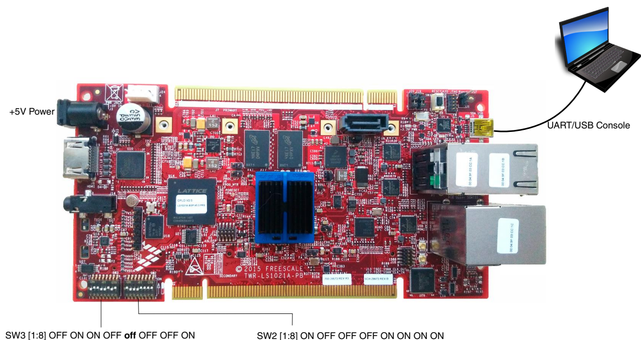
Figure 2. Switch/jumper settings and console port
