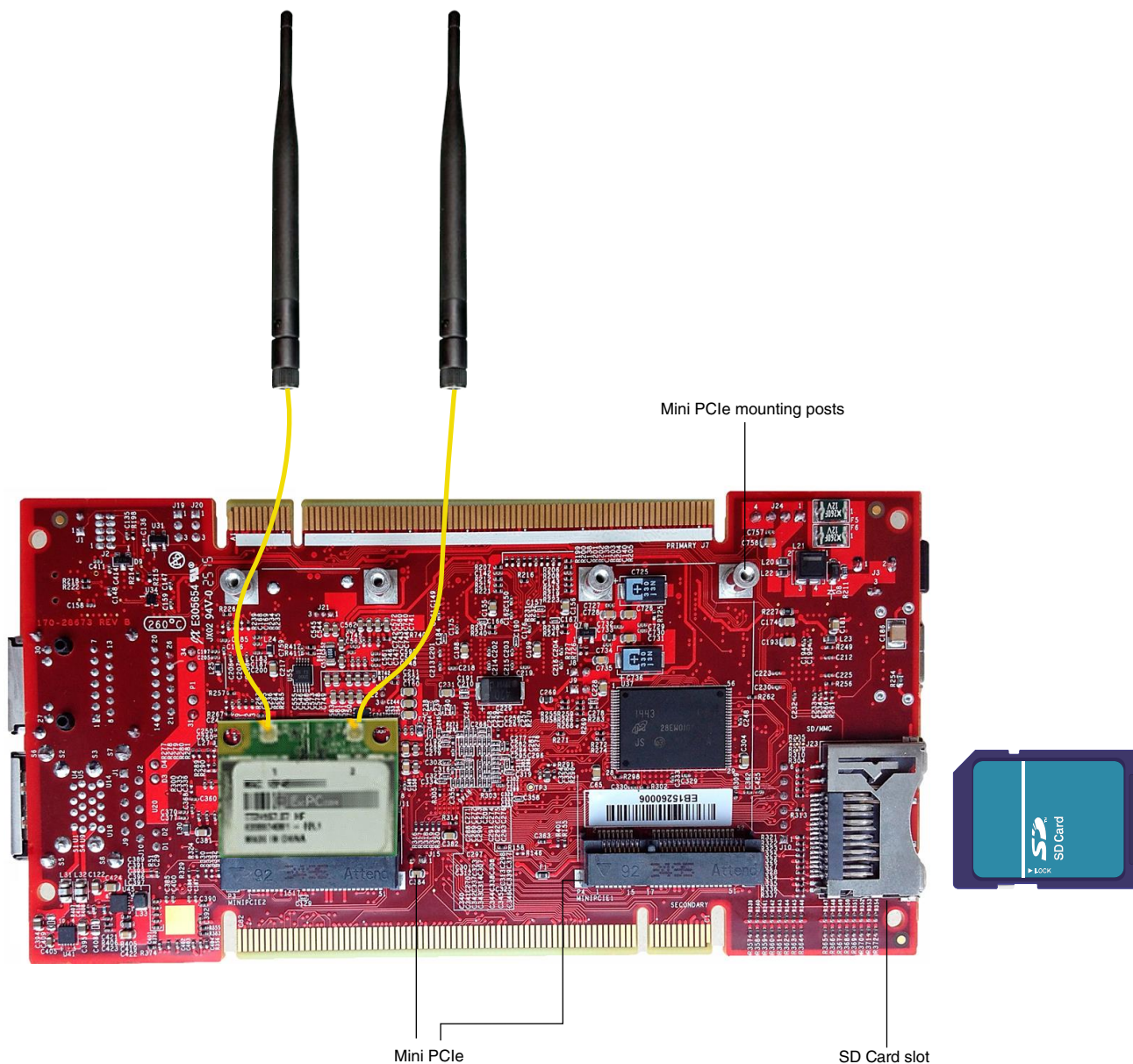
Figure 3. Inserting mPCIe Wi-Fi card and SD card
