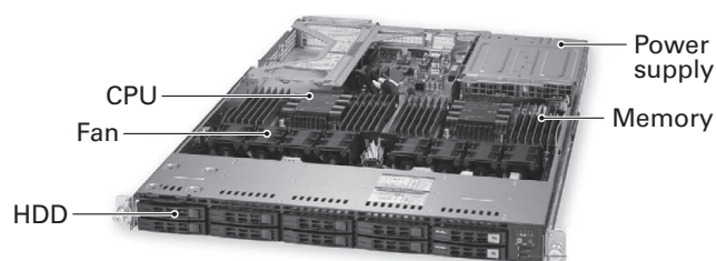
Fig. 2 Example of a 1U server (Photo courtesy of Super Micro Computer, Inc.)
