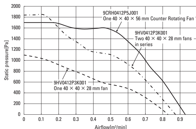
Fig. 8 Example of airflow vs. static pressure characteristics of our typical 40 × 40 mm fans
