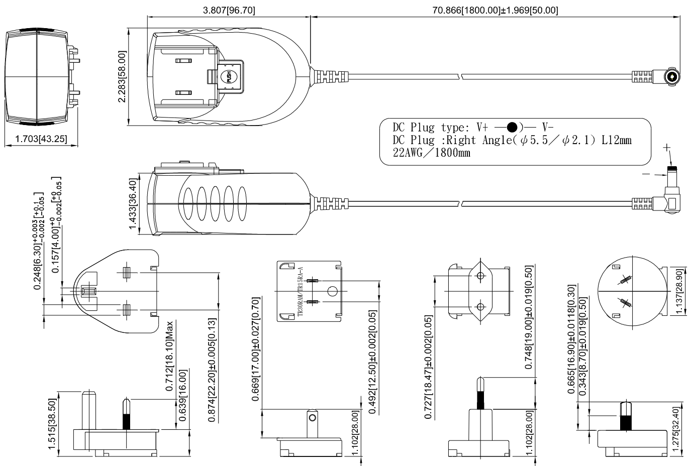
Figure 3. TR30RDM series Mechanical Outline Diagram
