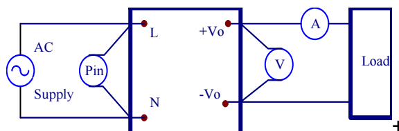
Figure 1. TR30RDM Series Test Setup
