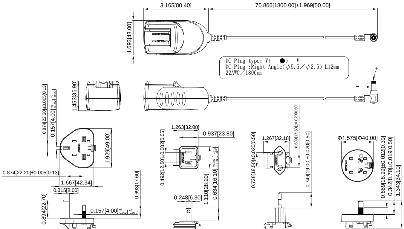
Figure 3. TR18RDM series Mechanical Outline Diagram
