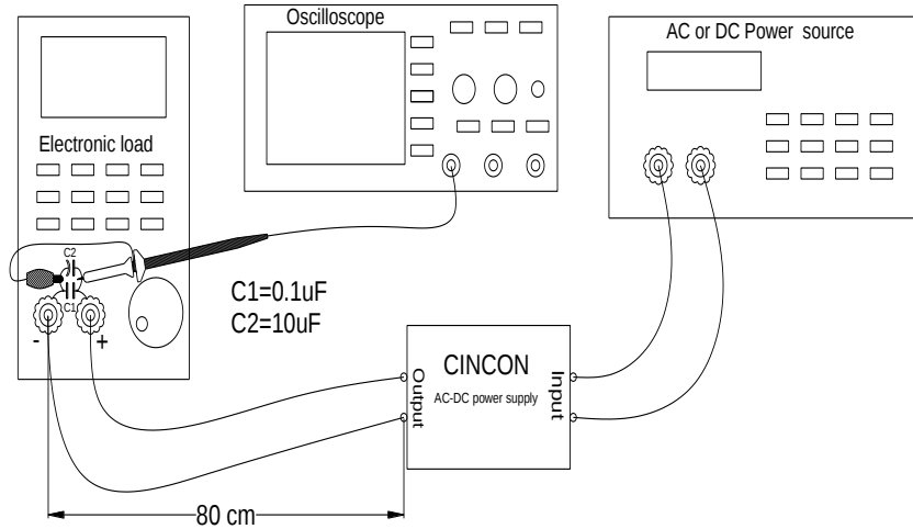
Figure 2. Output Voltage Ripple and Noise Measurement Set-Up
