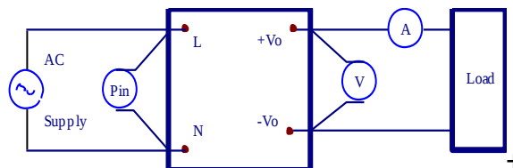
Figure 1. TR18RDM Series Test Setup
