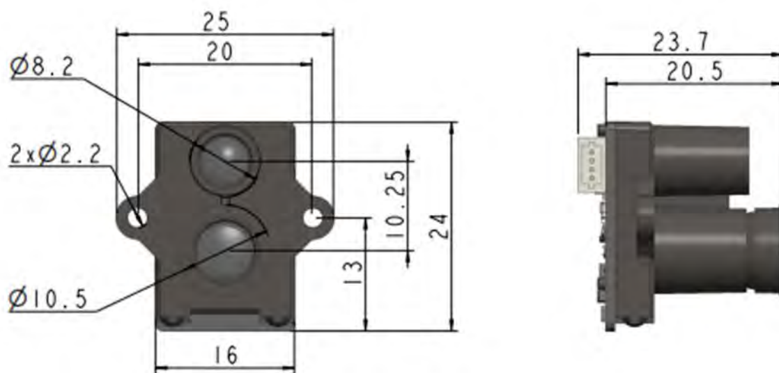
Figure. 4: Diagram of TF-UW500 installation hole
