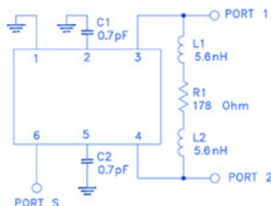
Figure 1. TCP-2-23-75X+ Functional Diagram
