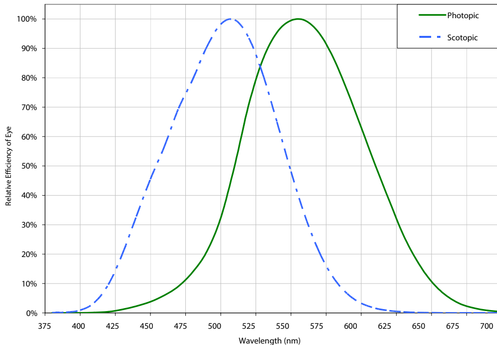
Figure 4. Scotopic and Photopic Vision
