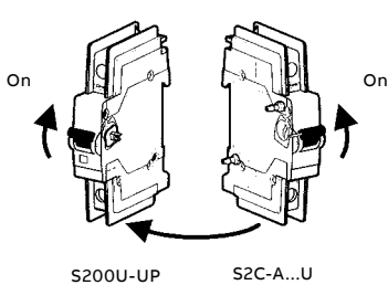
Addition of a S2C-A...U shunt trip
