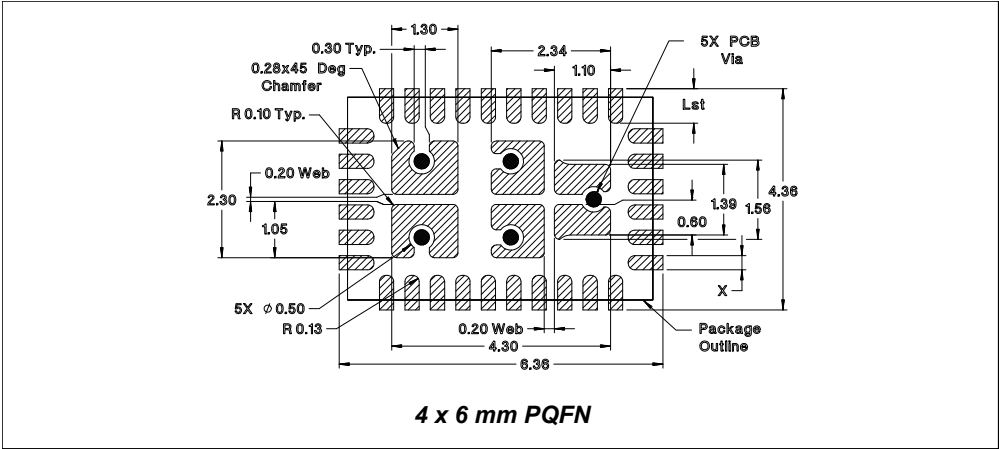
Figure 3-3 Stencil Design
