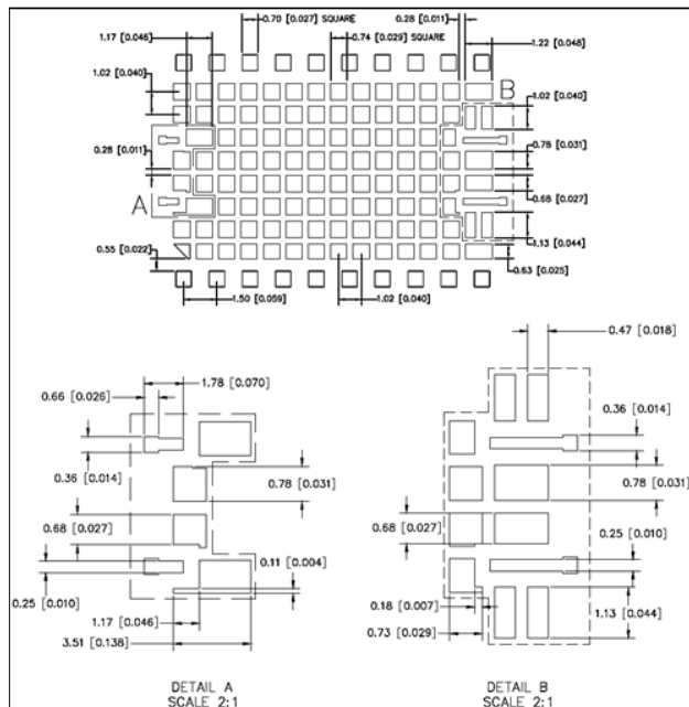
Figure 6: LGA Stencil Designs
