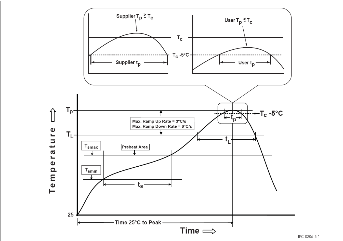
Figure 7. Reflow Profile
