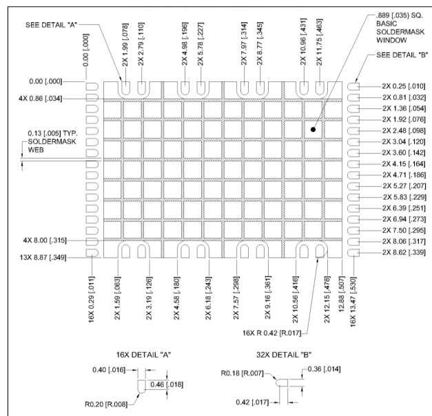
Figure 5: Land and Solder mask Layouts Cont'd
