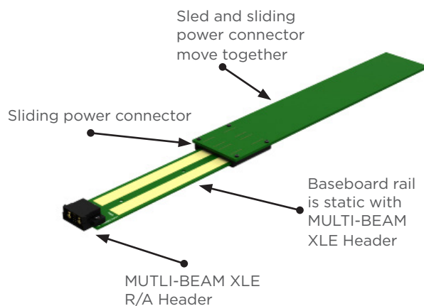
Sliding Power Connector - Top View
