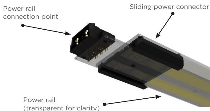
Sliding Power Connector - Bottom View
