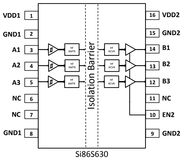
Figure 5.1. Si86S63x Pinout
