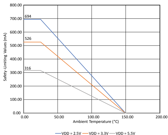
Figure 4.17. (QSOP-16) Thermal Derating Curve, Dependence of Safety Limiting Current
