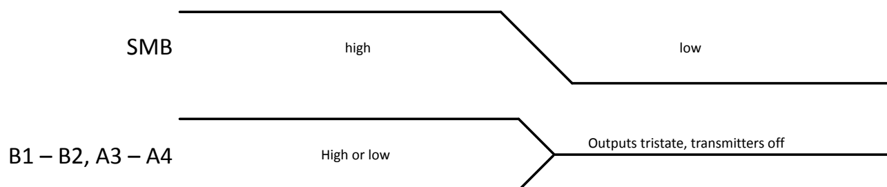
Figure 3.3. Sleep Mode Operation
