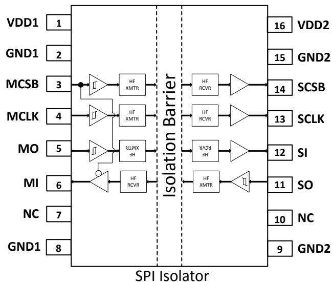
Figure 5.5. Si86SS41 Pinout
