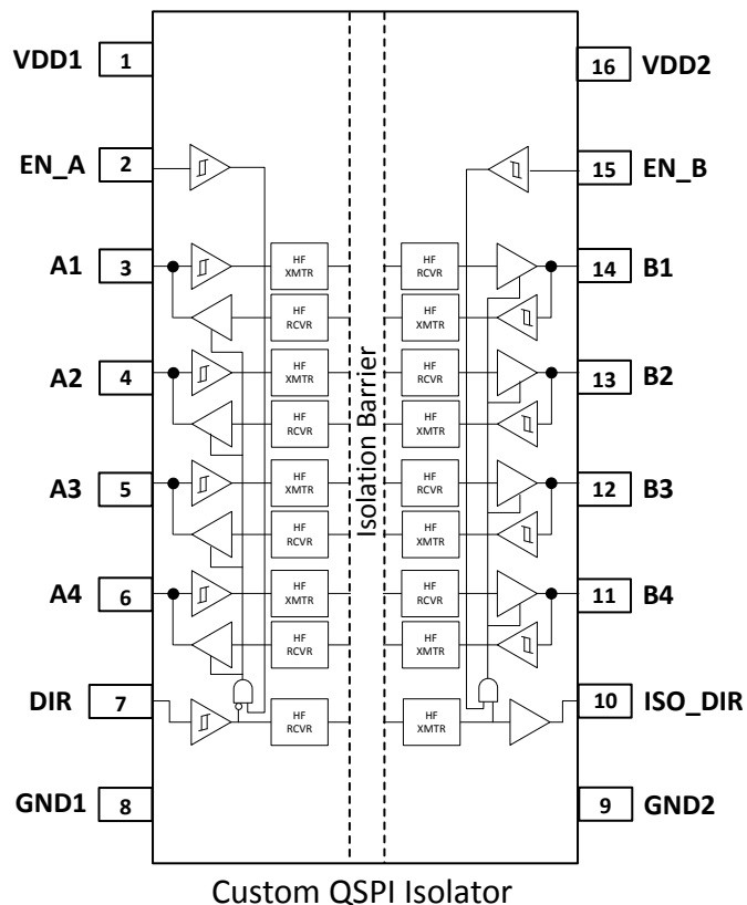
Figure 5.6. Si86SQ44 Pinout
