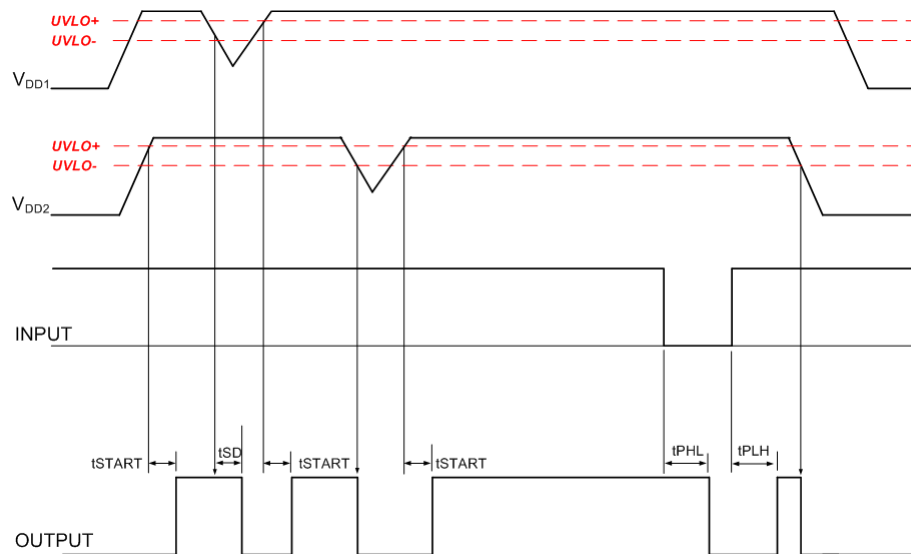
Figure 3.2. Device Behavior during Normal Operation
