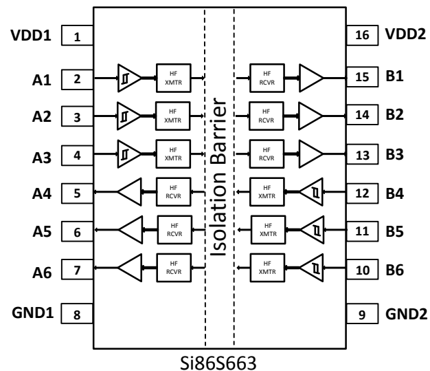
Figure 5.4. Si86S66x Pinout
