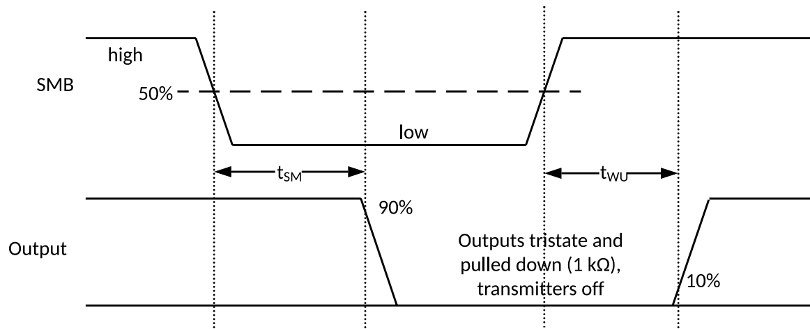
Figure 4.3. SMB Timing
