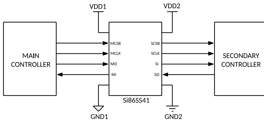
Figure 3.4. Basic SPI
