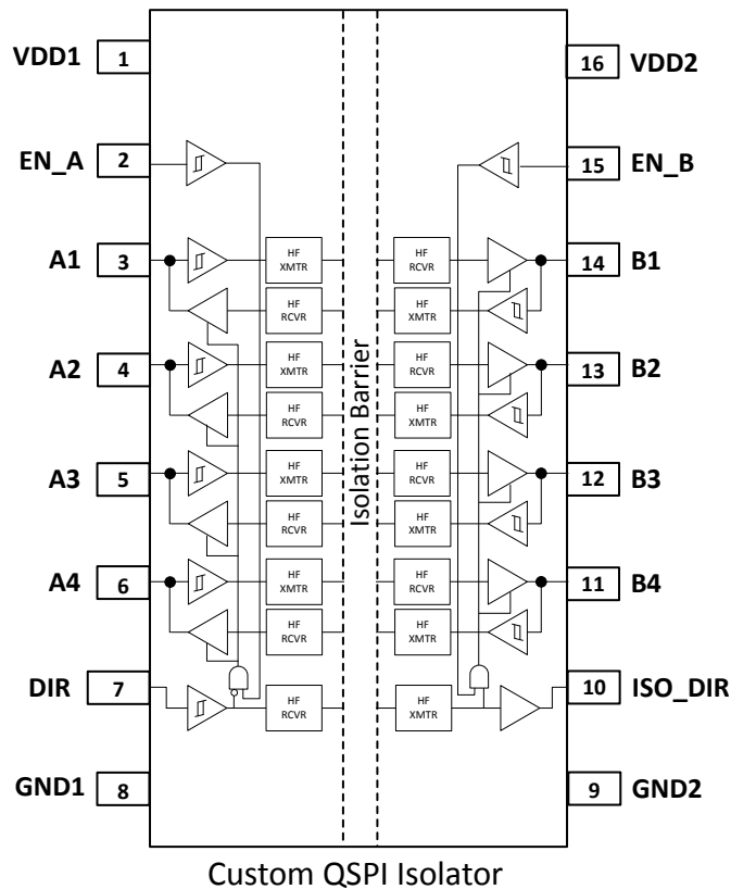
Figure 3.6. Si86SQ44 Configuration
