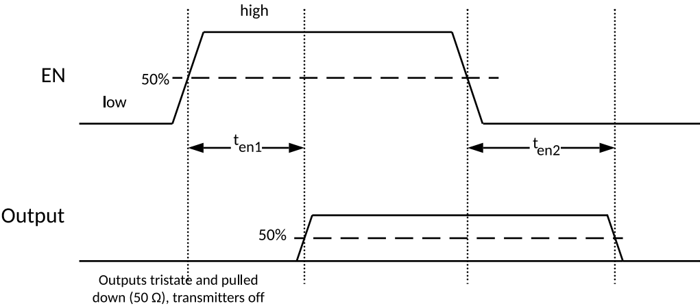
Figure 4.1. ENABLE Timing Diagram
