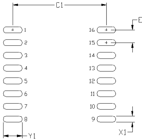
Figure 7.1. WB SOIC-16 PCB Land Pattern
