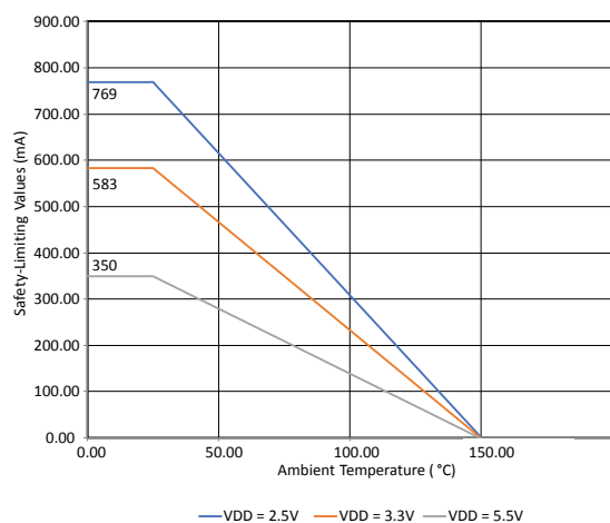
Figure 4.15. (WB SOIC-16) Thermal Derating Curve, Dependence of Safety Limiting Current
