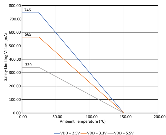
Figure 4.16. (NB SOIC-16) Thermal Derating Curve, Dependence of Safety Limiting Current
