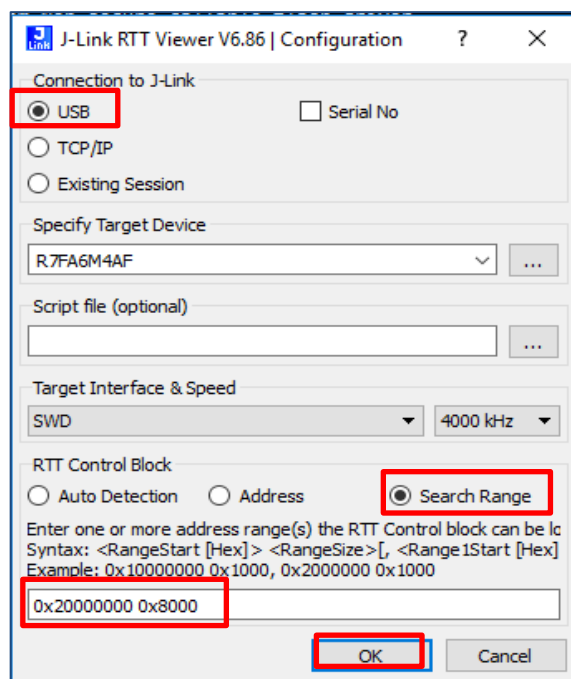
Figure 68. SEGGER RTT Viewer Connection Setup when MCU Running in Standalone Mode
