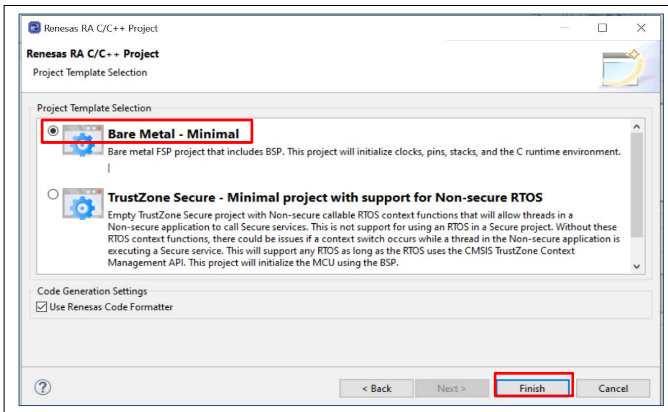
Figure 23. Choose the Project Template
