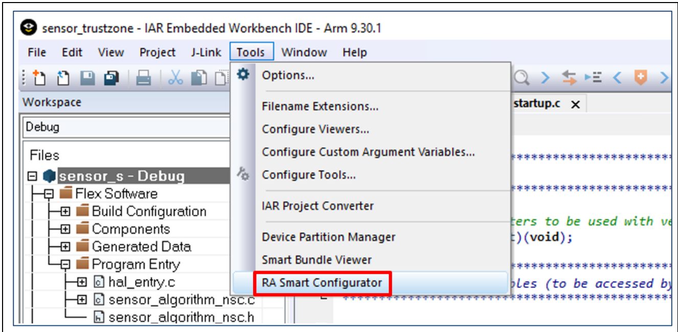
Figure 70. Launch RA Smart Configurator from IAR
