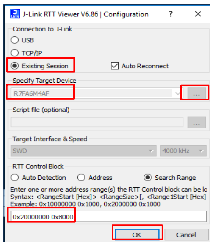
Figure 64. Start the RTT Viewer
