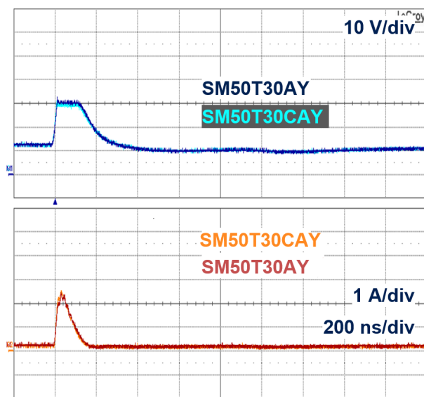
Figure 16. ISO7637-2 pulse 3b response ( V_S = 150\text{ V} ) with 12 V battery
