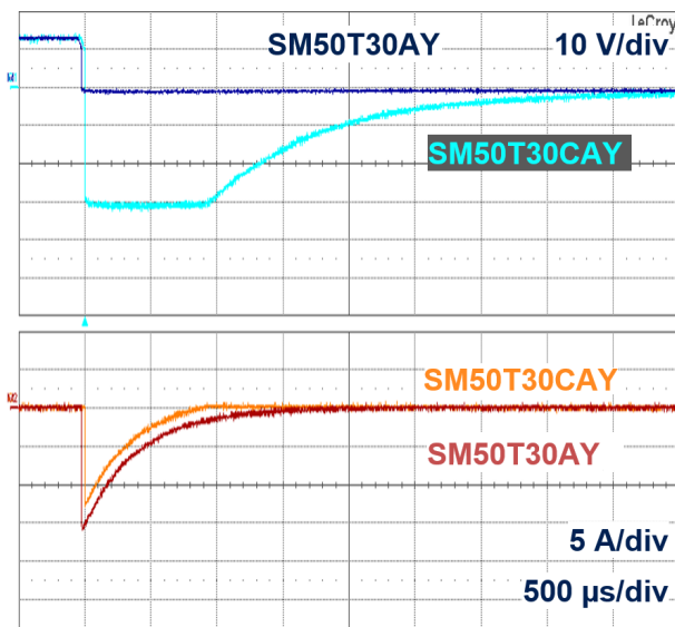
Figure 13. ISO7637-2 pulse 1 response ( V_S = -150 V ) with 12 V battery
