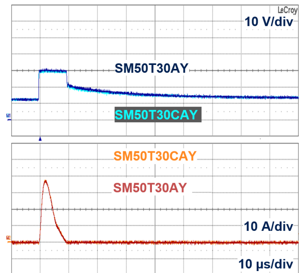
Figure 14. ISO7637-2 pulse 2a response ( V_S = 112 V ) with 12 V battery
