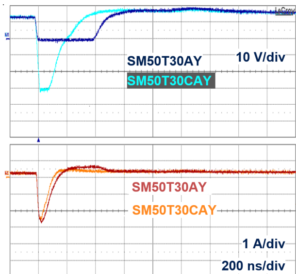
Figure 15. ISO7637-2 pulse 3a response ( V_S = -220\text{ V} ) with 12 V battery
