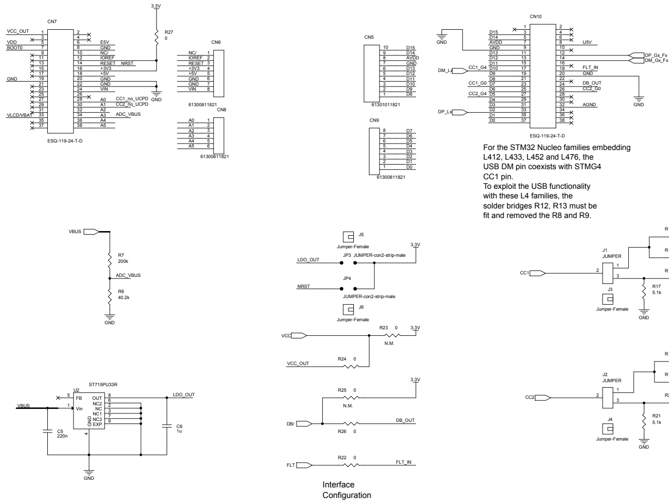
Figure 12. X-NUCLEO-SNK1M1 circuit schematic (1 of 2)
