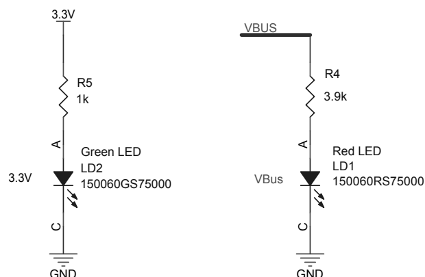
Figure 9. Indication LEDs
