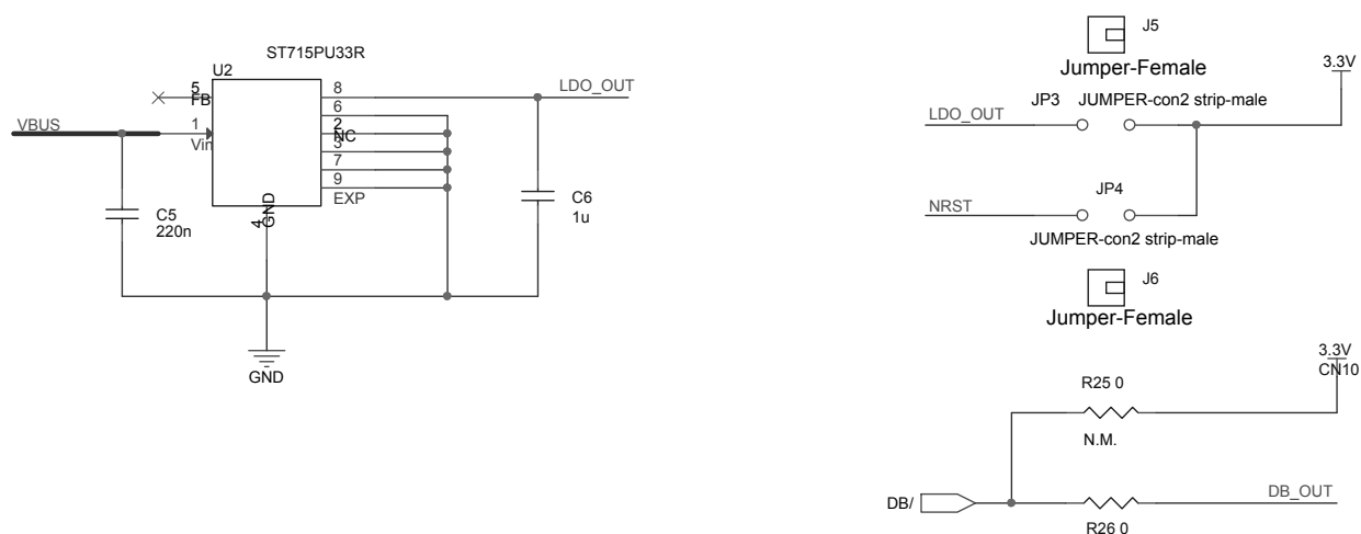
Figure 10. Dead battery mode circuitry
