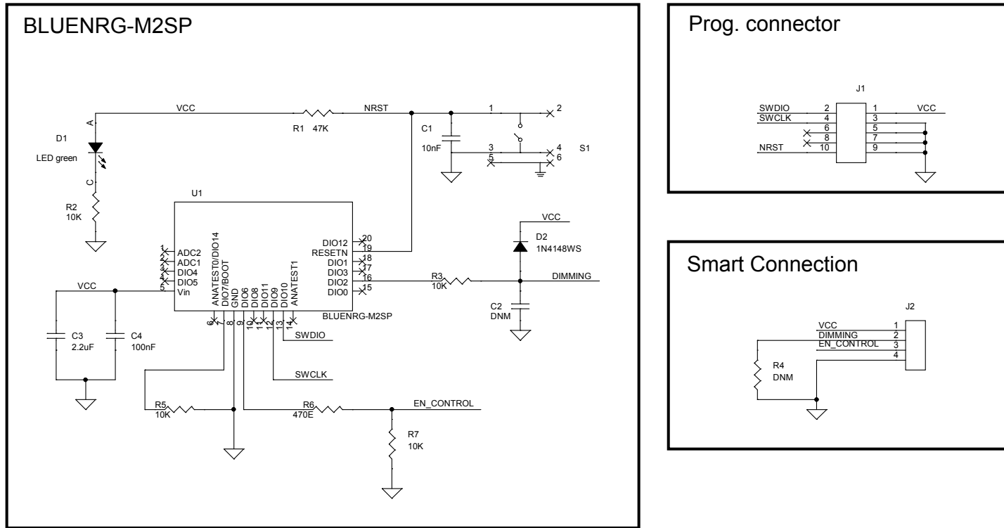
Figure 32. Connectivity board circuit schematic
