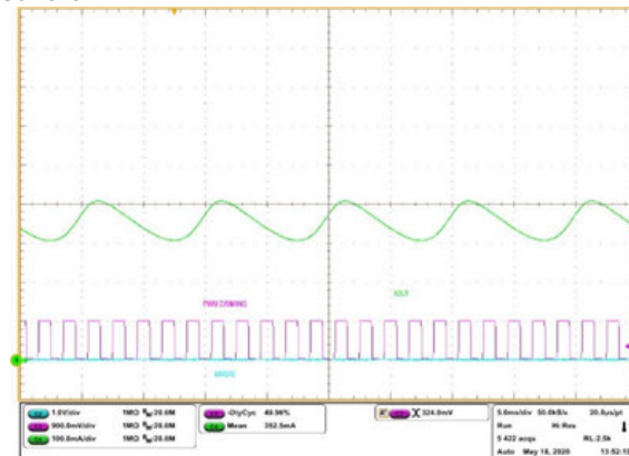
Figure 24. LED 50% dimming at full load
