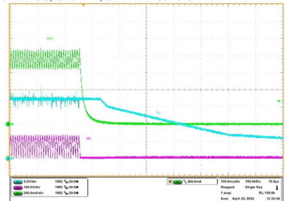
Figure 10. Shutdown plot at 90 V AC input
