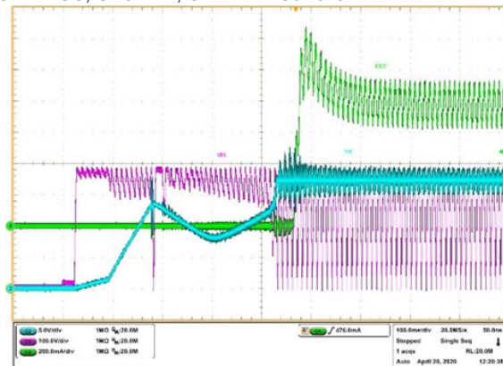
Figure 9. Start-up plot at 265 V AC input
