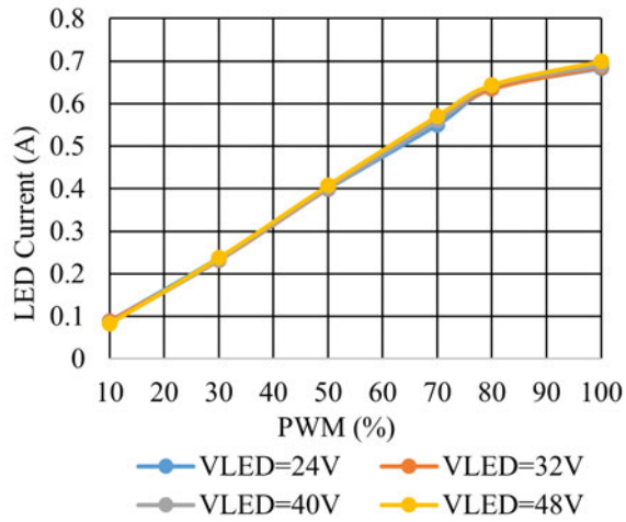
Figure 27. LED current linearity at different LED voltage and dimming value
