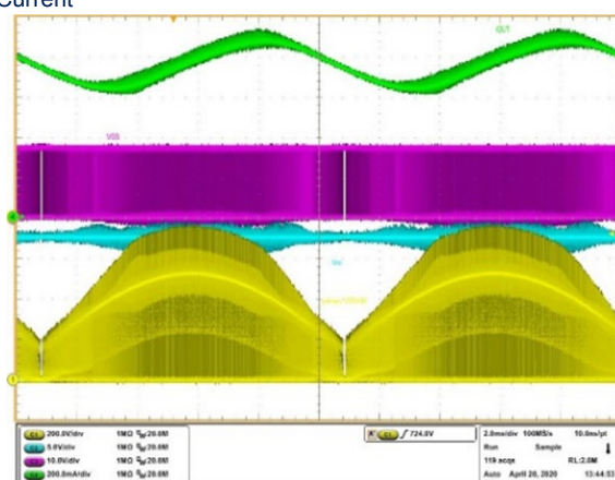
Figure 13. Switching plot at 265 V AC input (channels 1, 2, 3 and 4)
