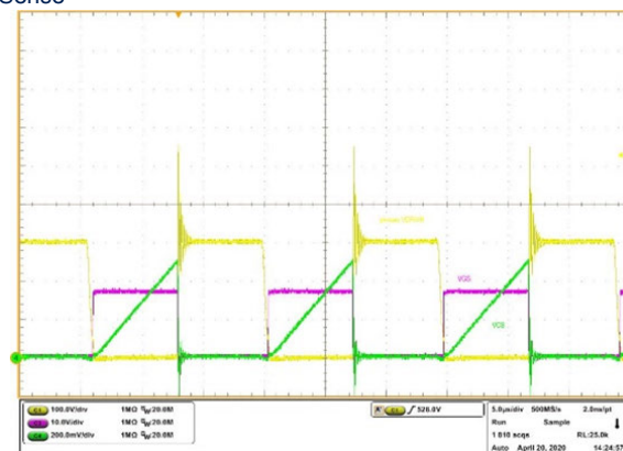
Figure 18. Switching plot at 115 V AC input (channels 1, 2 and 3)
