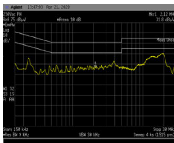
Figure 30. EMI measurement at full load input voltage (230 V AC )
