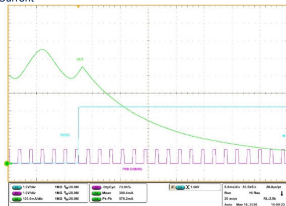
Figure 25. LED ON/OFF condition and 75% dimming at full load
