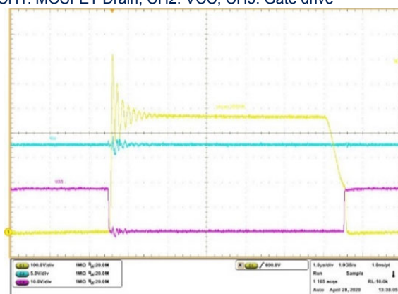
Figure 15. Switching plot at 230 V AC input (channels 1, 2 and 3)
