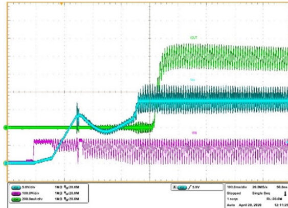
Figure 7. Start-up plot at 90 V AC input
