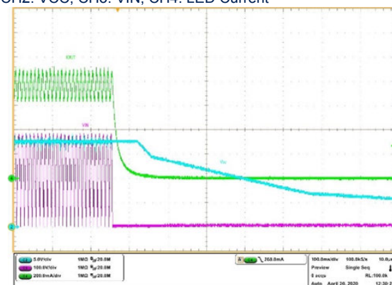
Figure 12. Shutdown plot at 265 V AC input
