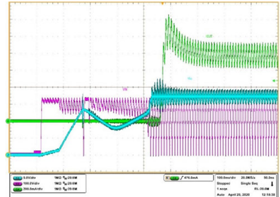
Figure 8. Start-up plot at 230 V AC input
