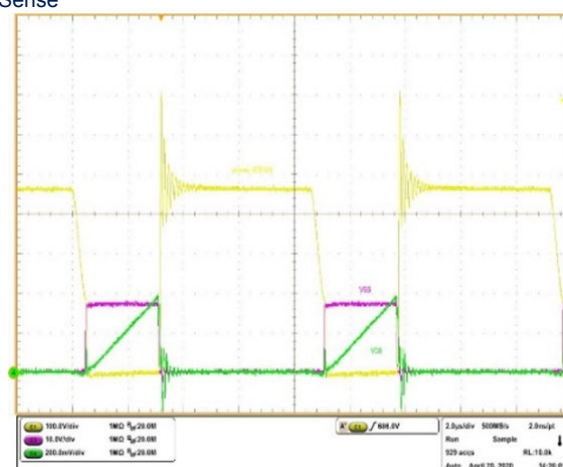
Figure 14. Switching plot at 230 V AC input (channels 1, 3 and 4)
