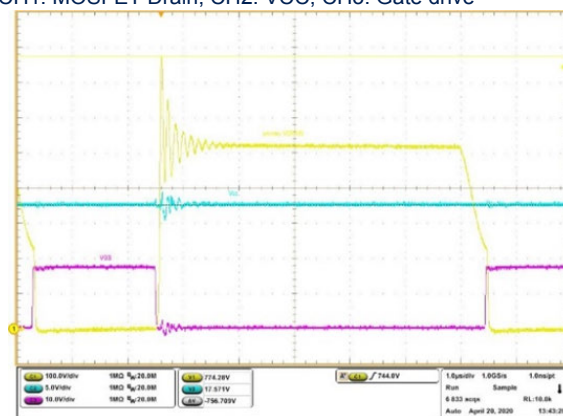
Figure 16. Switching plot at 265 V AC input (channels 1, 2 and 3)
