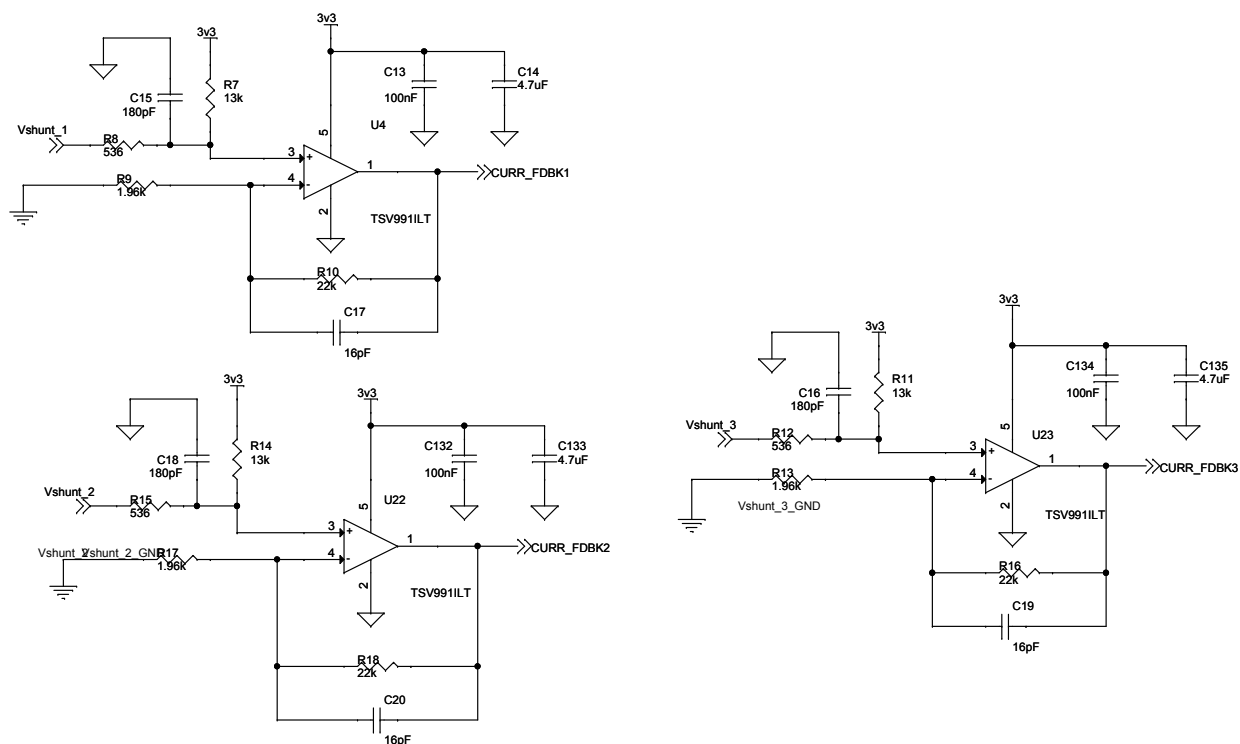
Motion Control - Current Sensing External op-amp
