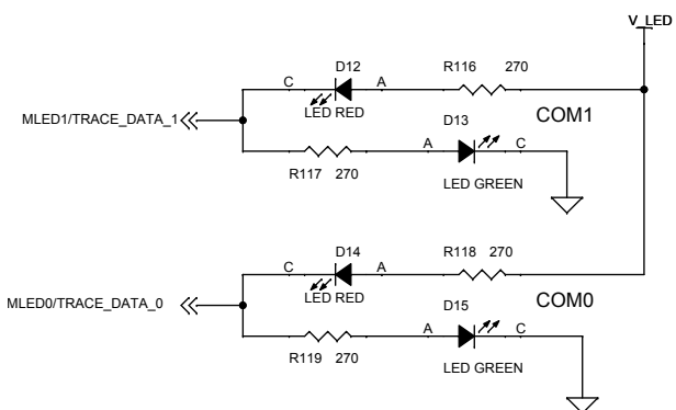
Figure 14. Communication status LEDs
