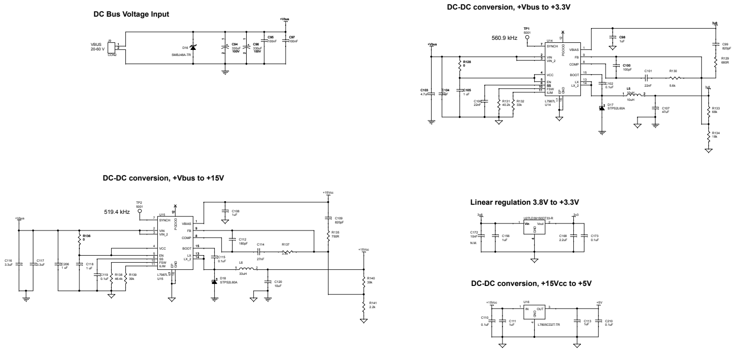
Figure 24. STEVAL-ETH001V1 circuit schematic (1 of 10)
