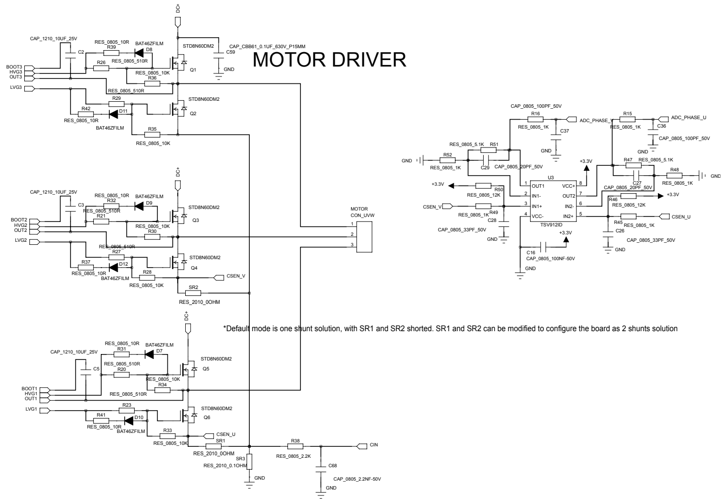
Figure 12. STEVAL-CTM012V1 circuit schematic (1 of 2)
