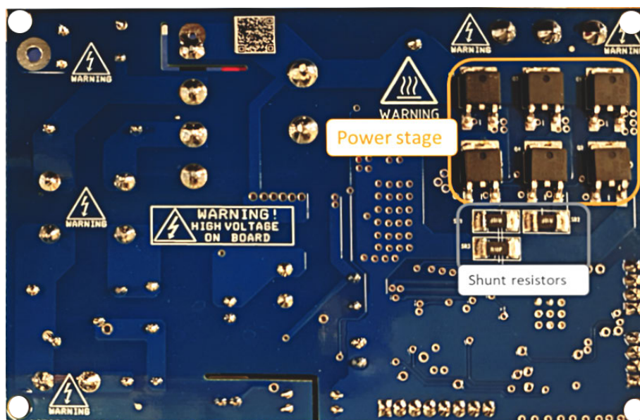
Figure 3. STEVAL-CTM012V1 main components (bottom view)
