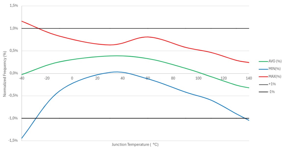
Figure 18. HSI frequency versus temperature
