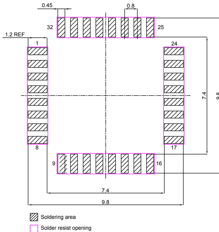
Figure 37. LQFP32 - Footprint example
