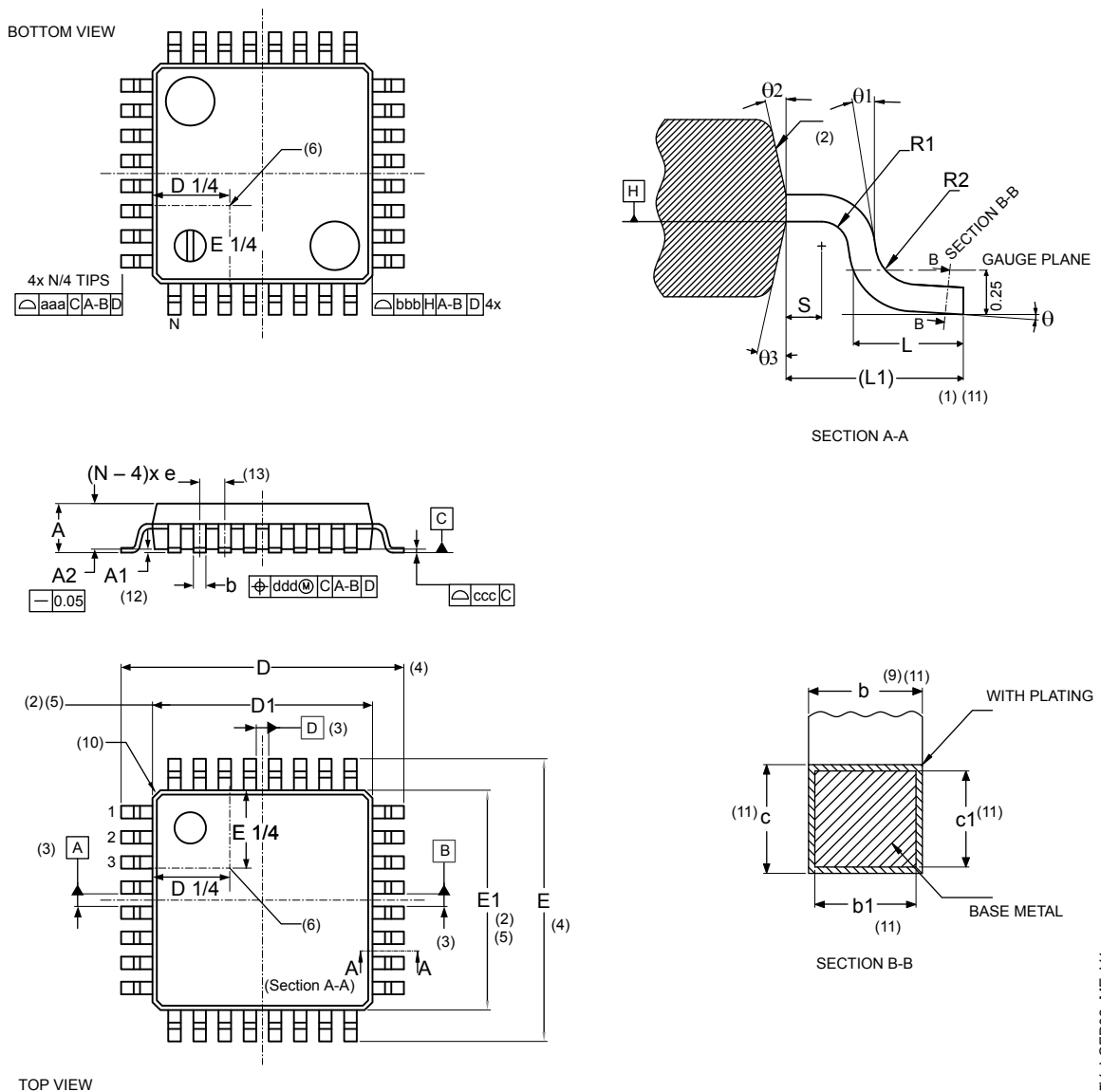
Figure 36. LQFP32- Outline
