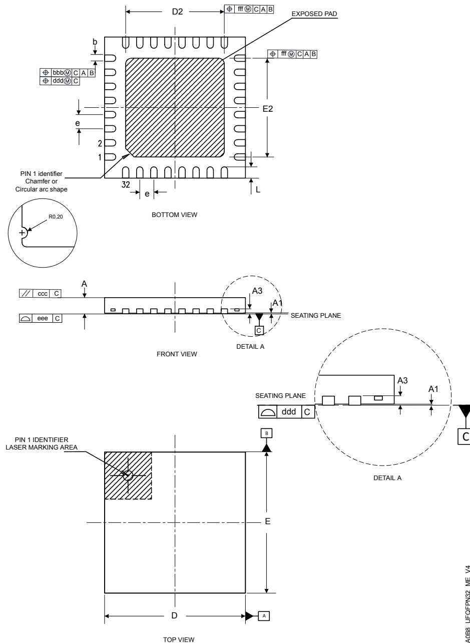
Figure 45. UFQFPN32 - Outline
