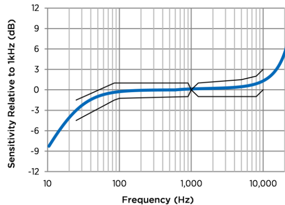
Figure 3: Typical Free Field Magnitude Response and Masks
