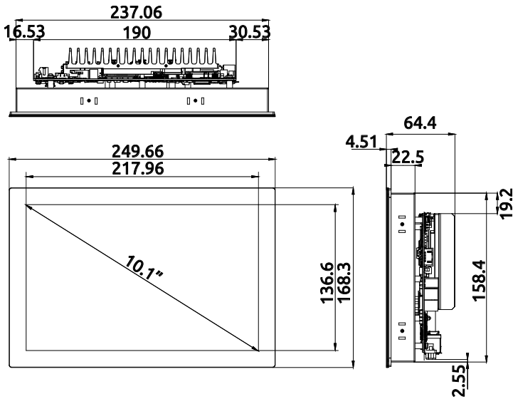
Figure 2-2: SP2-10WP-TGL Dimensions
