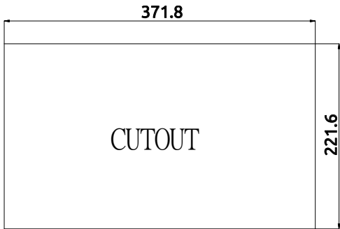
Figure 2-9: SP2-15WP-TGL Cutout Dimensions
