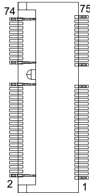
Figure 3-14: M.2 2230 Connector Pin Definition
