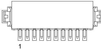
Figure 3-32: GPIO Connector Pin Definition
