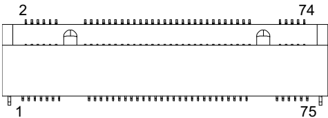
Figure 3-35: M.2 2280 Connector Pin Definition
