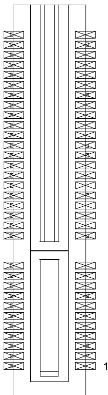
Figure 3-26: PCIe Gen4 x4 Connector Pin Definition
