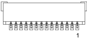
Figure 3-28: LED Connector Pin Definition
