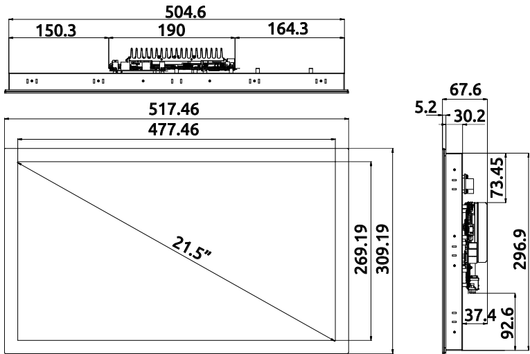
Figure 2-4: SP2-21WP-TGL Dimensions
