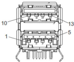
Figure 3-3: USB 3.2 Connector Pin Definition
