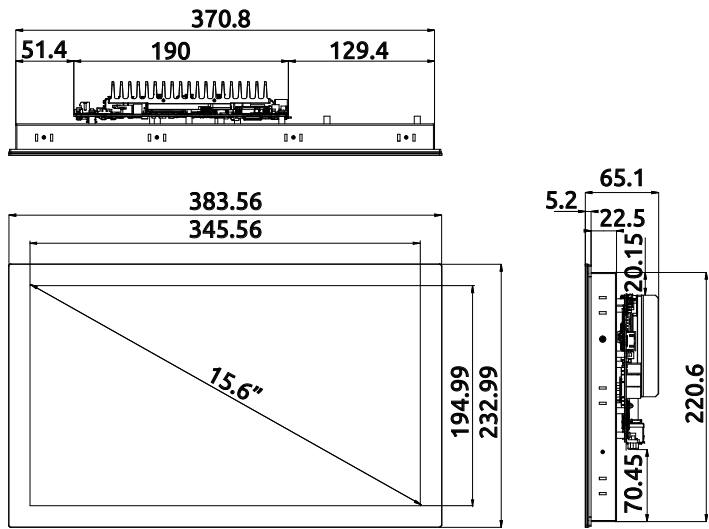
Figure 2-3: SP2-15WP-TGL Dimensions
