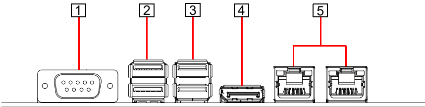
Figure 3-1: SP2-TGL Series External I/O
