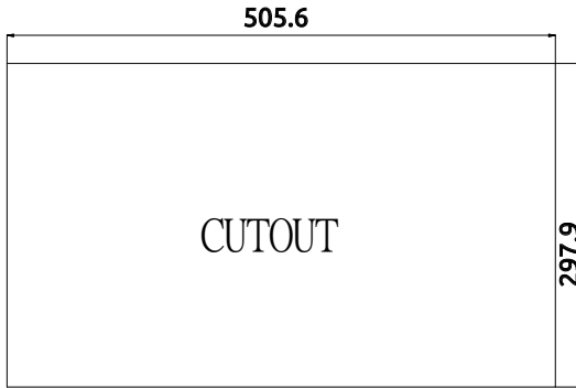
Figure 2-10: SP2-21WP-TGL Cutout Dimensions
