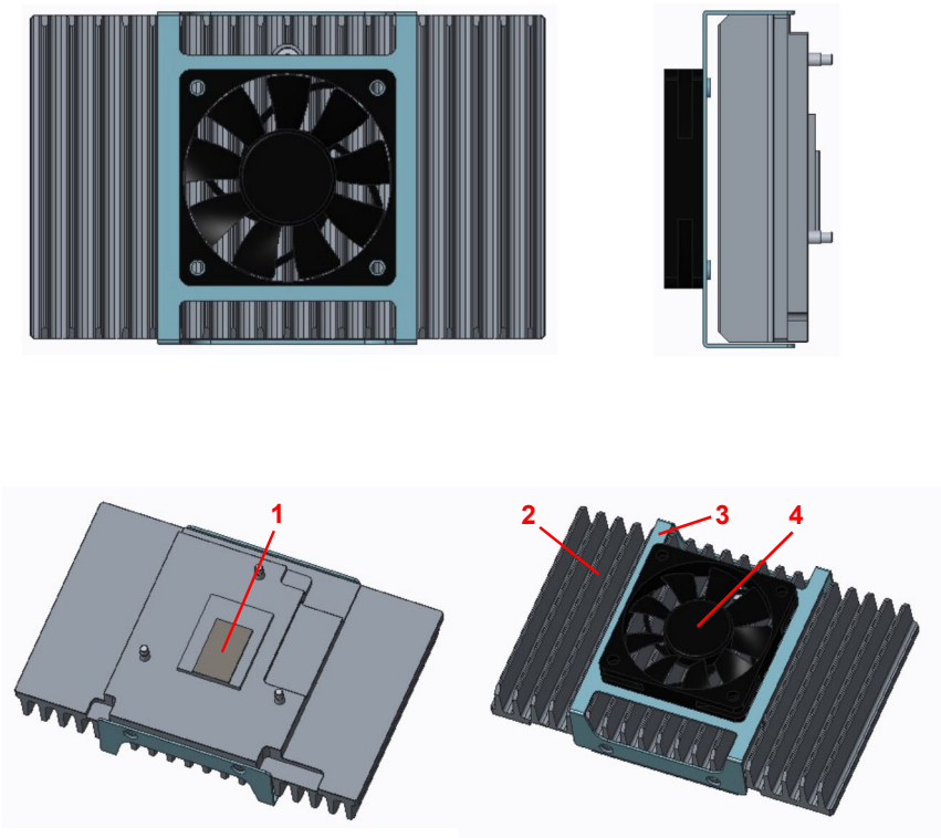
Figure 2-5: Active Cooling Heat Sink
