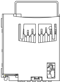
Figure 3-33: Nano SIM Connector Pin Definition
