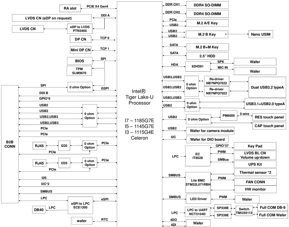
Figure 2-1: SP2-TGL Series Block Diagram
