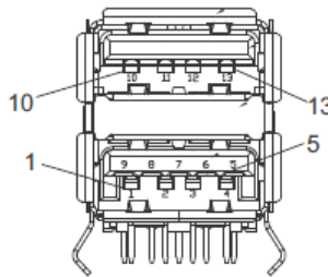
Figure 3-4: USB 3.0 + USB 2 .0 Connector Pin Definition
