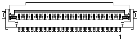
Figure 3-31: DB40 Connector Pin Definition
