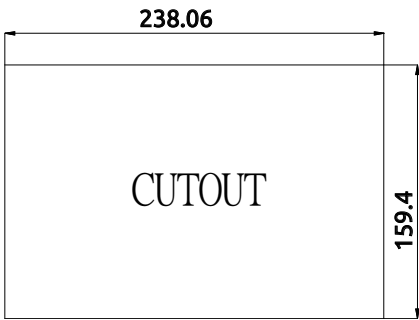
Figure 2-8: SP2-10WP-TGL Cutout Dimensions
