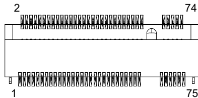
Figure 3-13: M.2 3042 Connector Pin Definition
