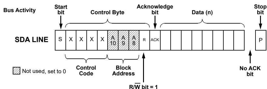
Figure 85: Current Address Read Command, \overline{R/W} = 1
