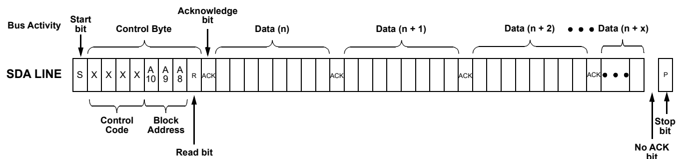
Figure 87: Sequential Read Command
