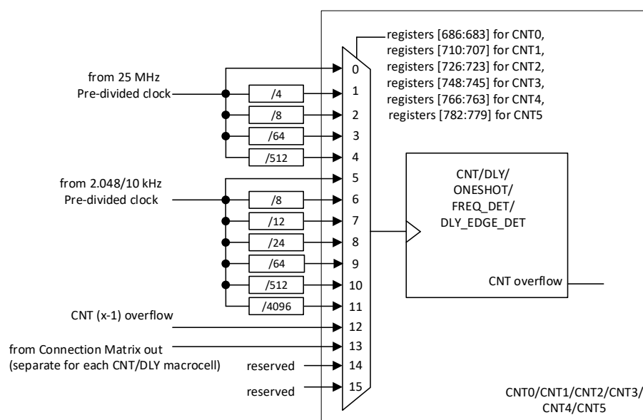
Figure 66: Clock Scheme
