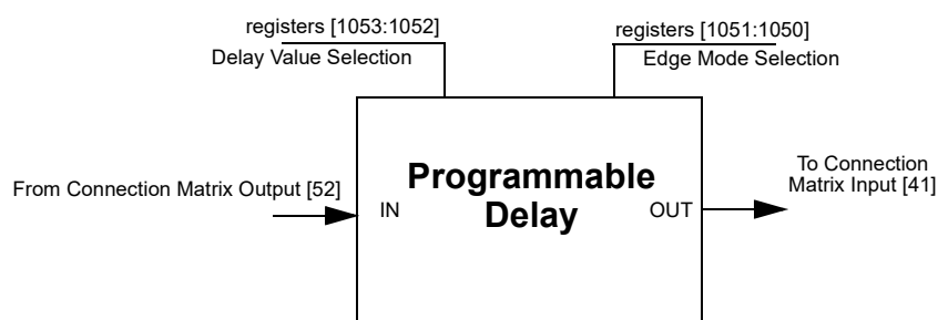
Figure 61: Programmable Delay
