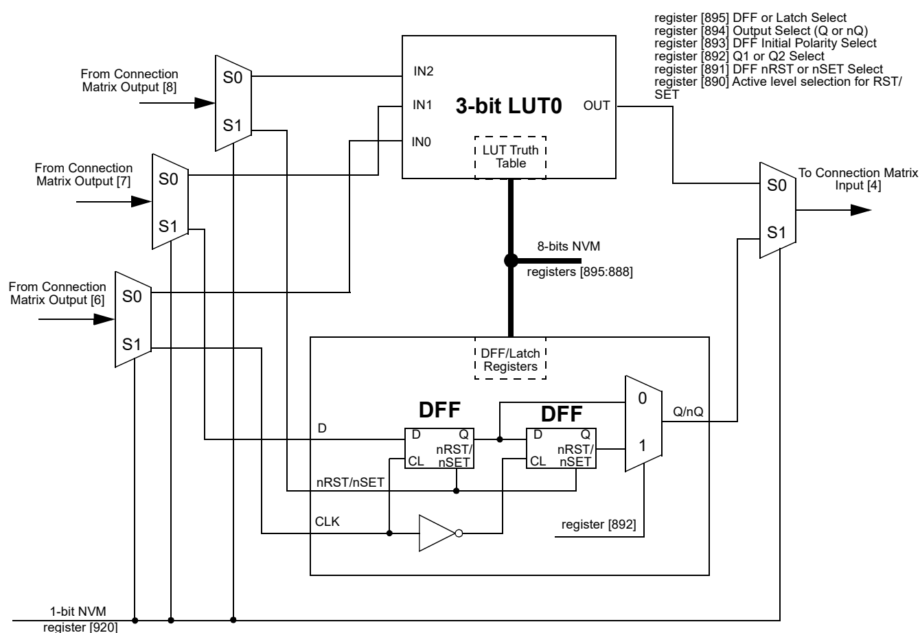
Figure 29: 3-bit LUT0 or DFF2
