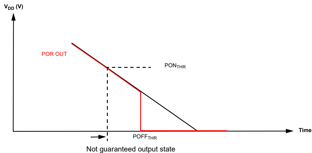
Figure 80: Power-Down
