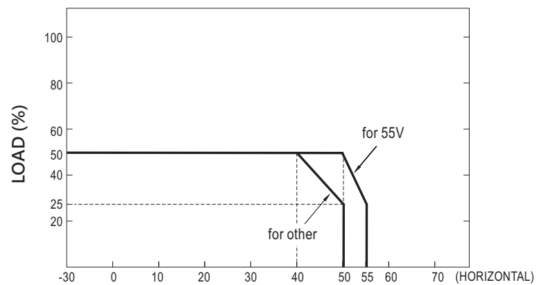
AMBIENT TEMPERATURE WITH 85CFM FAN*2
