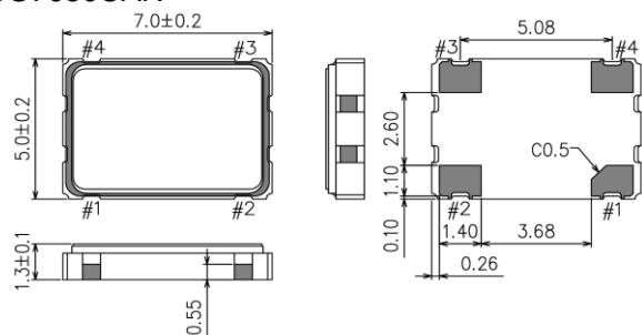
SG7050CAN
