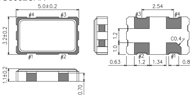
SG5032CAN
