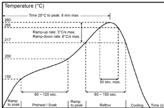
Solder Reflow Temperature Condition
