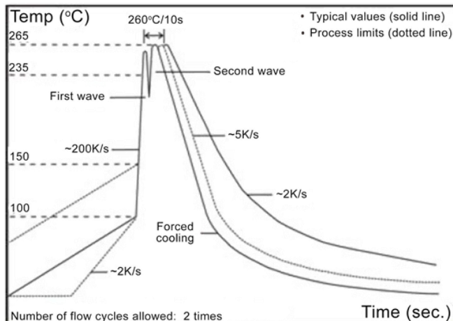
Wave Solder Temperature Condition
