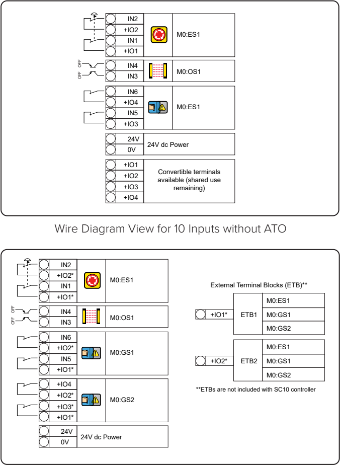
Wire Diagram View for 14 Inputs with ATO
