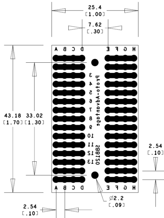
(Representative drawing only - not to scale)
