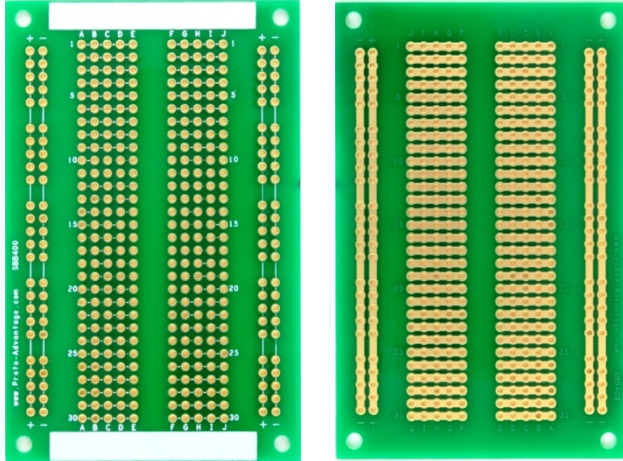
1/2 size breadboard match (P/N: SBB400)
