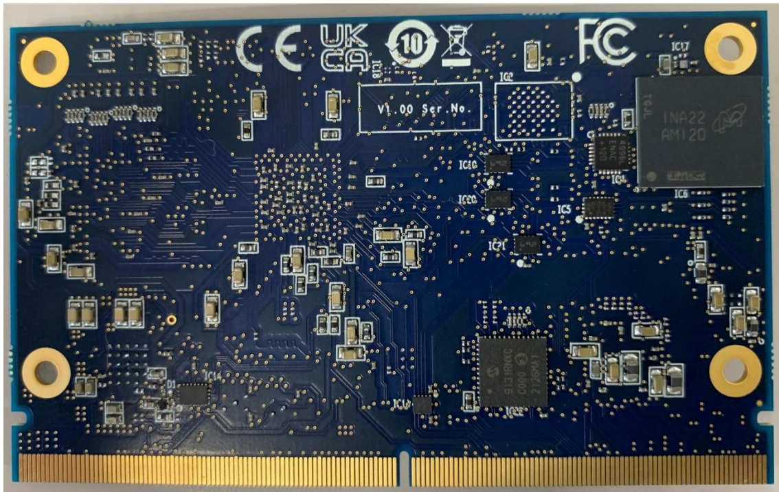
Figure 1.3 Bottom View of the RTK9743U11C01000BE
