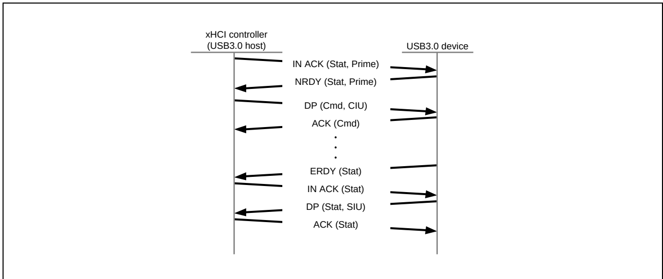
Figure 35.6-34 Example SuperSpeed UASP Non-Data Transfer
