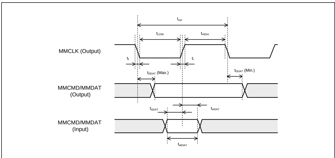
Figure 54.5-10 eMMC Timing
