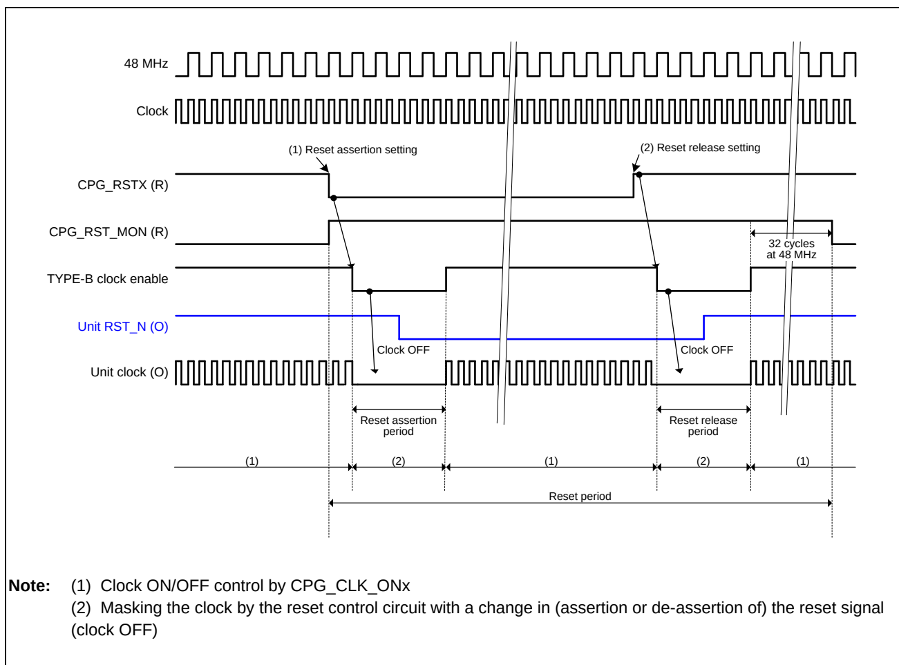
Figure 48.6-27 TYPE-B Reset Timing by the CPG Register
