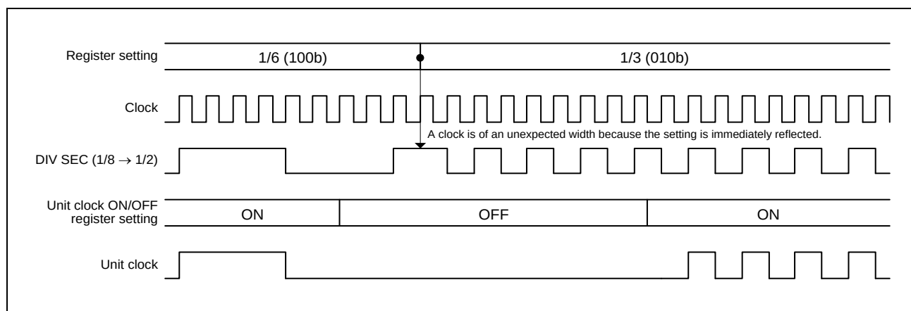
Figure 48.6-12 Timing Chart of Clock Switching of the Static Switching Variable Divider
