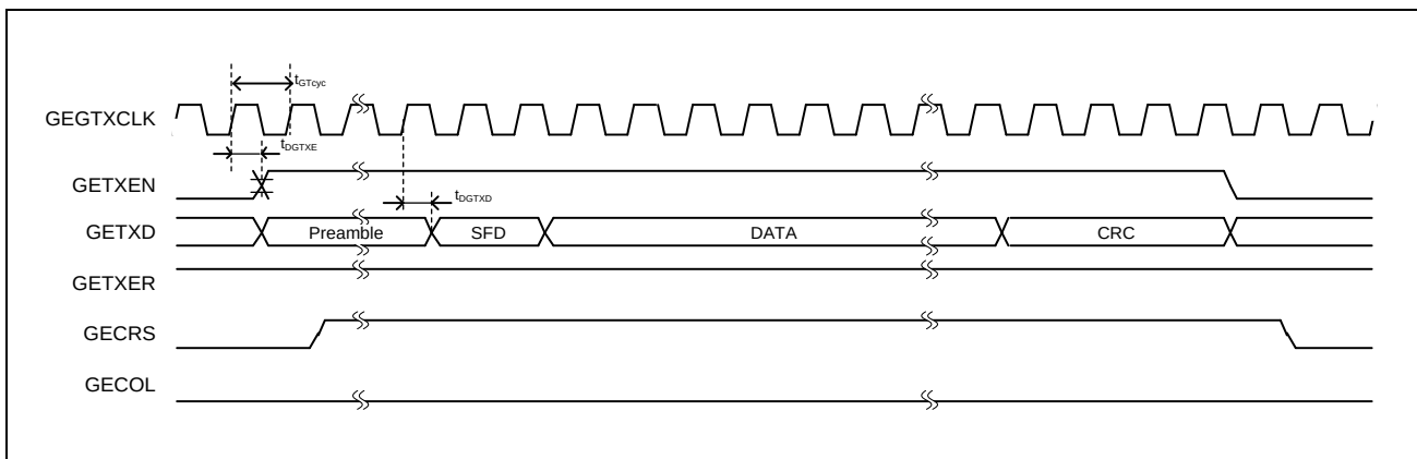
Figure 54.5-7 Transmission Timing
