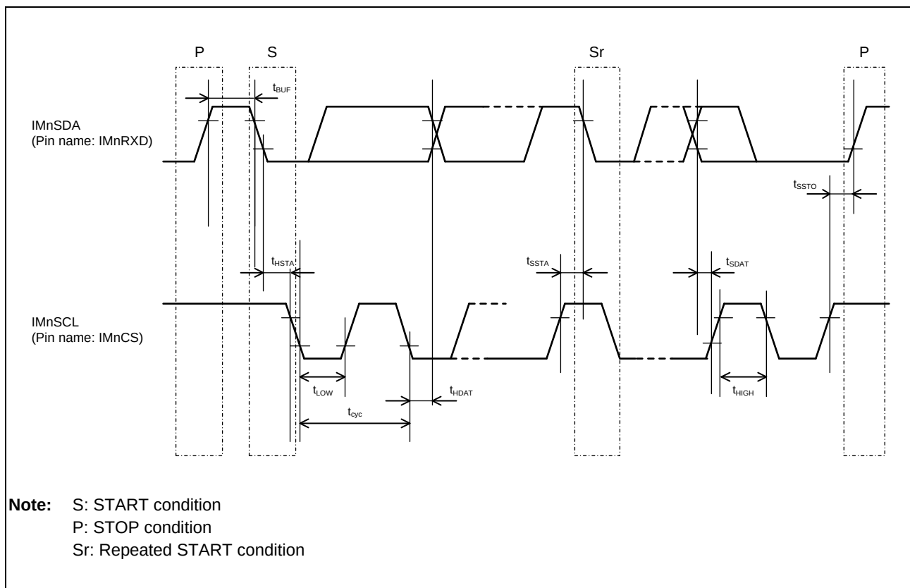
Figure 54.5-13 IIC Timing
