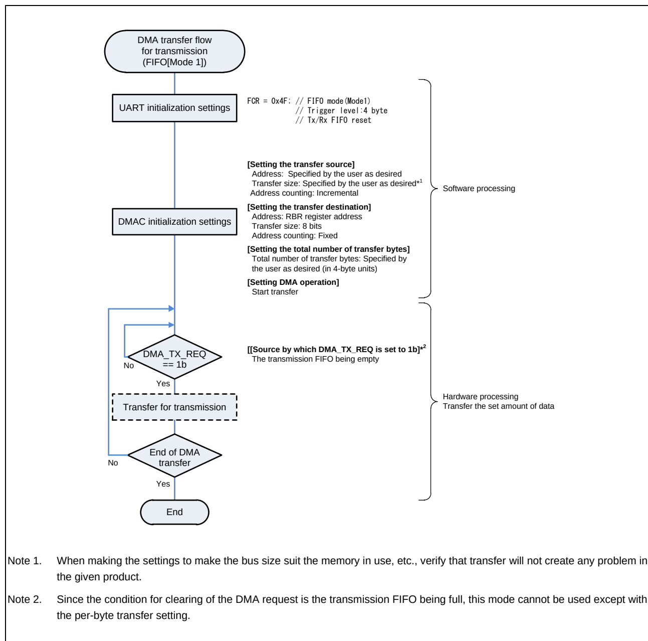
Figure 40.5-7 DMA Transfer Flow for Transmission (in (6) Mode 1)
