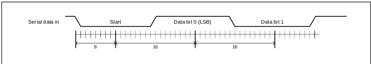
Figure 40.4-3 Serial Data Sampling Timing
