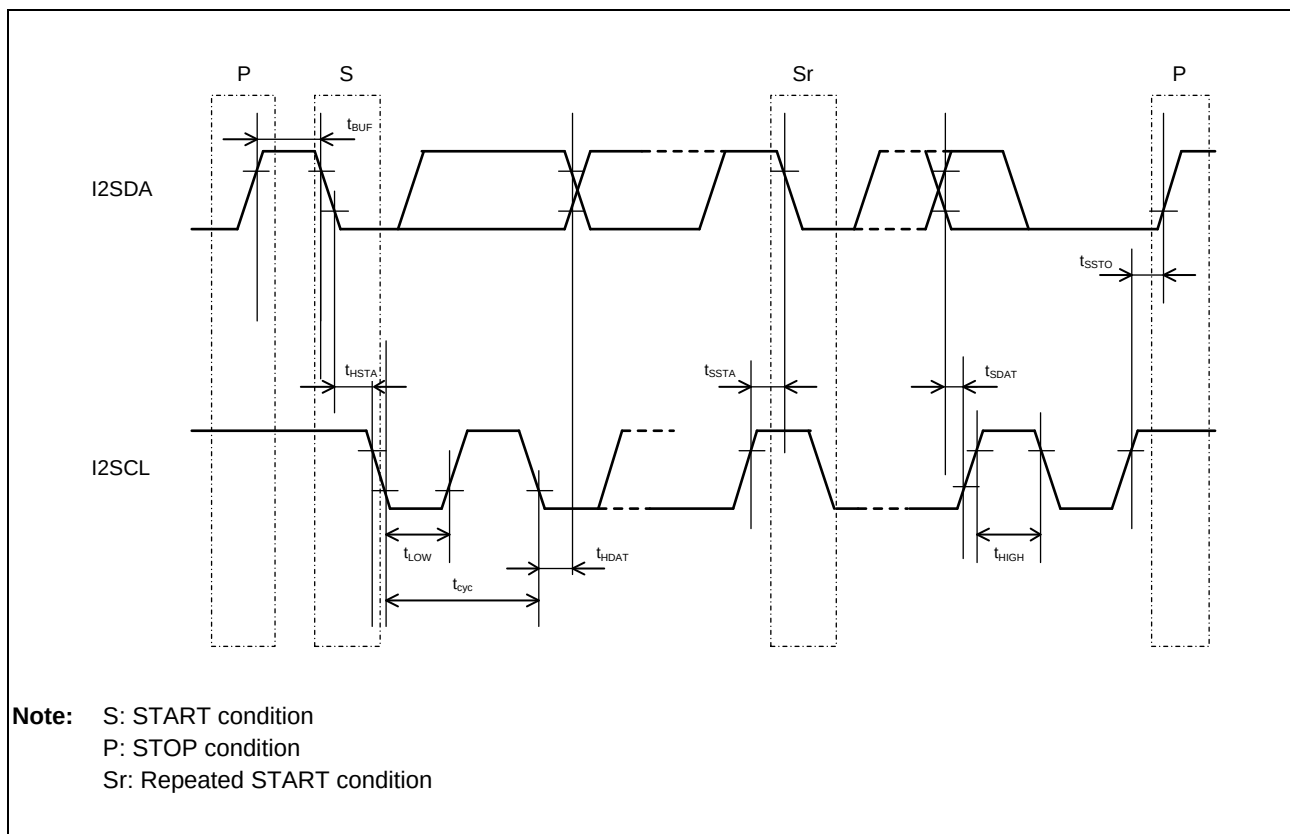
Figure 54.5-1 IIC Timing
