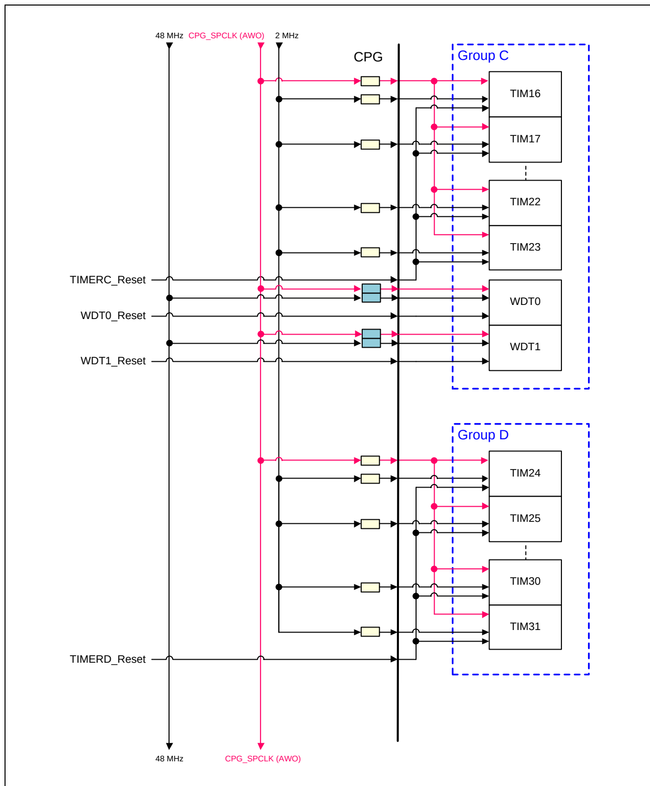
Figure 48.6-18 Block Diagram of Groups C and D
