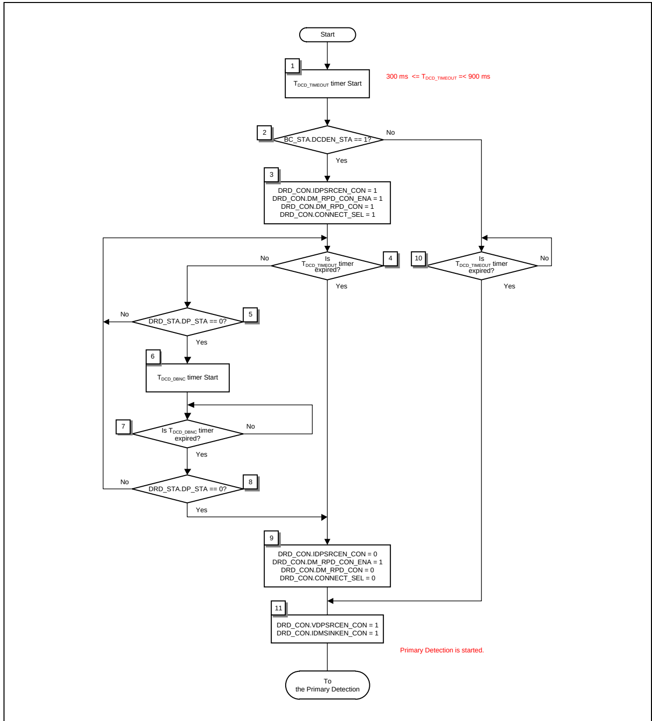
Figure 35.4-7 Good Battery Algorithm Flowchart (DCD Flow)
