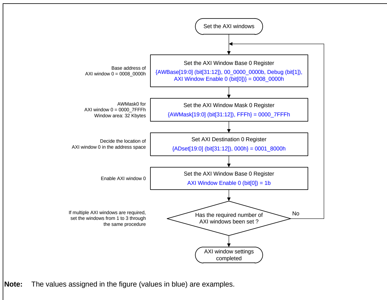
Figure 36.8-2 Example Settings of the AXI Windows
