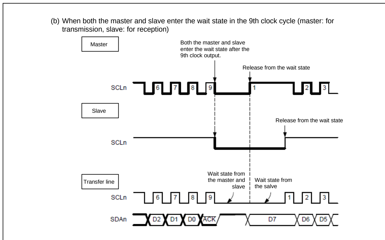
Figure 38.6-7 Wait (2/2)
