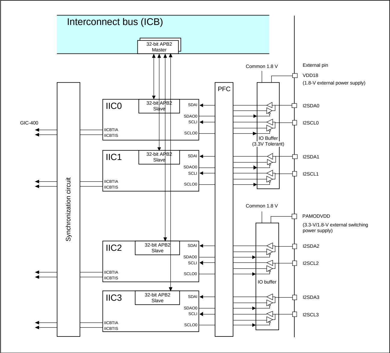
Figure 38.1-1 Connection Configuration
