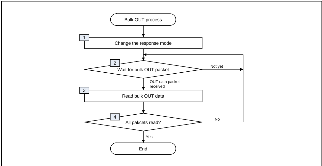
Figure 35.6-31 Bulk OUT Process Flow
