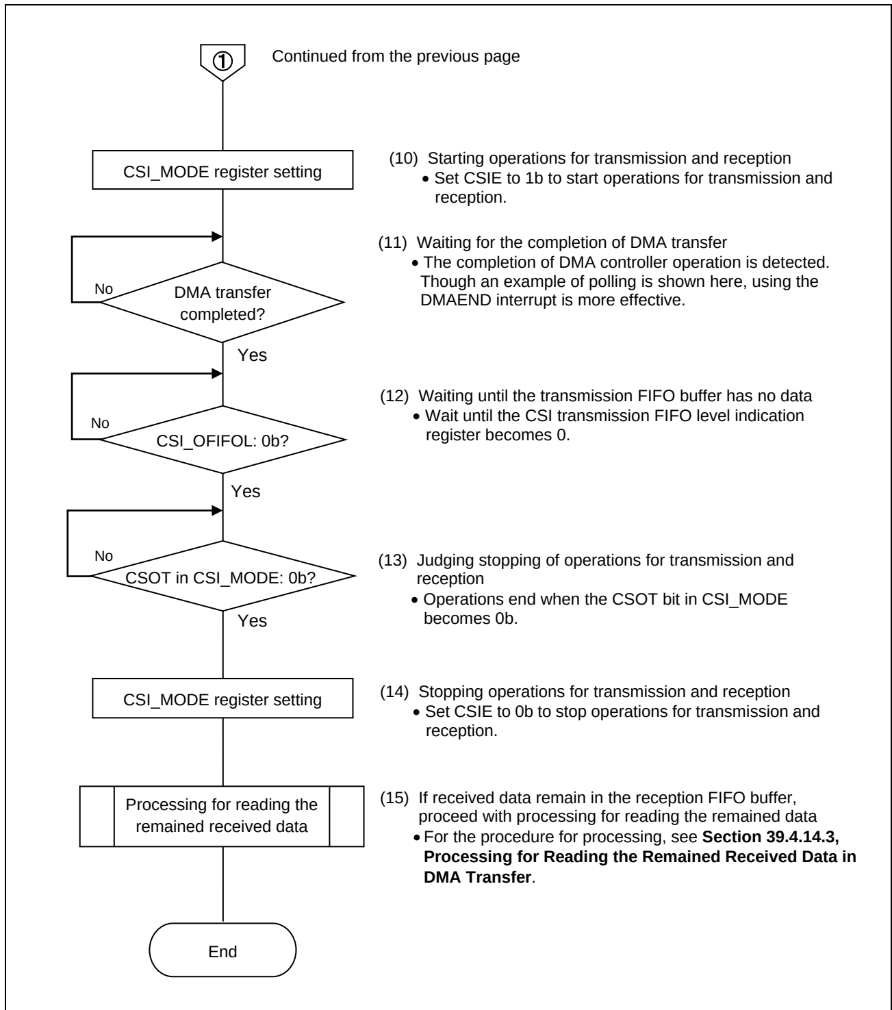
Figure 39.4-23 Flow of Operations of DMA Transfer in Master Transmission/Reception Mode (Continuous Data Transmission) (2/3)
