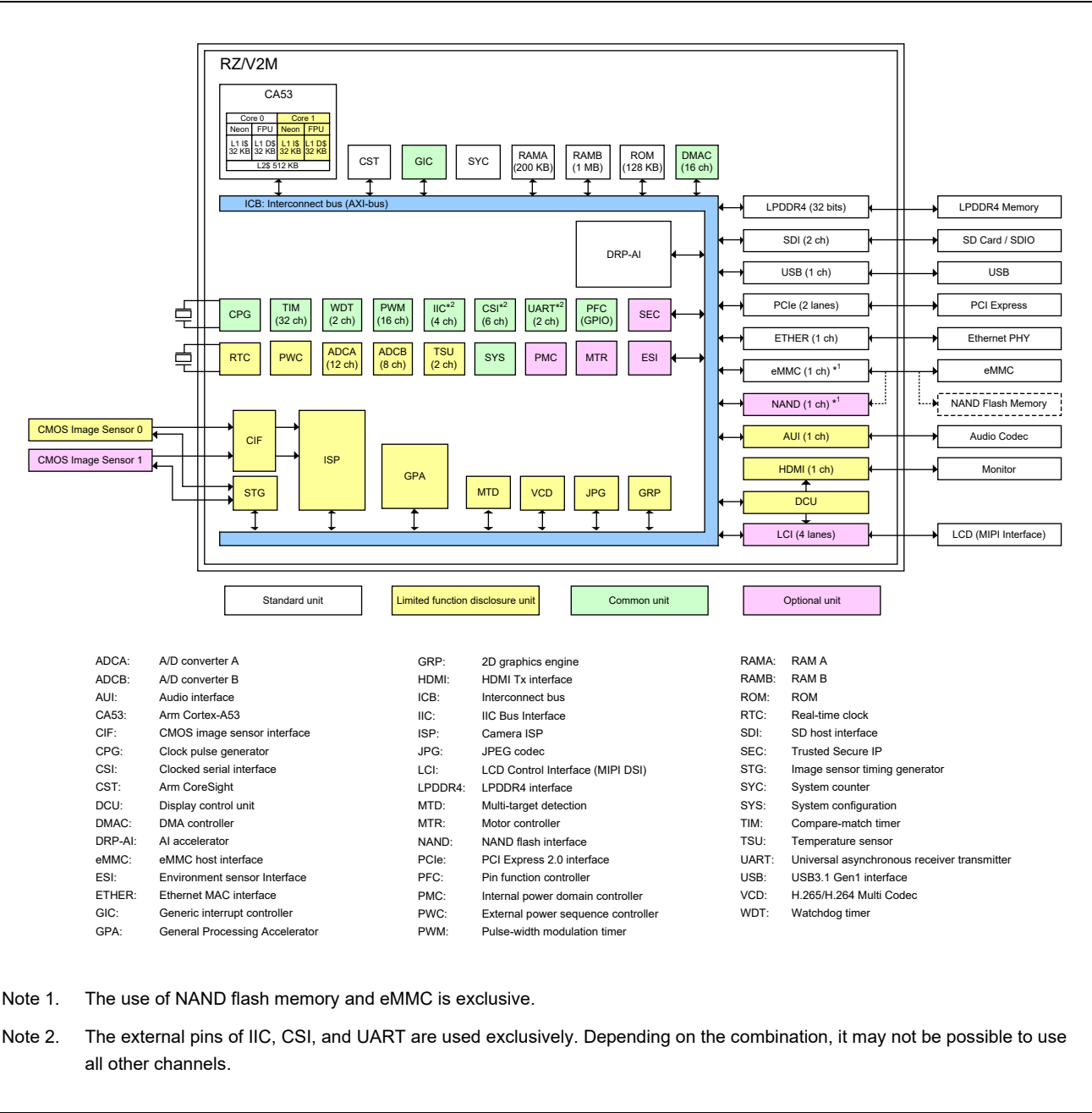
Figure 1.4-1 Block Diagram
