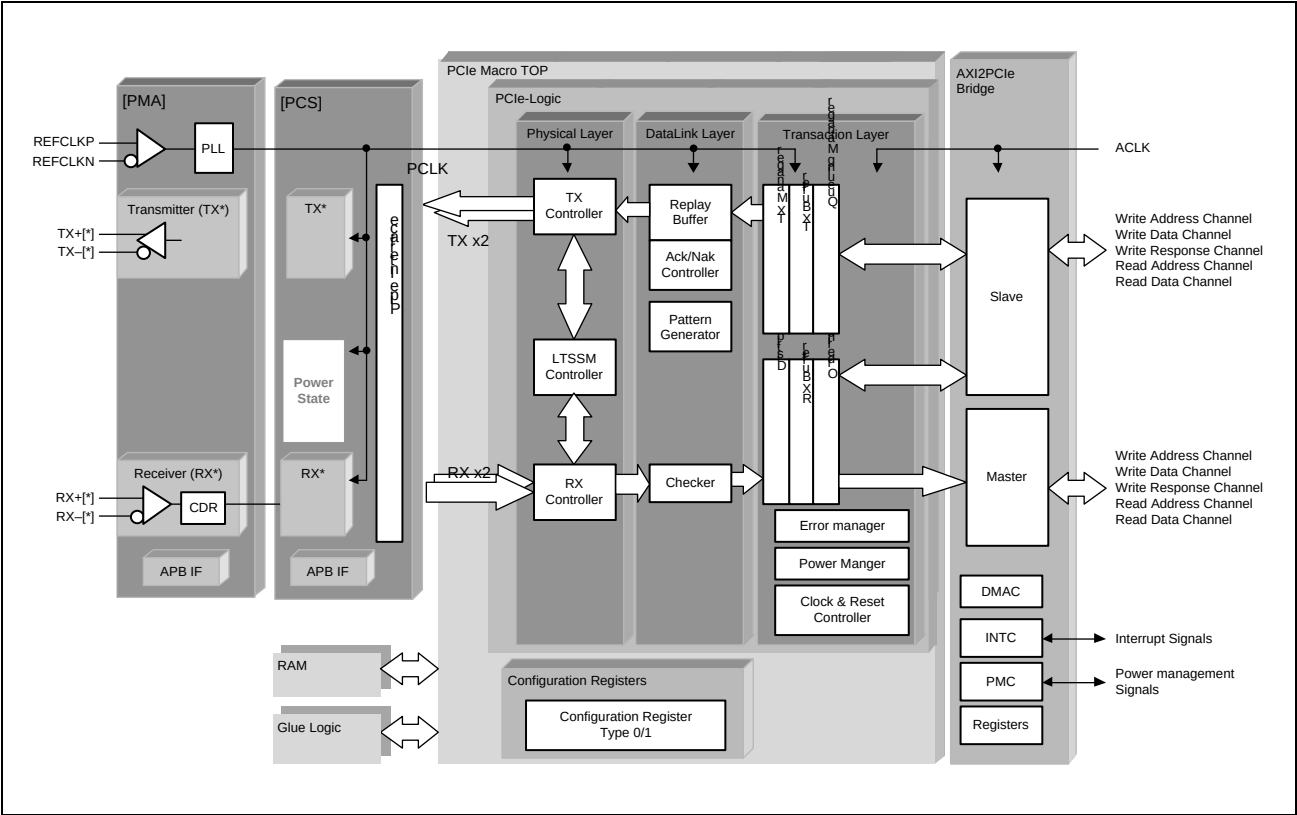
Figure 36.3-1 Block Diagram
