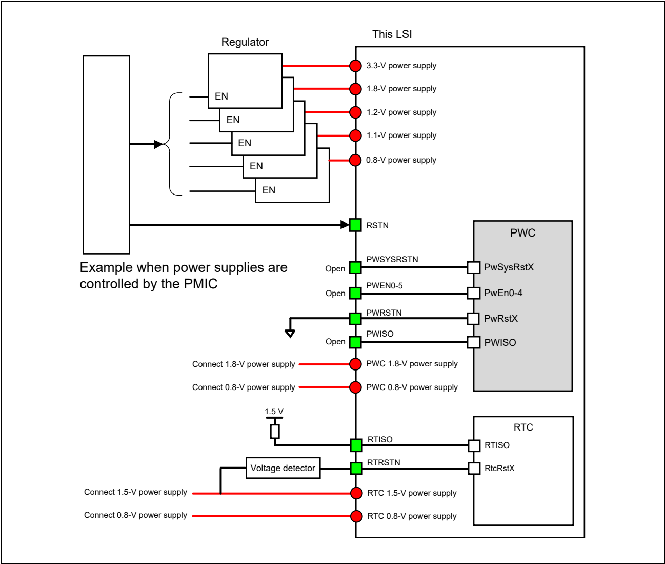
Figure 8.1-2 Example of External Connections when the PWC is not to be Used
