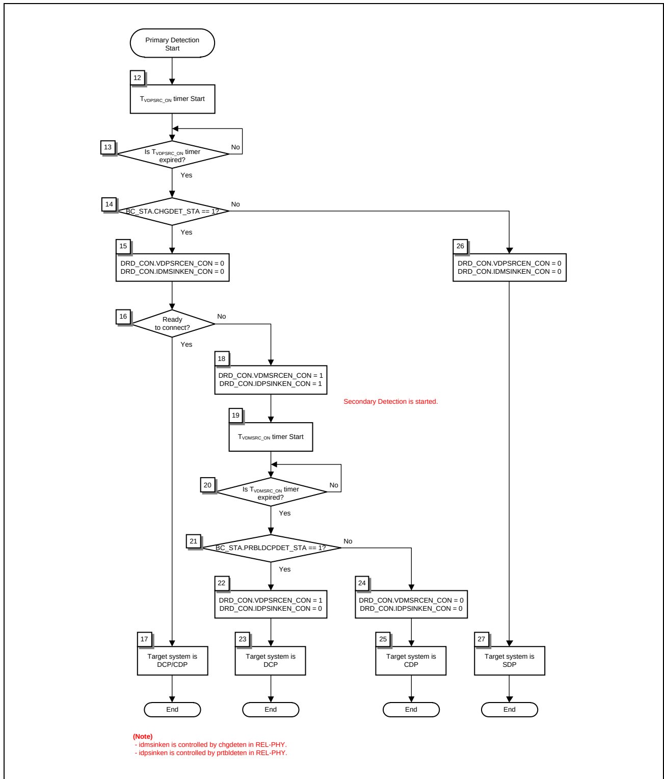
Figure 35.4-8 Good Battery Algorithm Flowchart (Primary &amp; Secondary Detection Flow)
