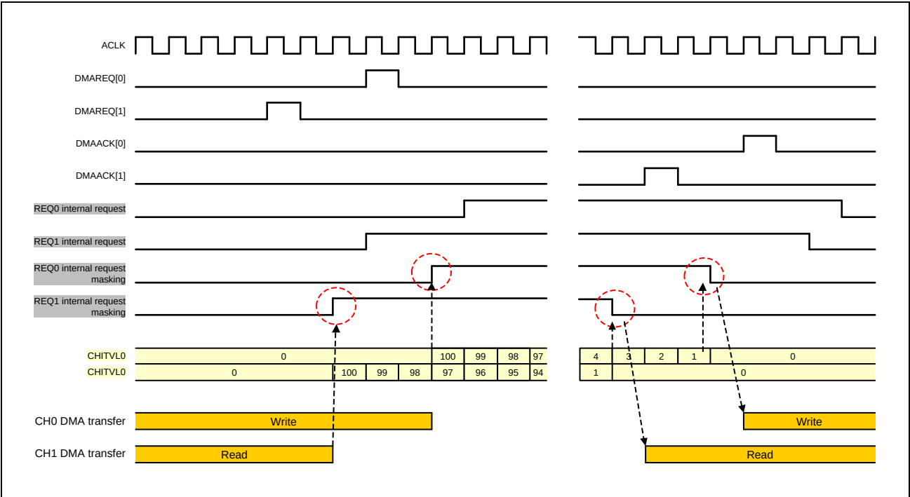
Figure 19.6-22 Interval Counting
