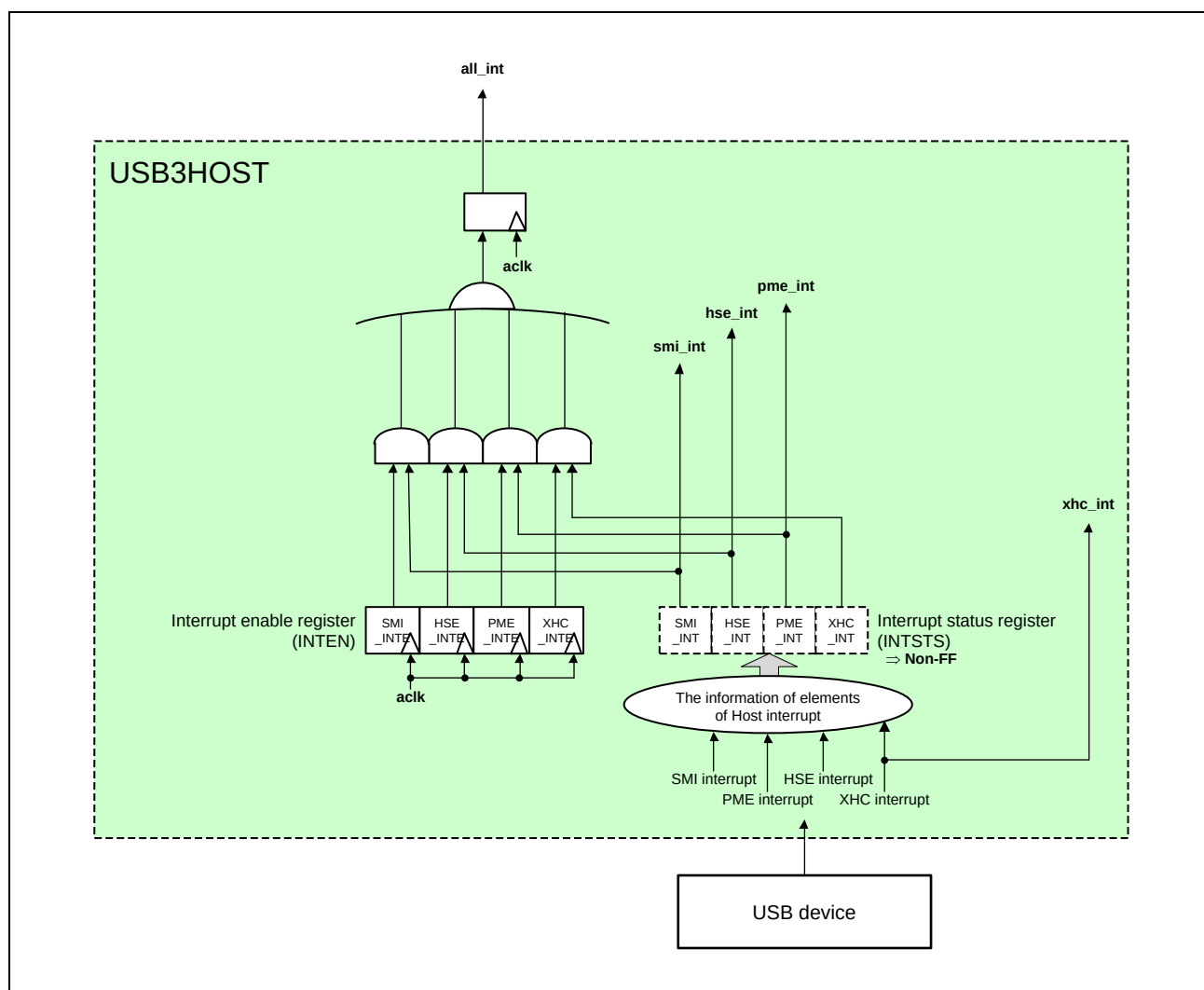
Figure 35.5-1 USB3HOST Interrupts Structure
