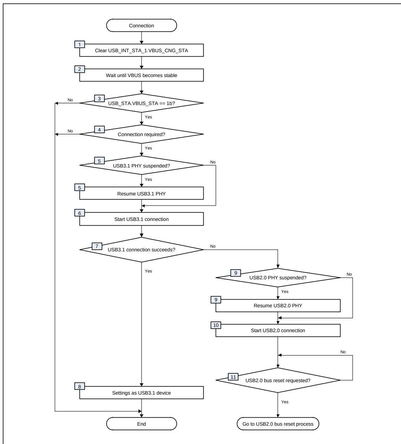
Figure 35.6-21 USB Connection Flow
