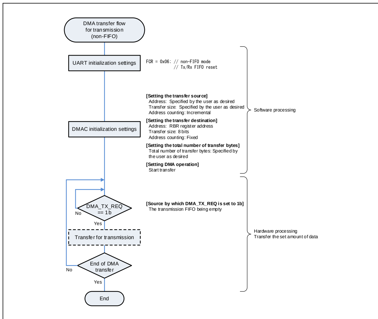
Figure 40.5-5 DMA Transfer Flow for Transmission (in (4) Non-FIFO Mode)
