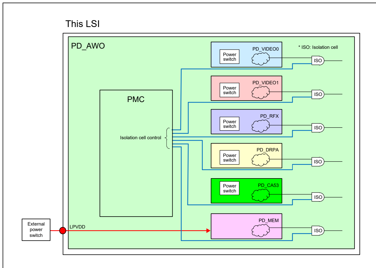
Figure 51.3-3 Isolation Cell Control
