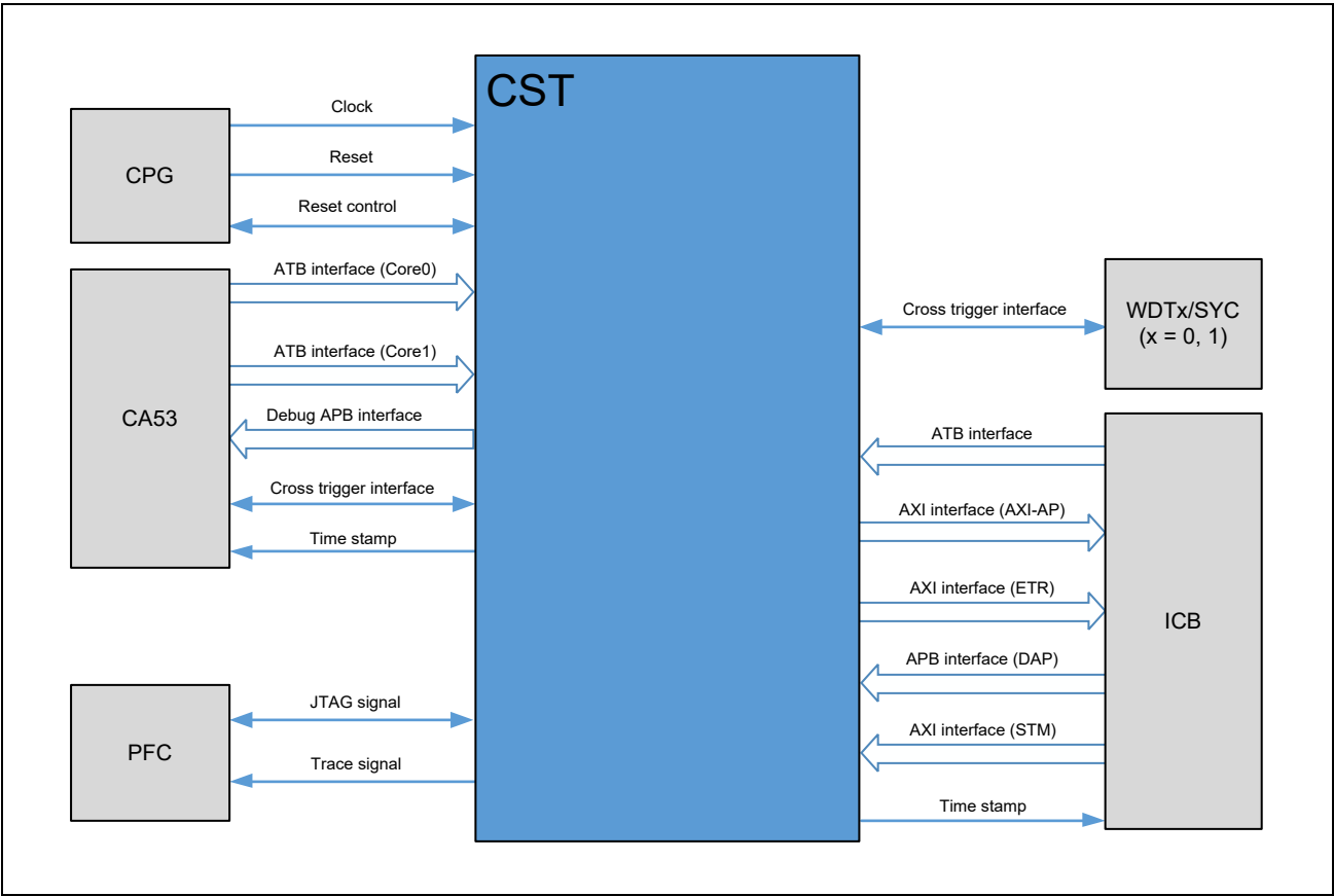
Figure 53.3-1 Connection Configuration
