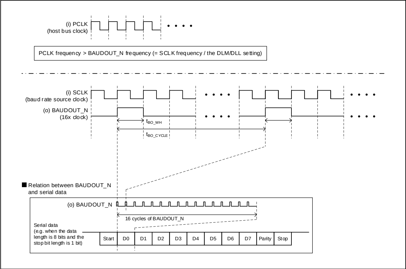
Figure 40.4-1 Clock Timing
