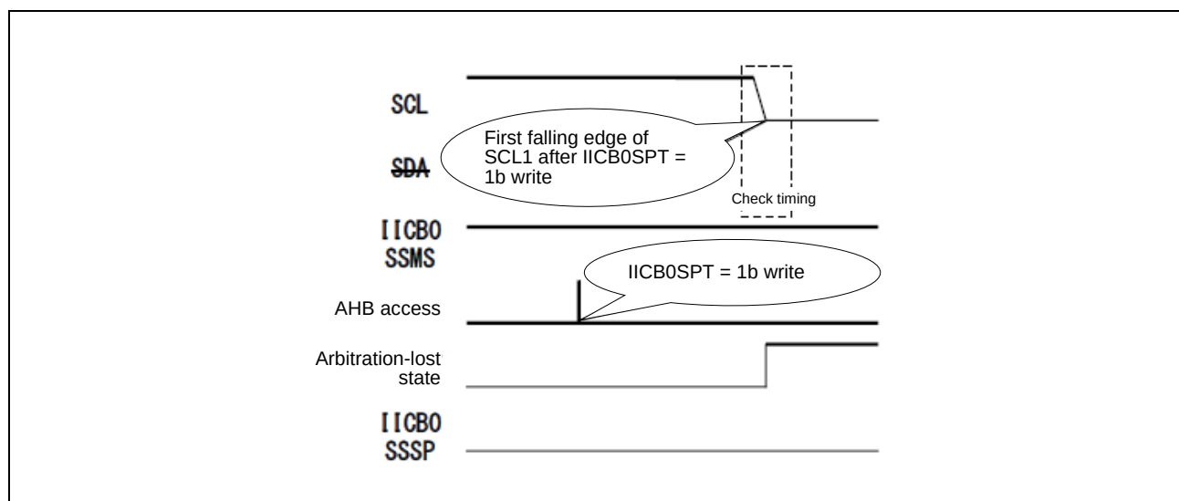
Figure 38.6-14 Arbitration-Lost State in (10)
