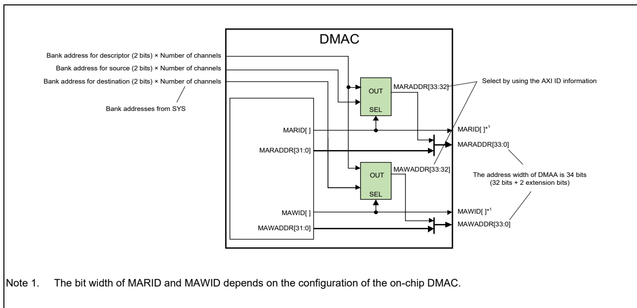
Figure 6.4-2 Schematic of Address Bus Width Extension (Address Extension 2)
