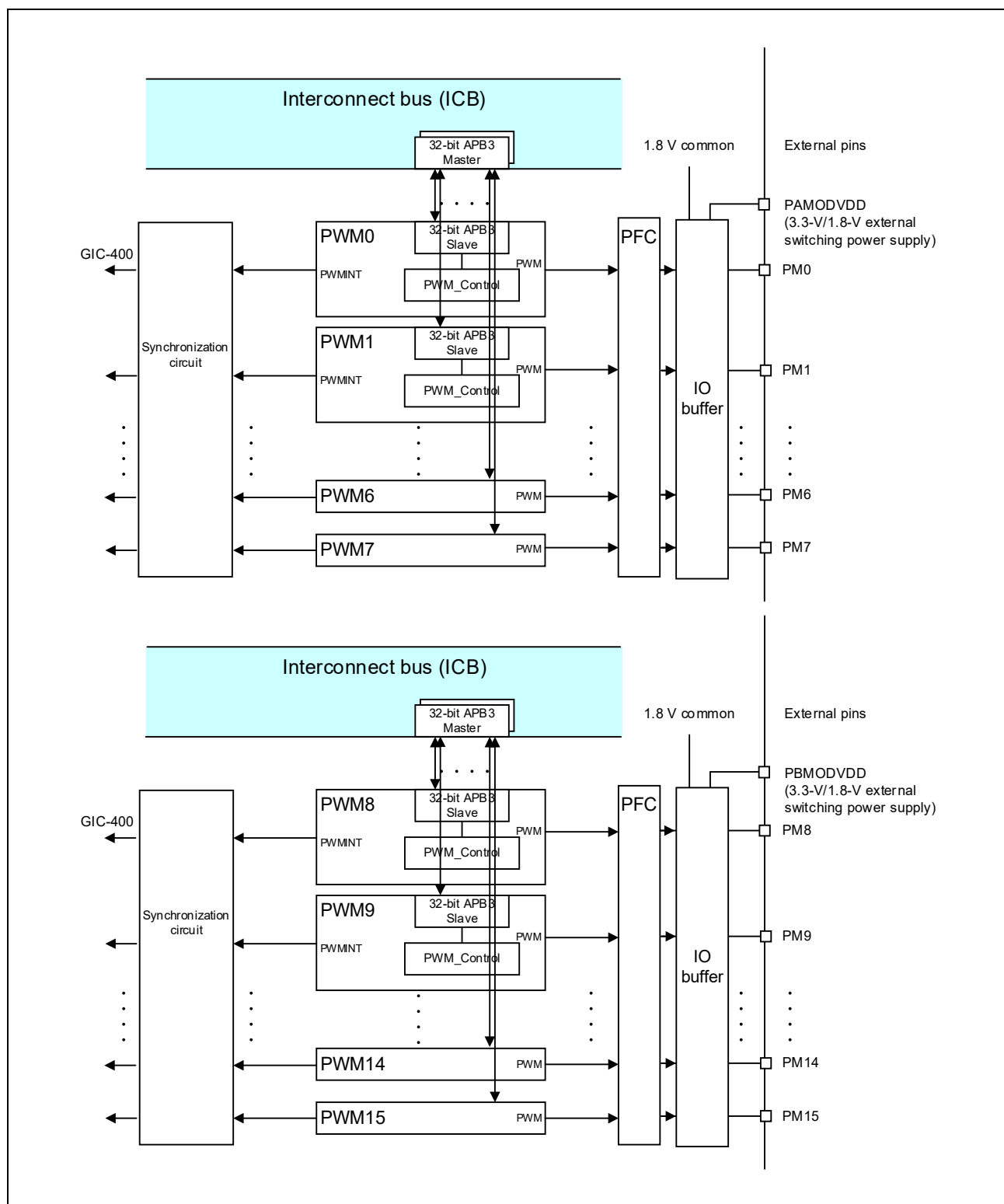
Figure 17.1-2 Schematic of the PWM Connection
