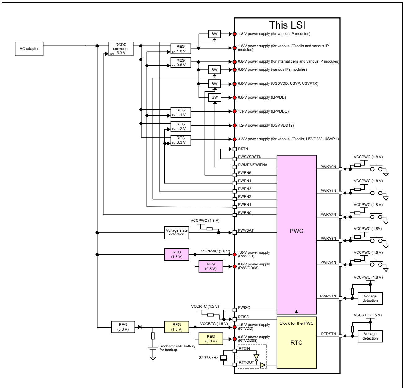
Figure 50.5-1 Example System Configuration for External Power Supplies
