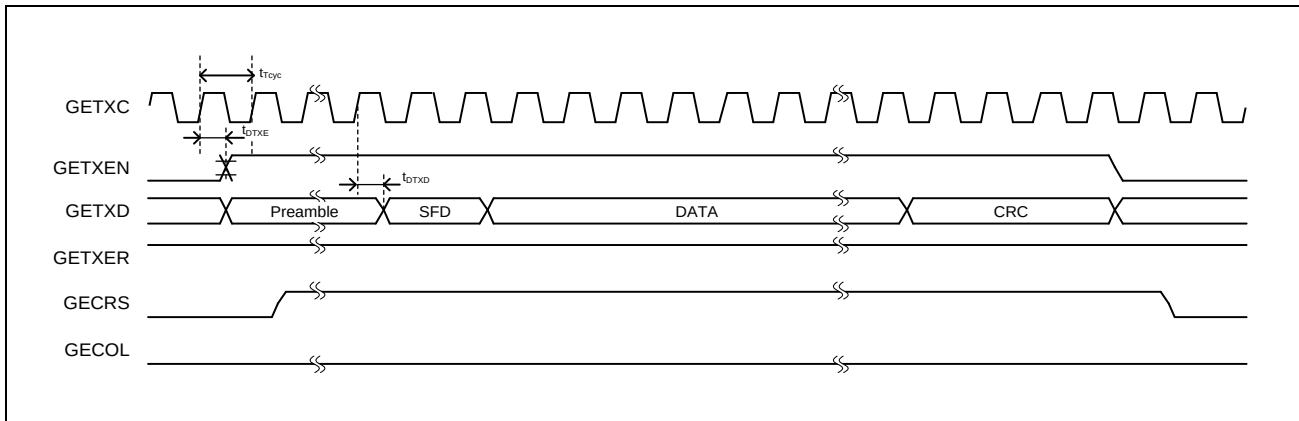
Figure 54.5-4 Transmission Timing
