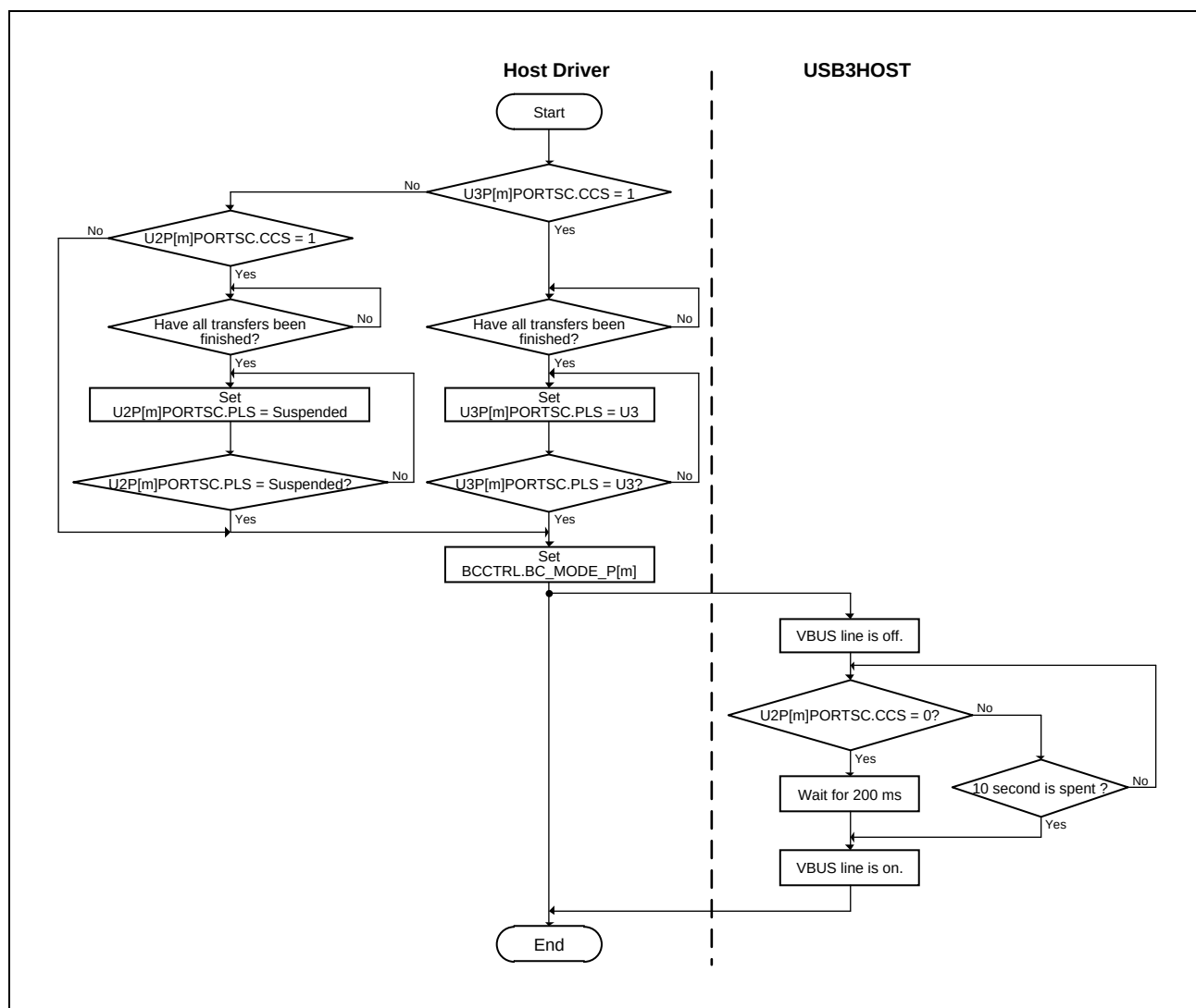
Figure 35.5-2 Host Driver's Flow to Set BC Mode (m = 1)
