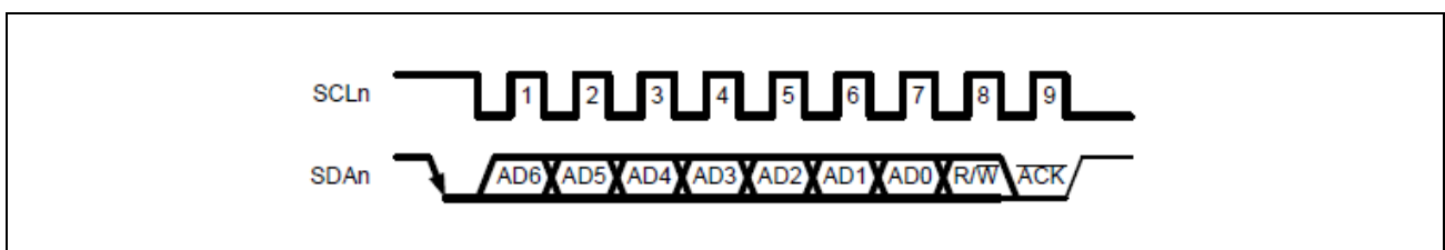
Figure 38.6-5 Acknowledge ( \overline{ACK} )
