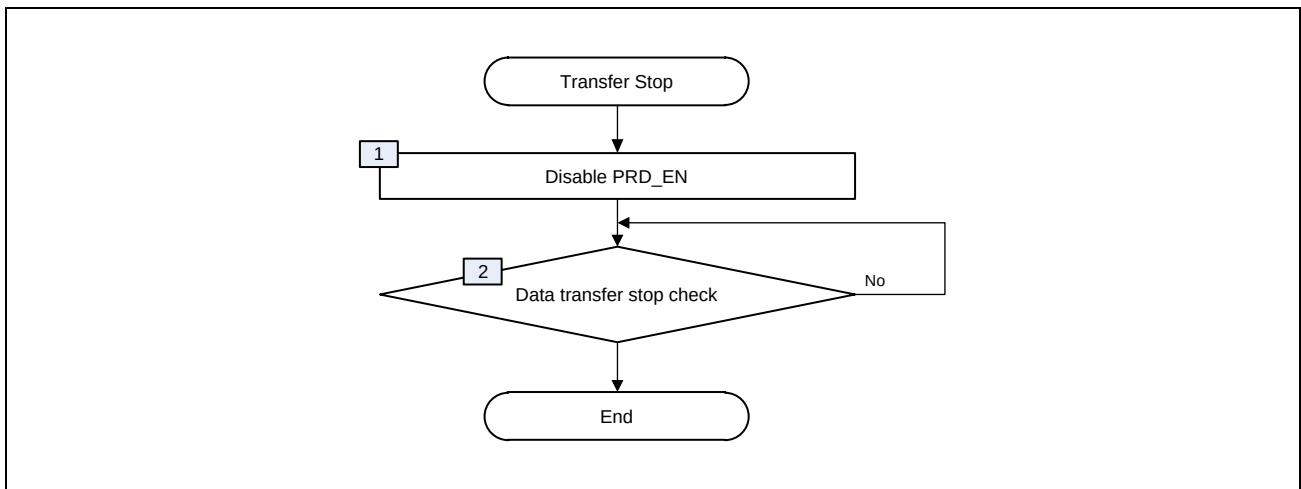
Figure 35.6-39 Transfer Stop Flow
