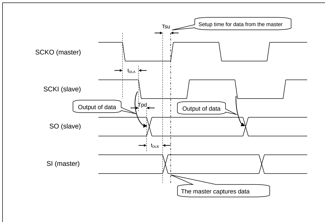
Figure 39.6-2 Timing of Data Reception by the Master
