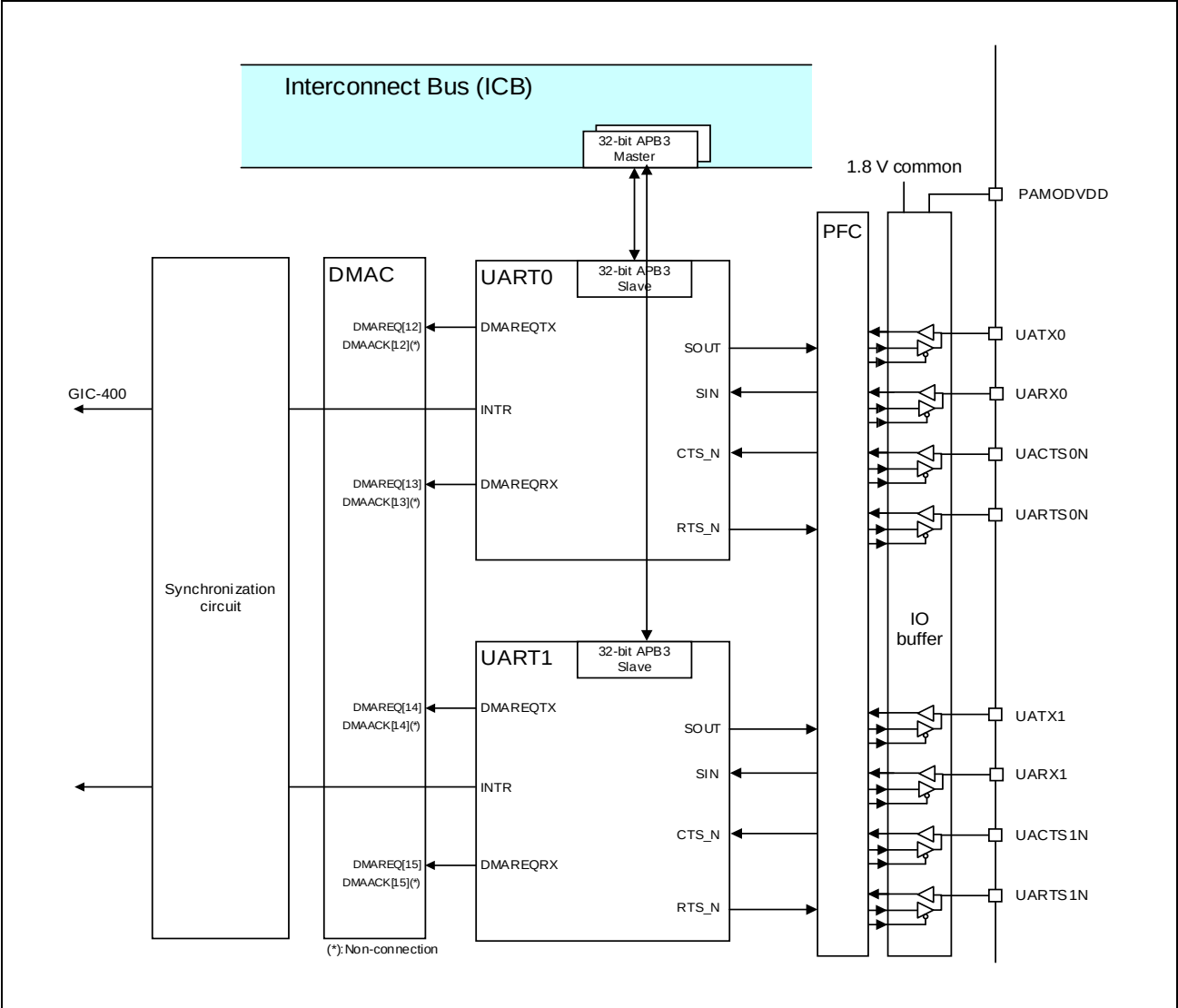
Figure 40.1-1 Connection Configuration
