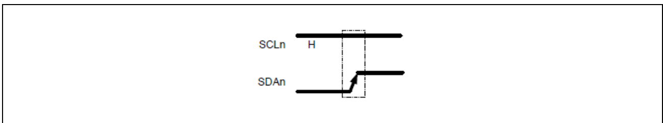
Figure 38.6-6 Stop Condition
