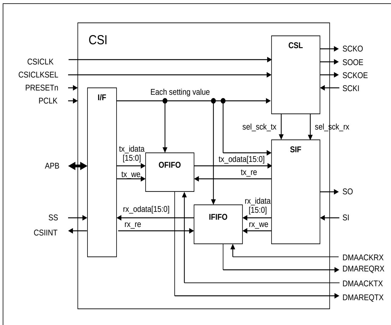
Figure 39.1-1 Block Diagram
