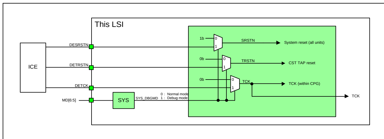
Figure 48.6-21 Block Diagram
