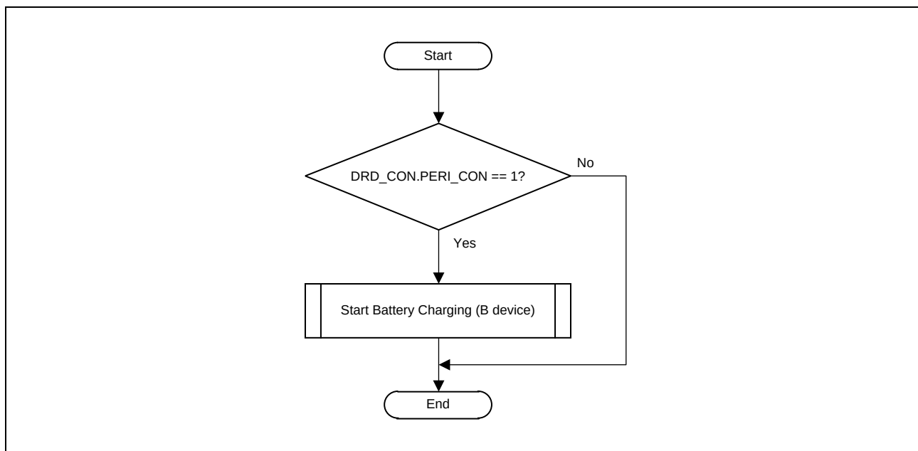
Figure 35.4-5 Prior Confirmation Flow for the Battery Charging of B-Device
