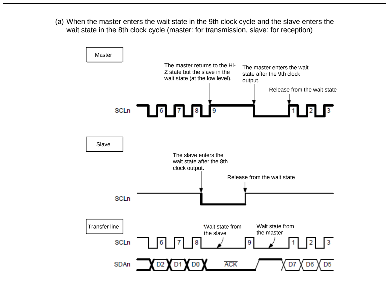
Figure 38.6-7 Wait (1/2)
