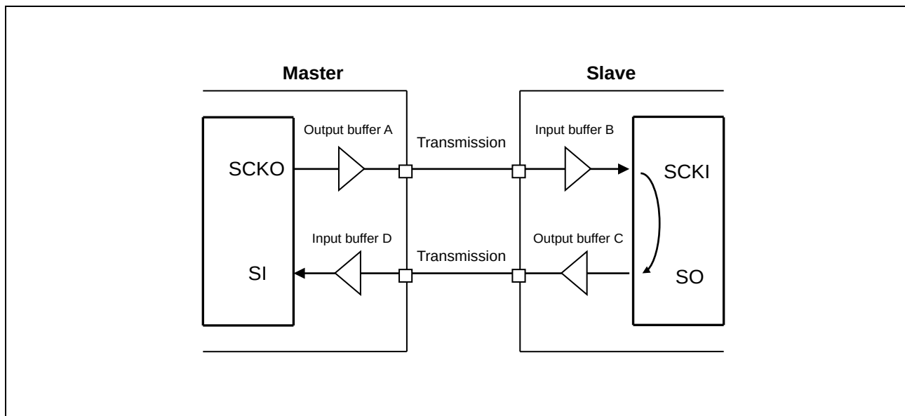
Figure 39.6-1 Master and Slave Connection
