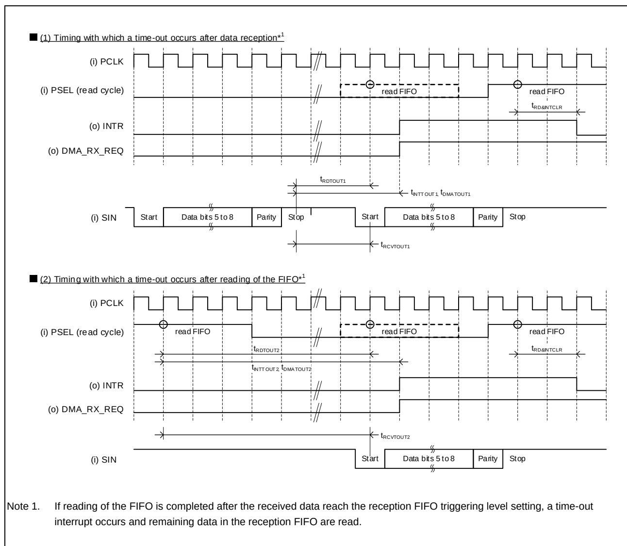
Figure 40.4-8 Time-out Timing
