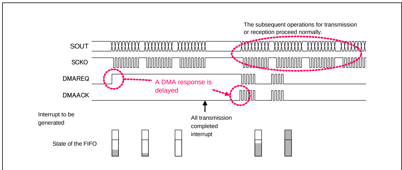
Figure 39.4-7 CSI All Transmission Completed Interrupt
