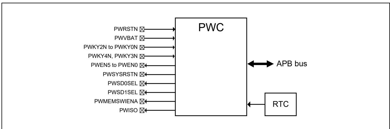
Figure 50.2-1 Connection Configuration of the PWC
