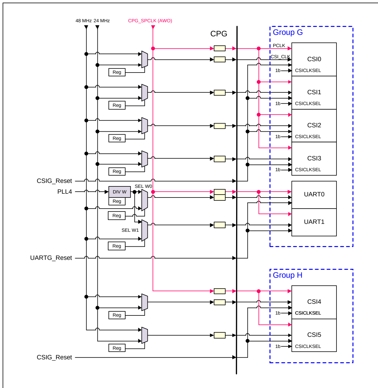
Figure 48.6-20 Block Diagram of Groups G and H
