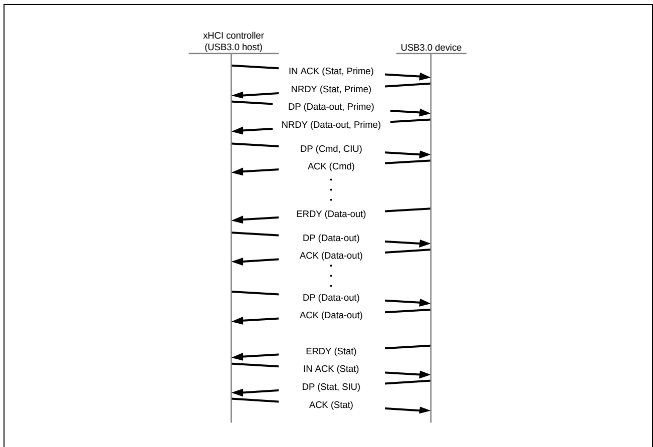
Figure 35.6-36 Example SuperSpeed UASP Data-OUT Transfer
