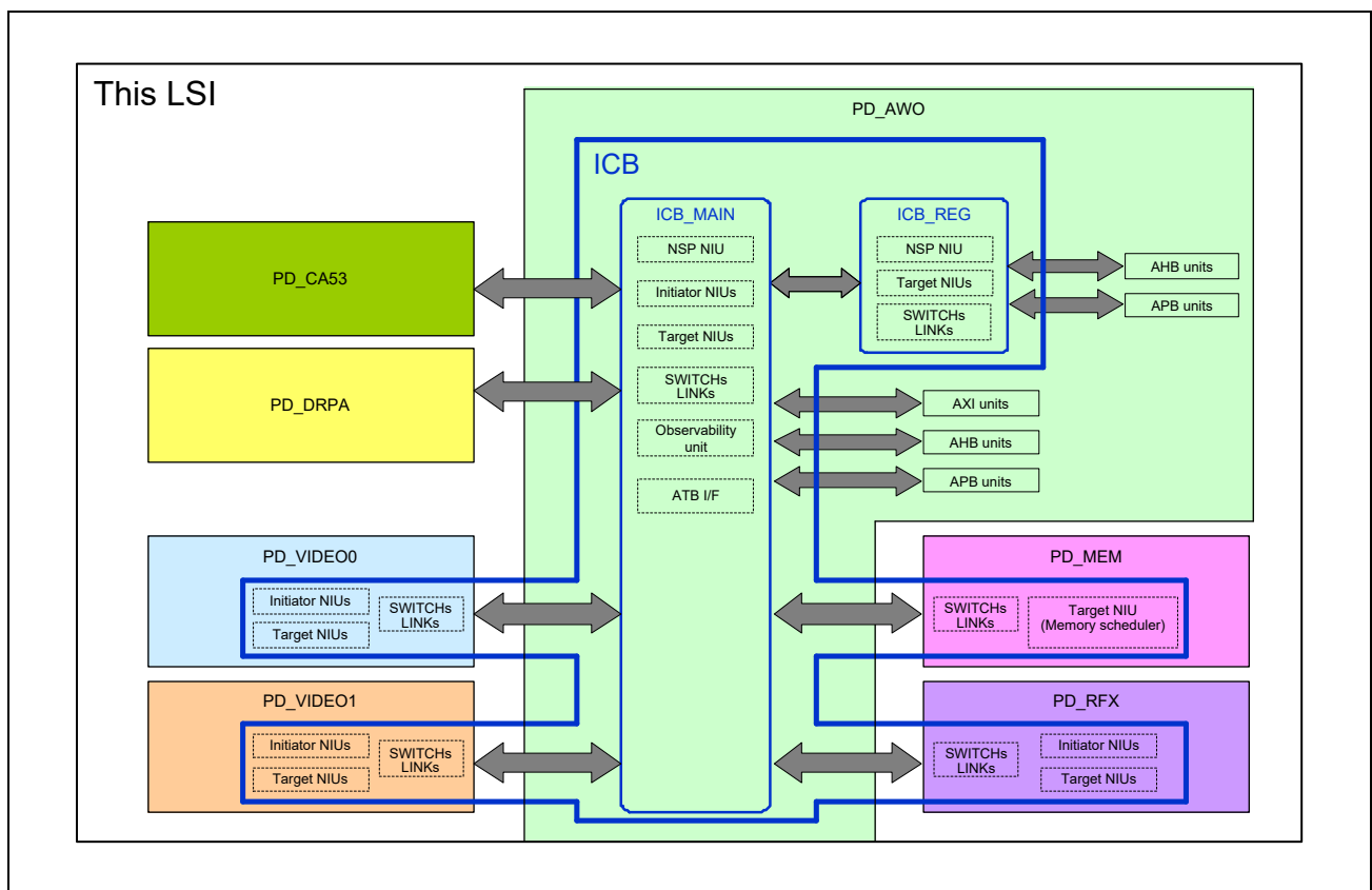
Figure 49.2-1 Internal Configuration
