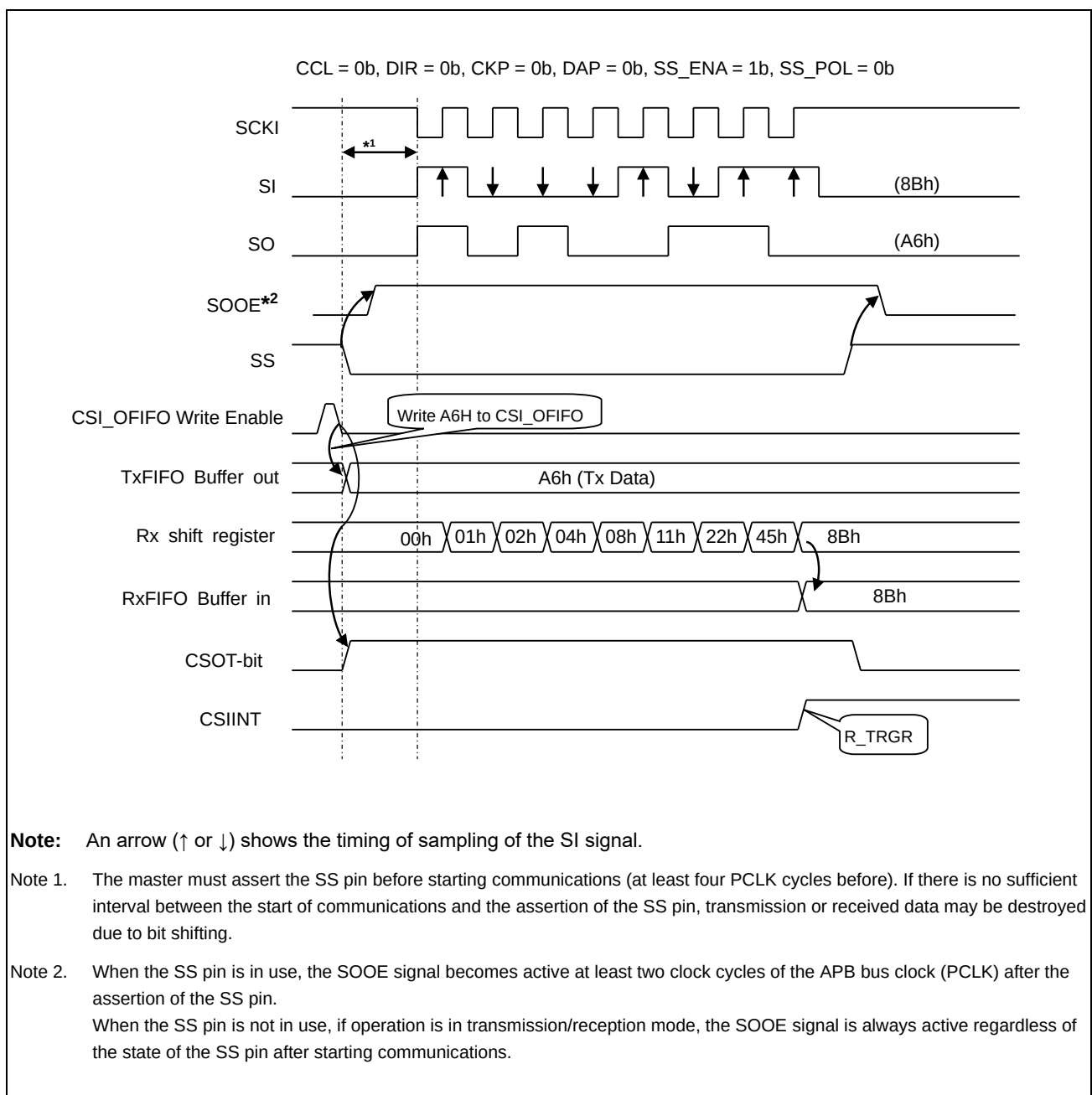
Figure39.5-3 Timing of Single-Word Transfer (in Slave Transmission/Reception Mode)
