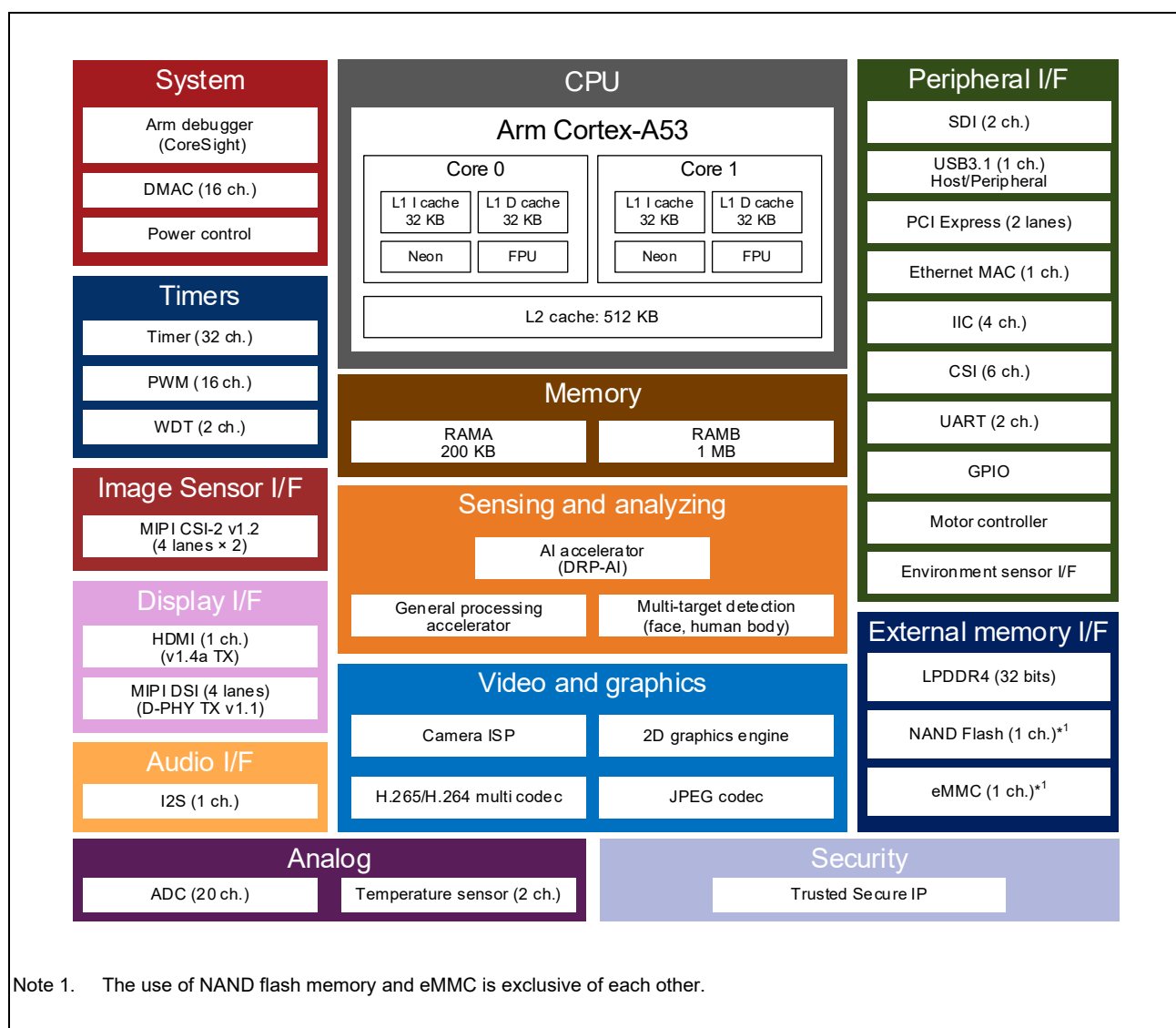
Figure 1.1-1 Diagram of Functional Overview
