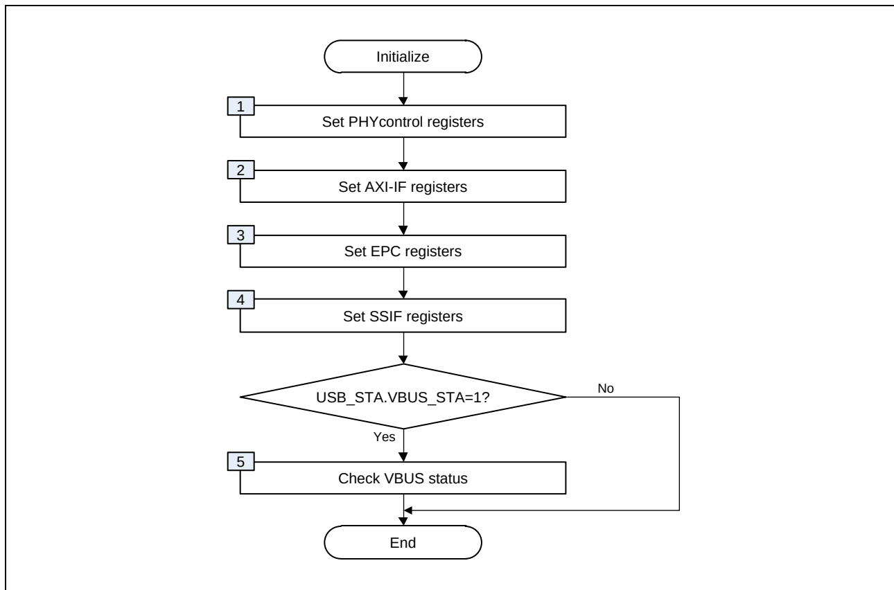
Figure 35.6-19 Initialization Flow
