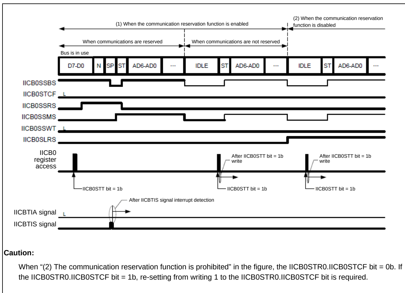
Figure 38.6-16 Timing of Effective Writing to the IICB0DAT Register
