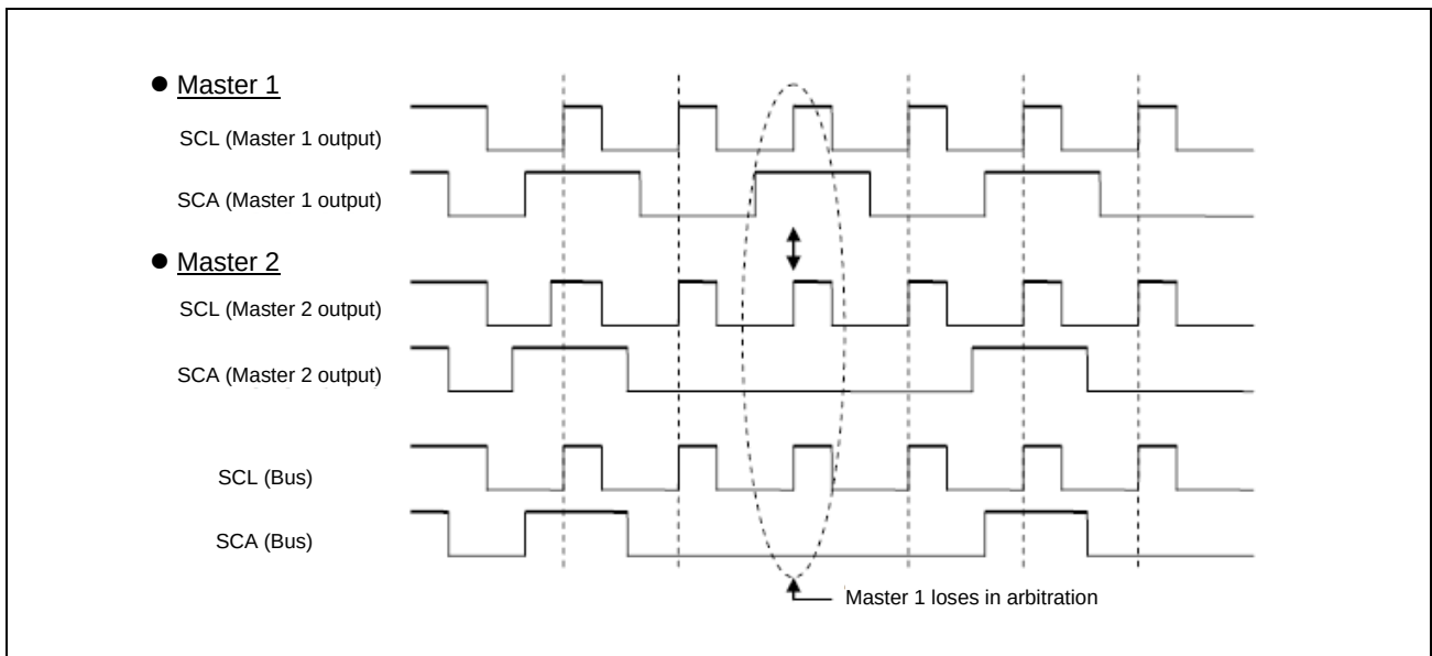
Figure 38.6-11 Example of Arbitration Loss
