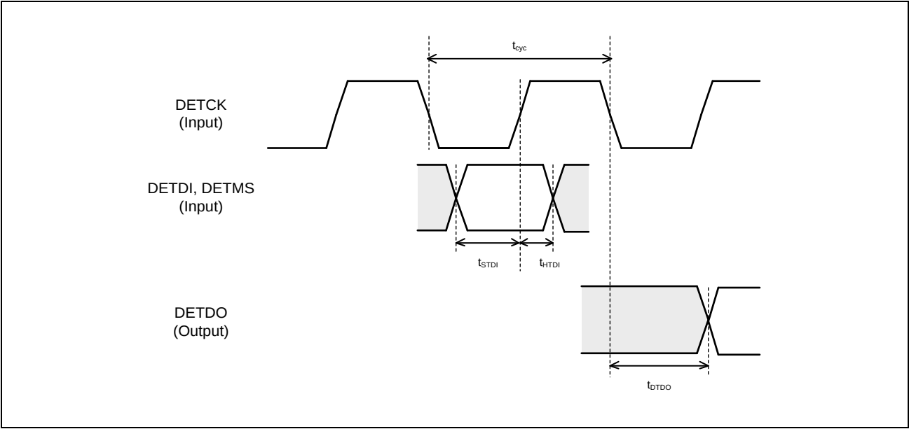
Figure 54.5-17 JTAG Timing
