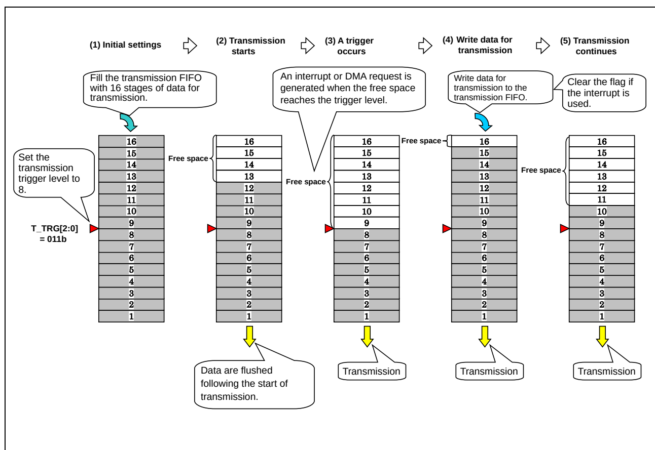
Figure 39.4-18 Operation of the Transmission FIFO when the Transmission Trigger Level is Set
