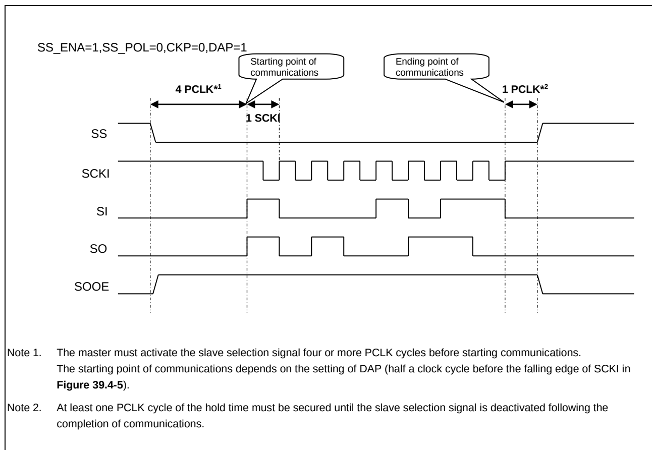
Figure 39.4-5 Slave Selection Signal Control Timing (when DAP = 1b for Slave)
