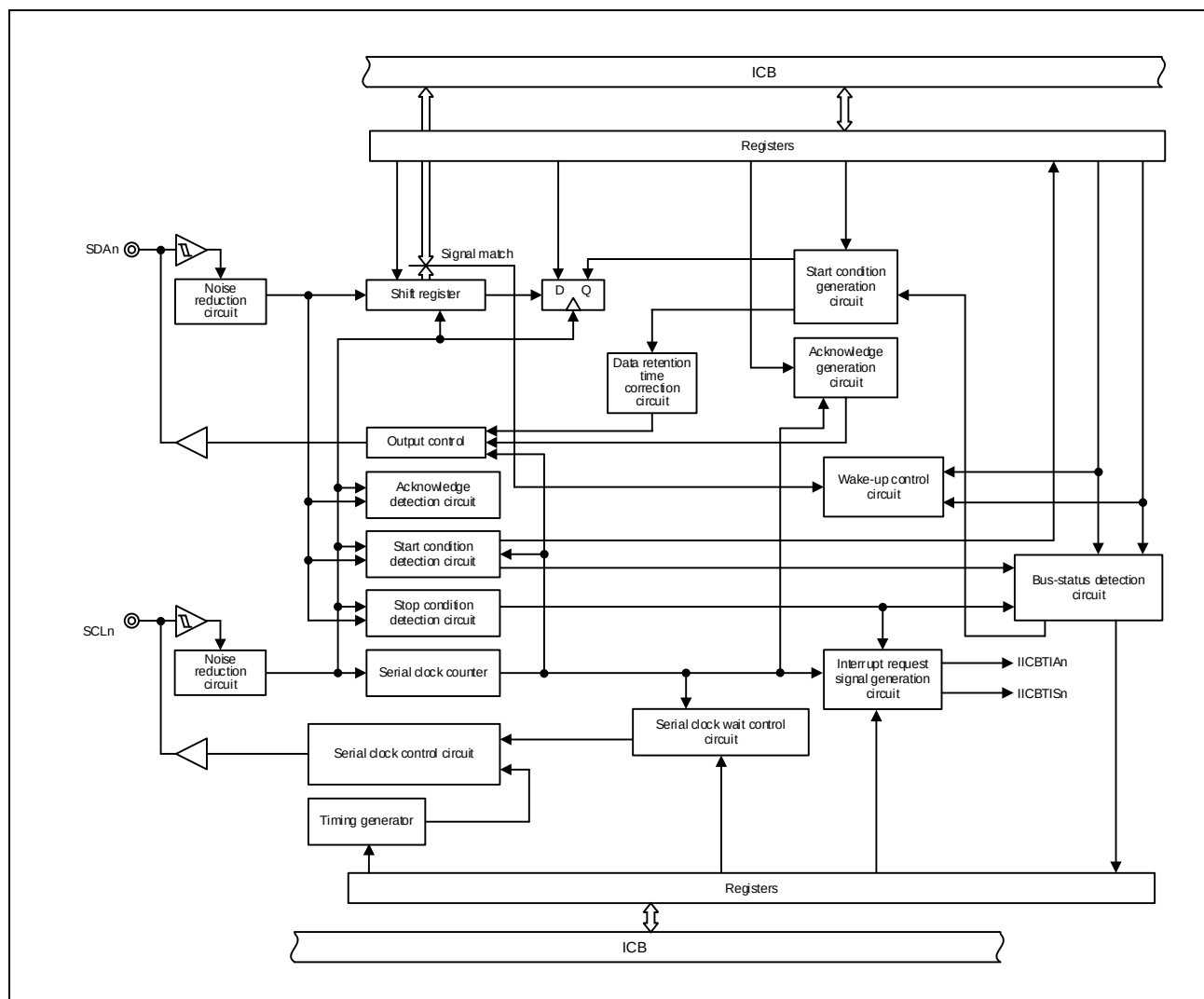
Figure 38.2-1 Block Diagram
