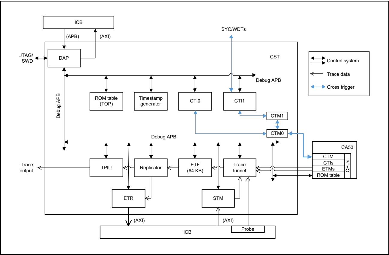
Figure 53.2-1 Block Diagram
