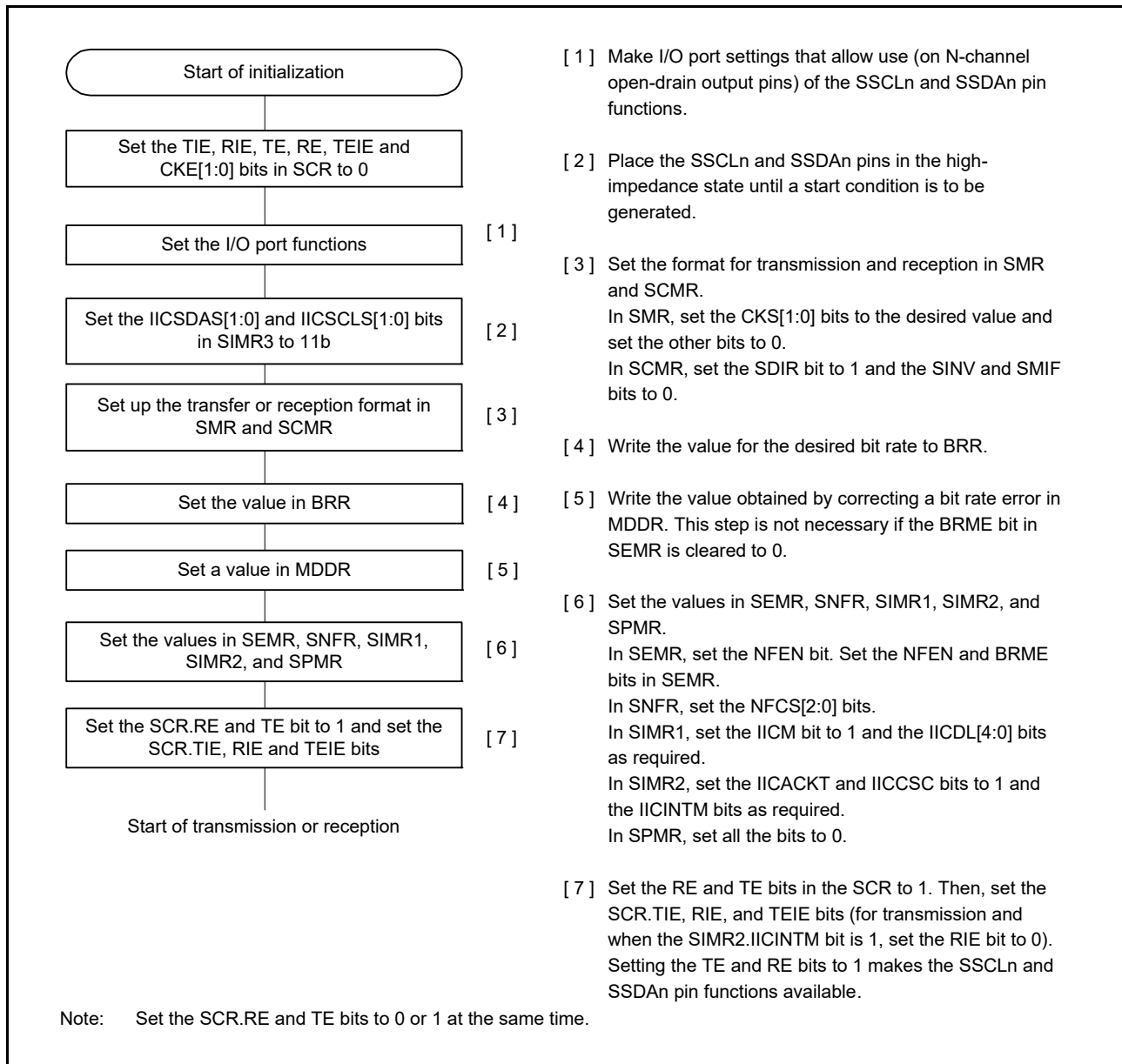
Figure 23.50 Example of the Flowchart of SCI Initialization (for Simple I 2 C Mode)
