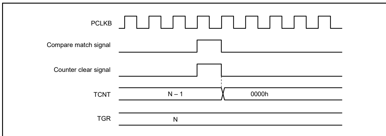
Figure 19.108 Counter Clear Timing (Compare Match) (MTU5)
