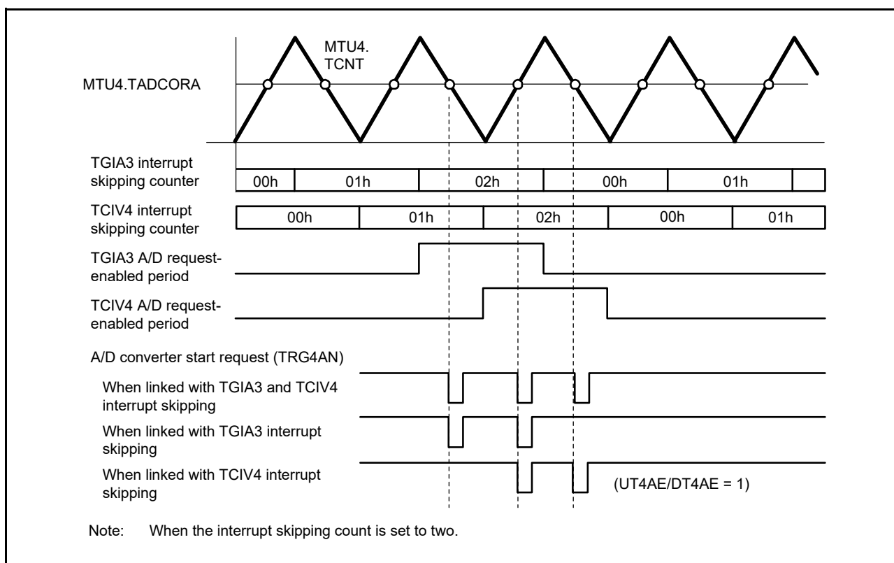
Figure 19.86 Example of A/D Converter Start Request Signal (TRG4AN) Operation Linked with Interrupt Skipping Function 1 (UT4AE and DT4AE = 1)
