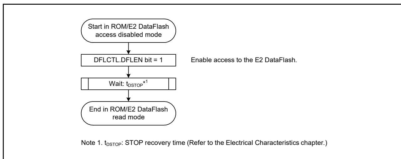
Figure 31.6 Procedure for Transition from E2 DataFlash Access Disabled Mode to ROM/E2 DataFlash Read Mode
