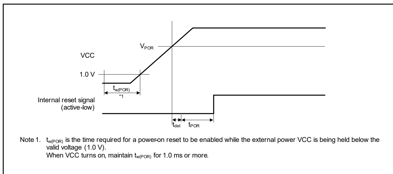
Figure 32.39 Power-On Reset Timing
