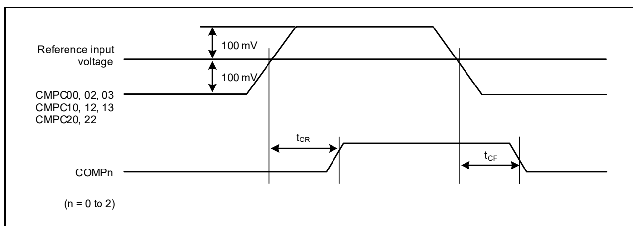
Figure 32.37 Comparator Response Time
