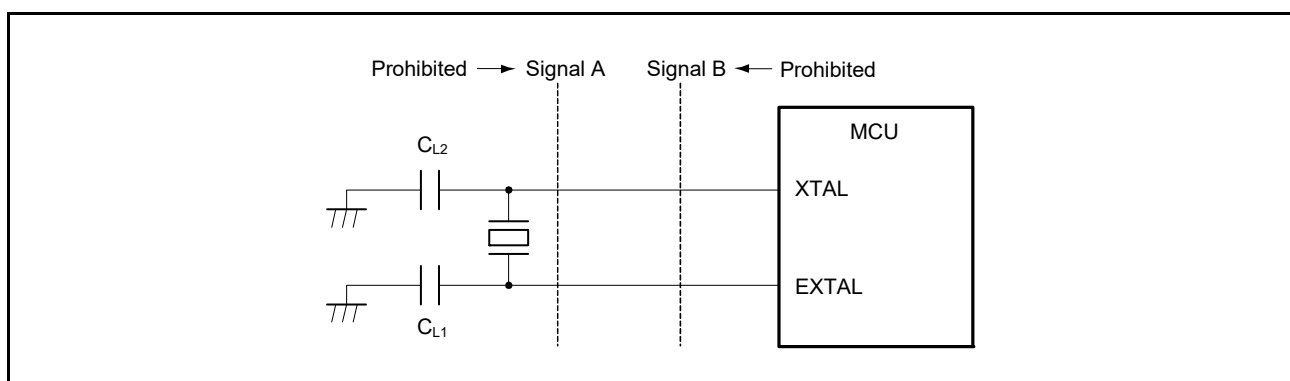
Figure 9.6 Notes on Board Design for Oscillation Circuit
