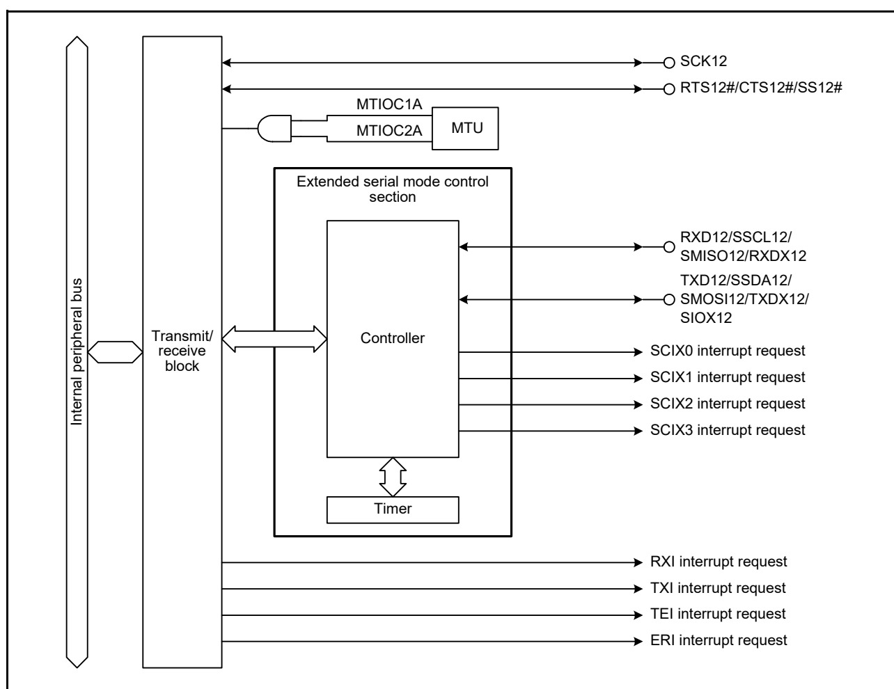
Figure 23.2 Block Diagram of SCIf (SCI12)
