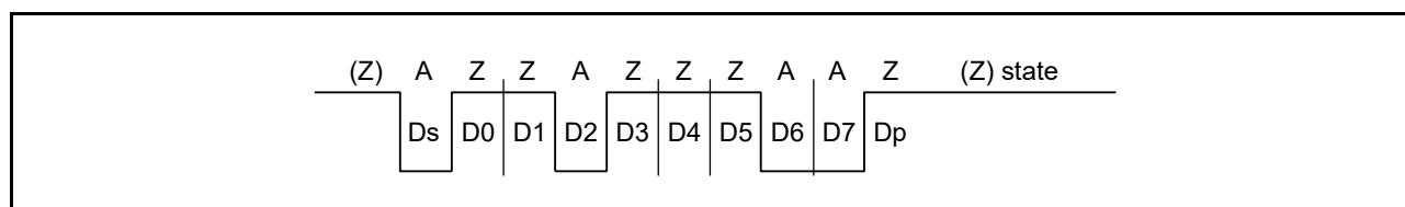
Figure 23.34 Direct Convention (SDIR in SCMR = 0, SINV in SCMR = 0, PM in SMR = 0)
