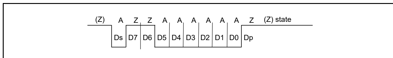
Figure 23.35 Inverse Convention (SDIR in SCMR = 1, SINV in SCMR = 1, PM in SMR = 1)
