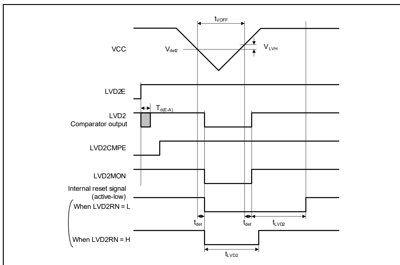
Figure 32.42 Voltage Detection Circuit Timing ( V_{det2} )
