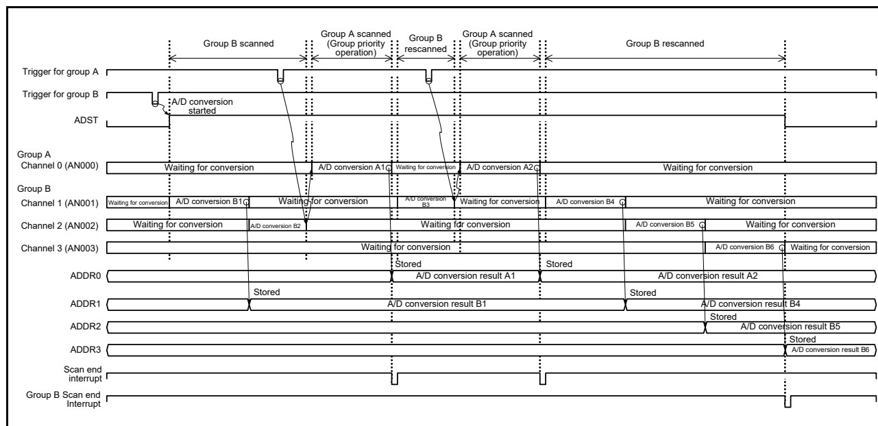
Figure 26.17 Example 2 of Group Priority Operation: Group A Trigger Input during Group B Rescan, With Rescan Setting (ADGSPCR.GBRSCN = 1, ADGSPCR.GBRP = 0, ADGSPCR.LGRRS = 0)
