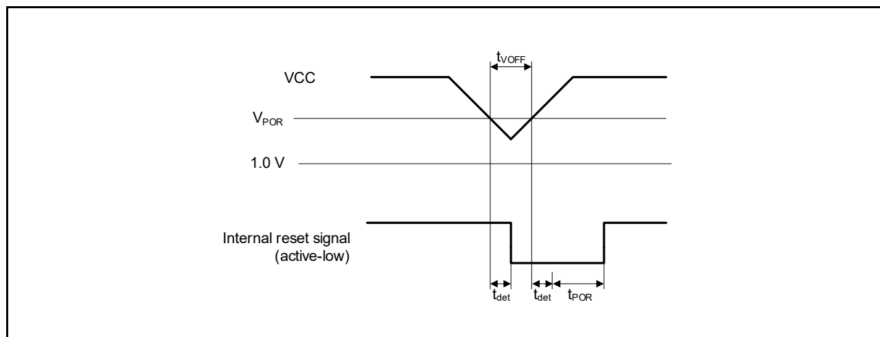
Figure 32.38 Voltage Detection Reset Timing
