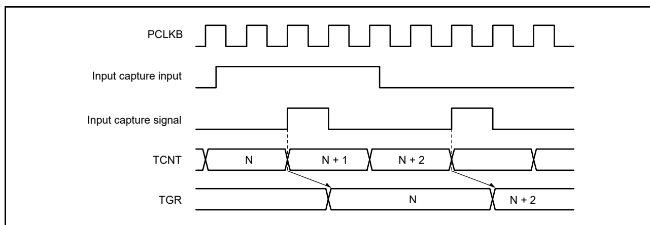
Figure 19.106 Input Capture Input Signal Timing
