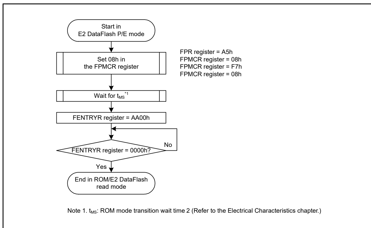
Figure 31.10 Procedure for Transition from E2 DataFlash P/E Mode to ROM/E2 DataFlash Read Mode
