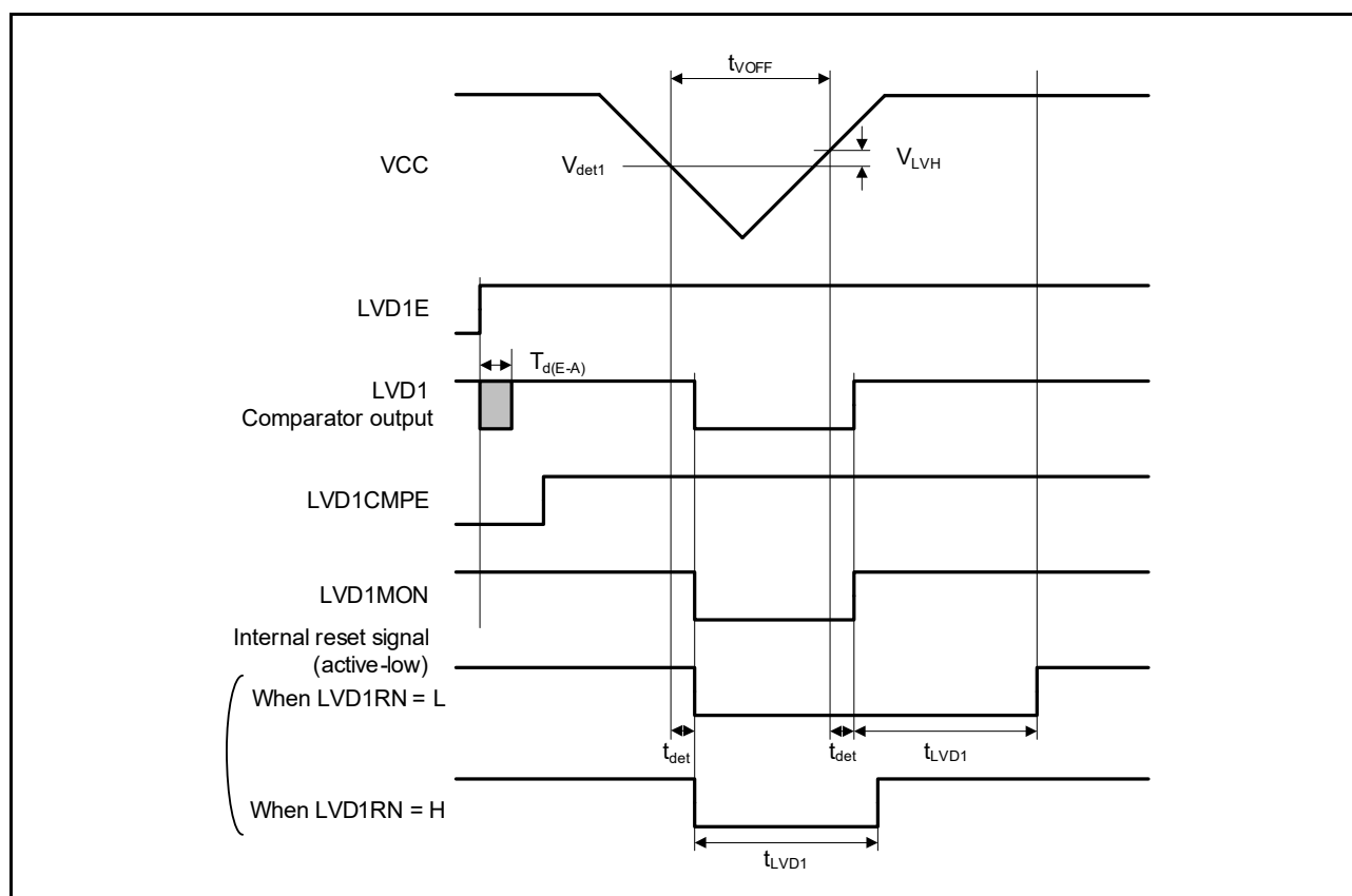
Figure 32.41 Voltage Detection Circuit Timing ( V_{det1} )
