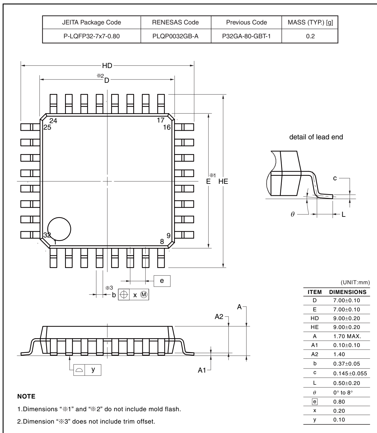
Figure B 32-Pin LQFP (PLQP0032GB-A)
