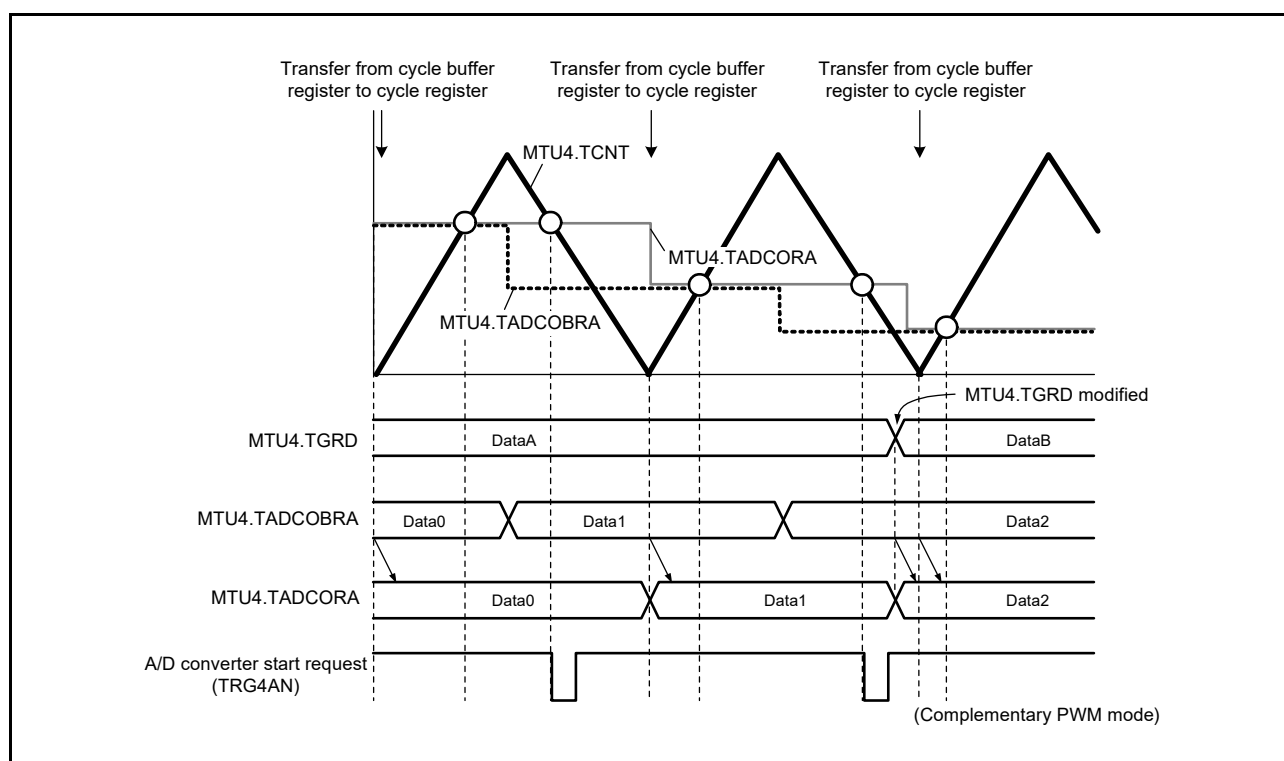
Figure 19.85 Example of A/D Converter Start Request Signal (TRG4AN) and Buffer Transfer Operation
