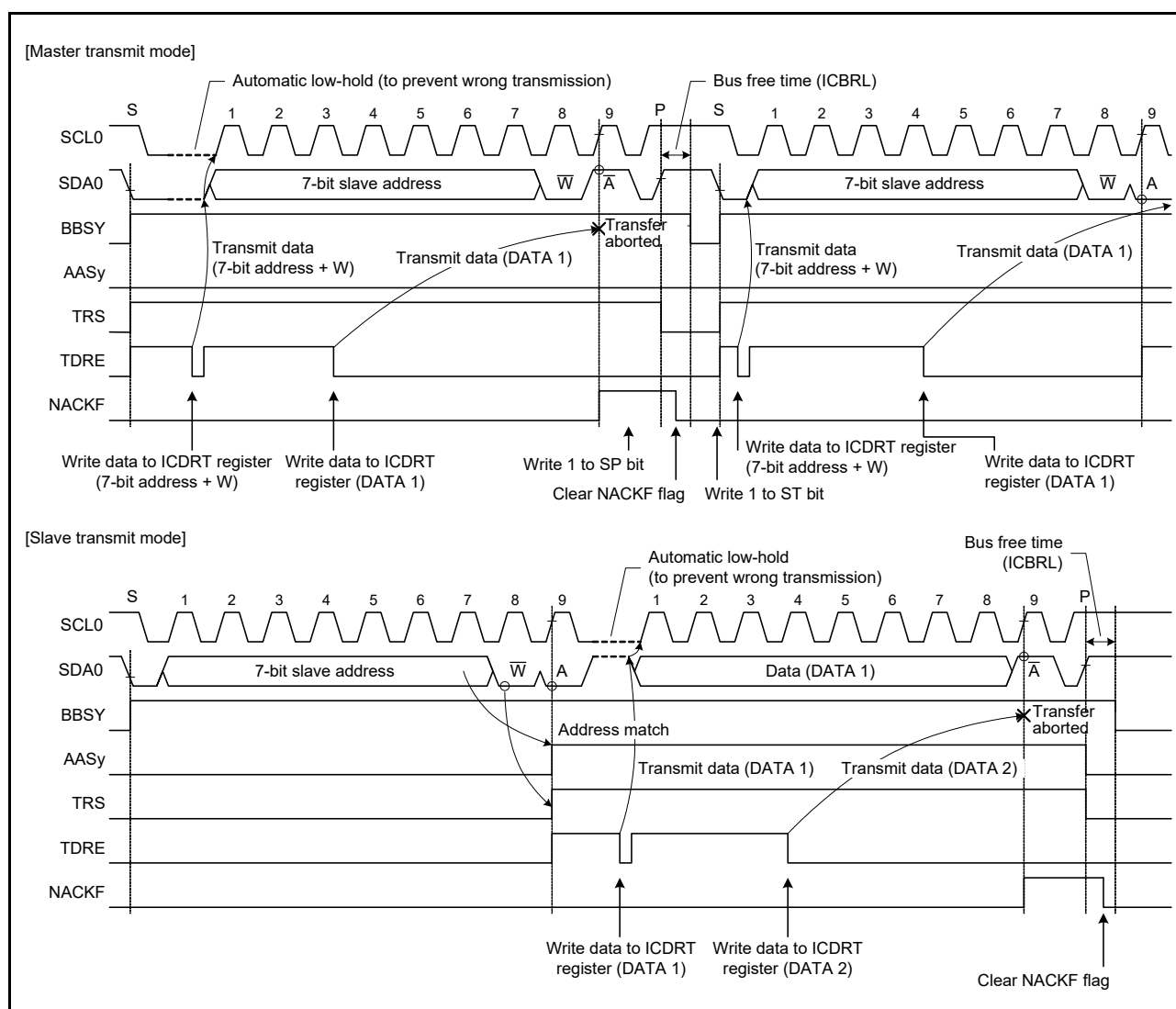
Figure 24.31 Abort of Data Transfer When NACK is Received (NACKE = 1)
