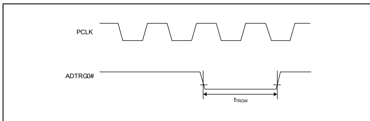
Figure 32.29 A/D Converter External Trigger Input Timing
