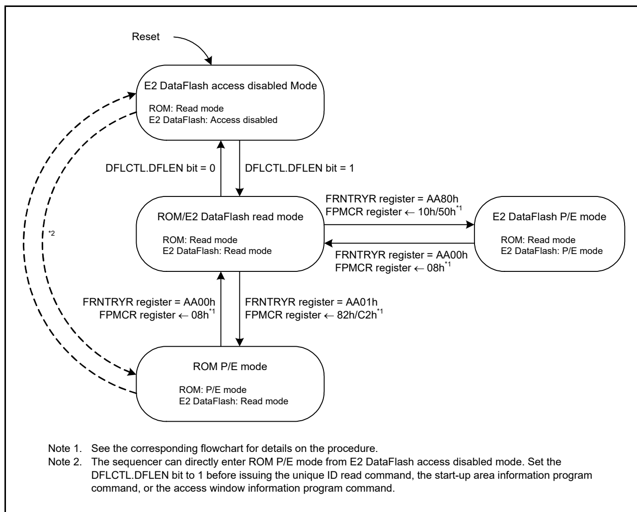
Figure 31.5 Mode Transitions of the Flash Memory
