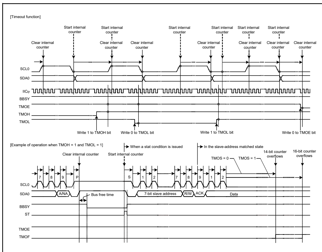
Figure 24.39 Timeout Function
