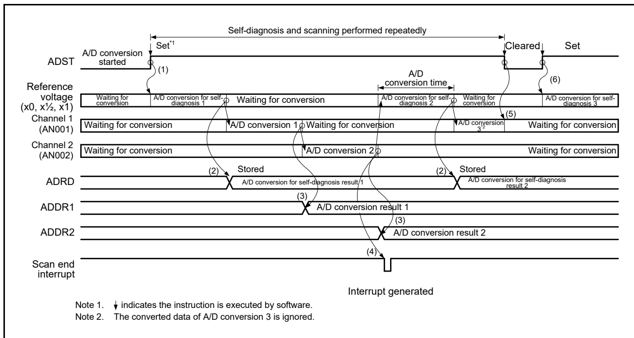
Figure 26.11 Example of Operation in Continuous Scan Mode (Basic Operation; AN001 and AN002 Selected + Self-Diagnosis)
