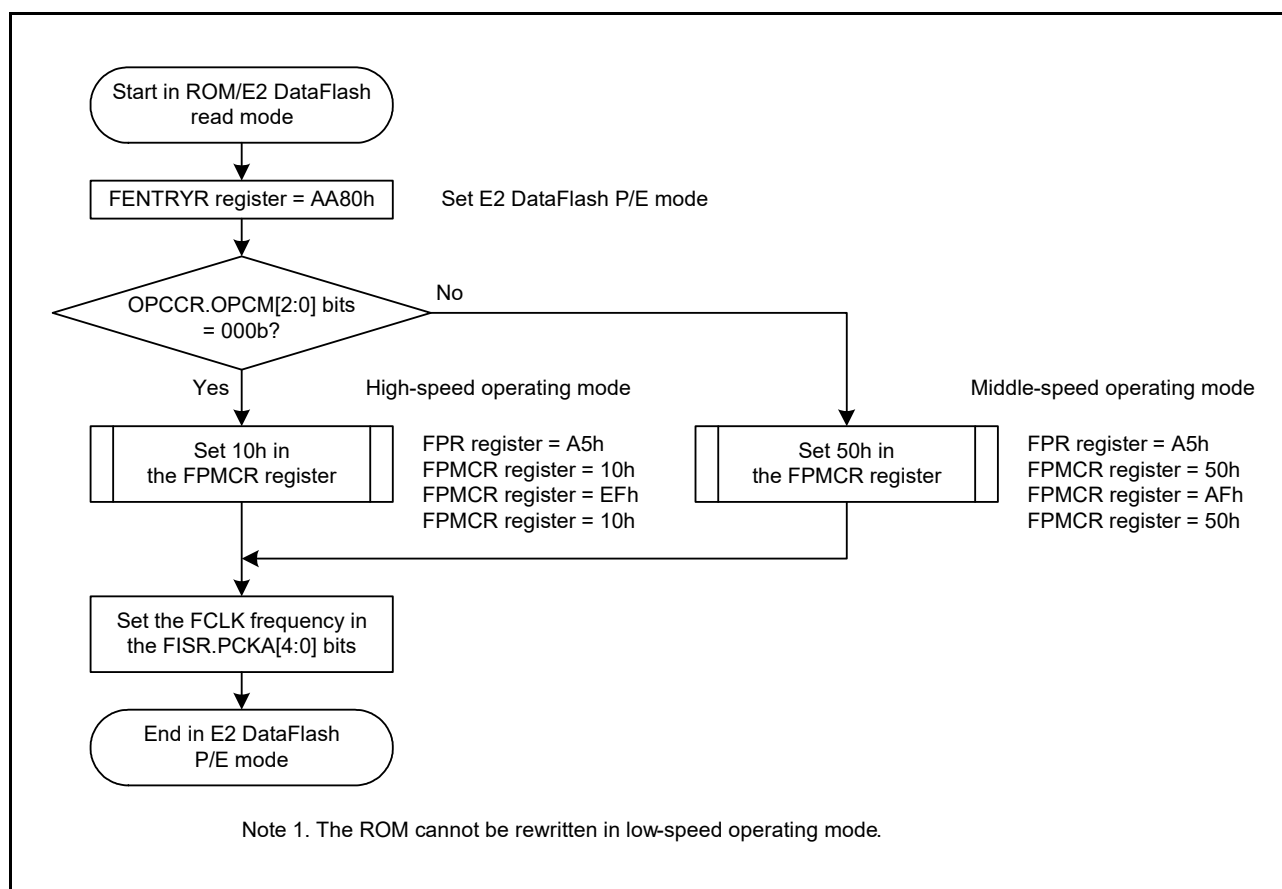
Figure 31.8 Procedure for Transition from ROM/E2 DataFlash Read Mode to E2 DataFlash P/E Mode
