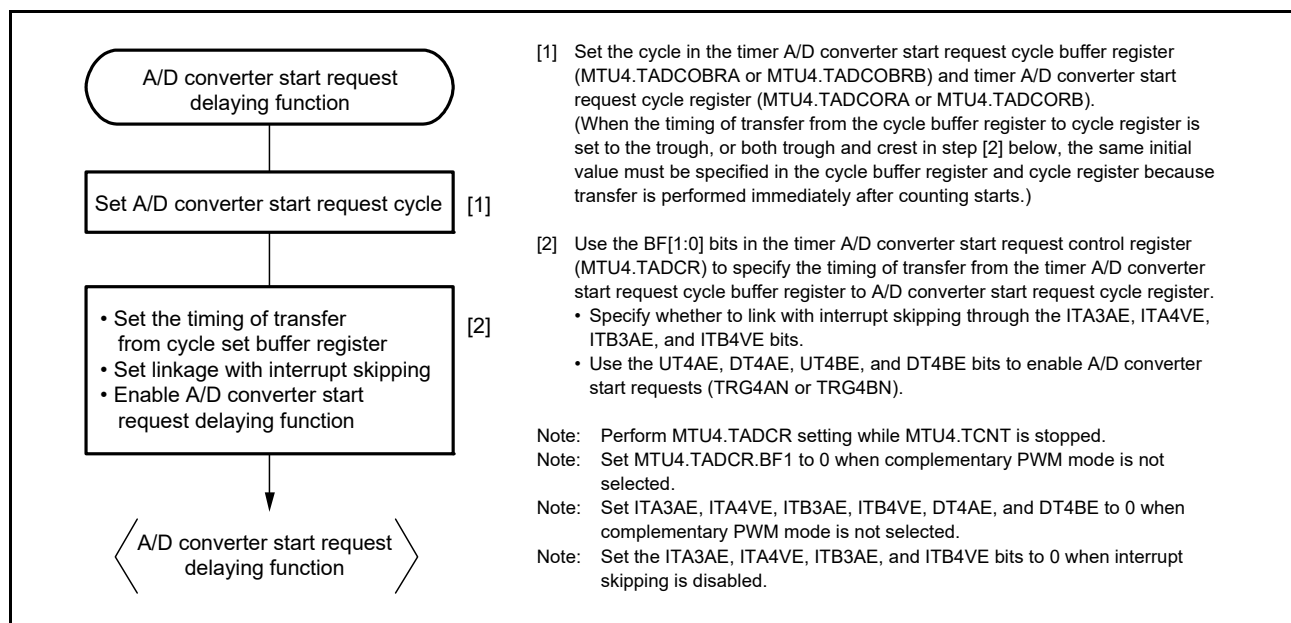
Figure 19.83 Example of Procedure for Specifying A/D Converter Start Request Delaying Function (MTU3 and MTU4)
