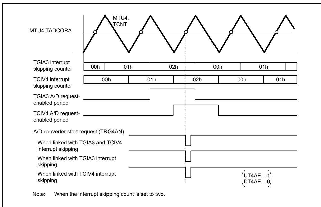
Figure 19.87 Example of A/D Converter Start Request Signal (TRG4AN) Operation Linked with Interrupt Skipping Function 1 (UT4AE = 1, DT4AE = 0)
