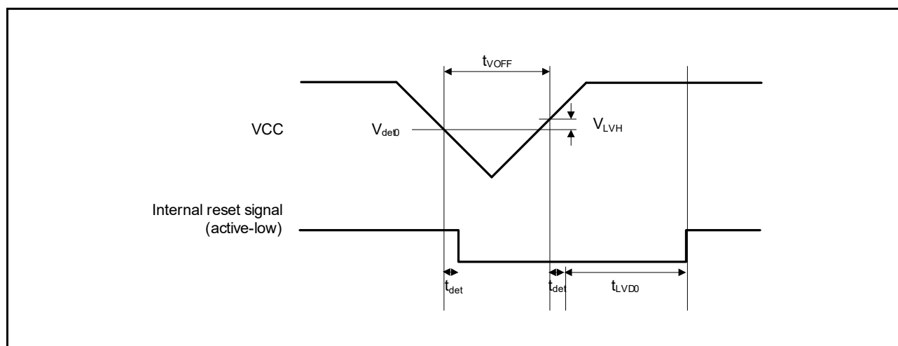
Figure 32.40 Voltage Detection Circuit Timing ( V_{det0} )
