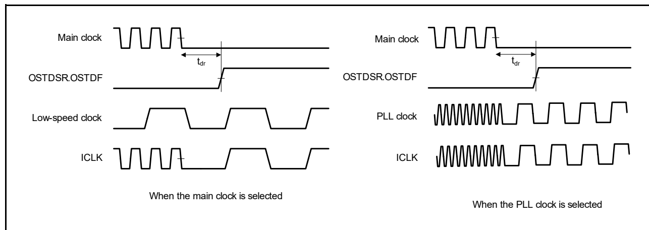
Figure 32.43 Oscillation Stop Detection Timing
