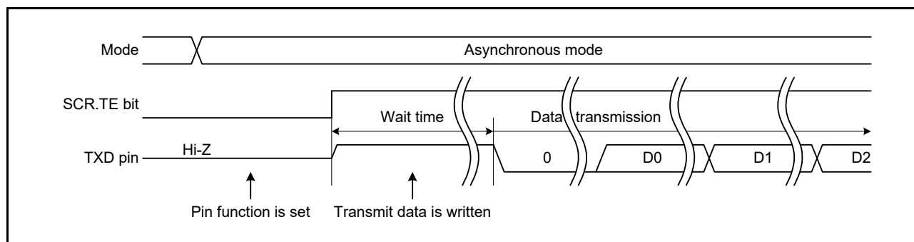
Figure 23.8 Example of Data Transmission Timing in Asynchronous Mode
