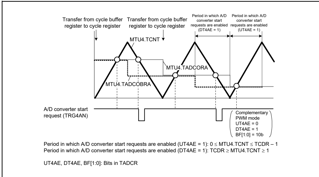
Figure 19.84 Basic Example of A/D Converter Start Request Signal (TRG4AN) Operation
