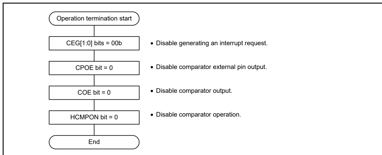
Figure 28.6 Comparator Operation Termination Flowchart
