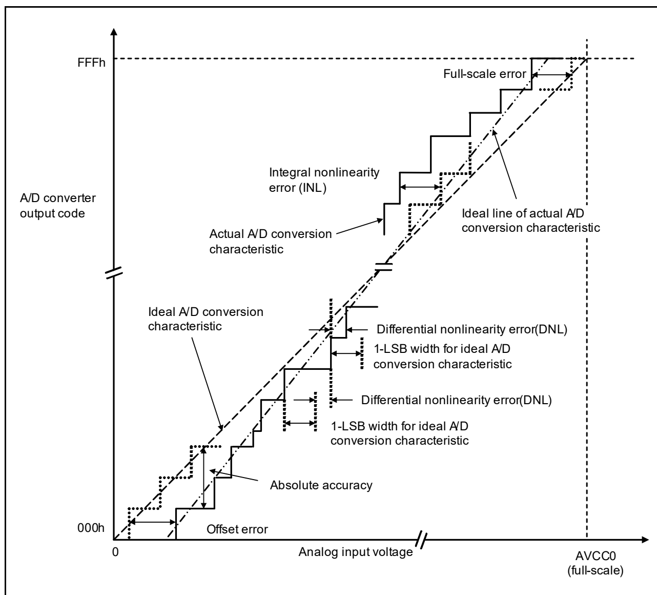
Figure 32.36 Illustration of A/D Converter Characteristic Terms
