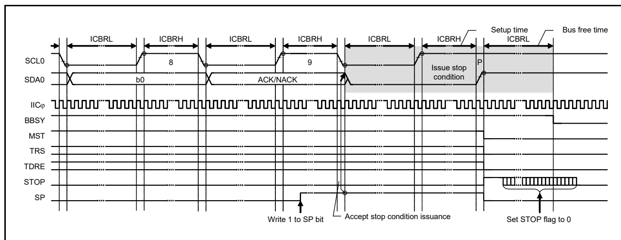
Figure 24.38 Stop Condition Issue Timing (SP Bit)
