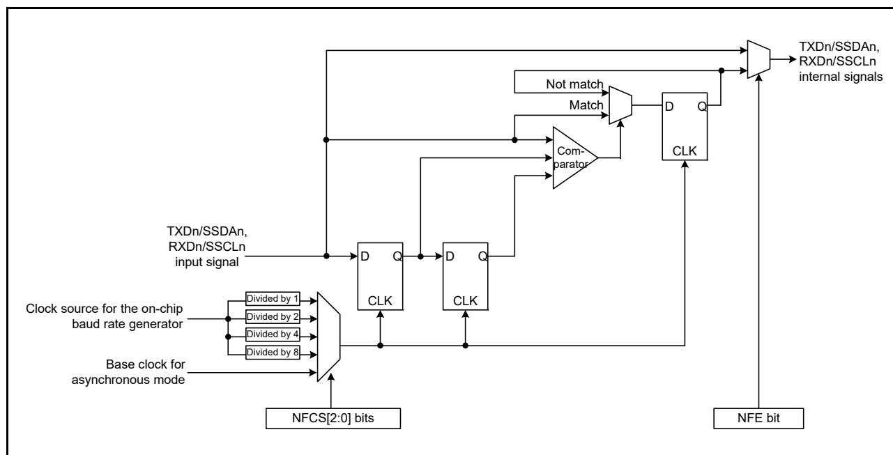
Figure 23.74 Block Diagram of Digital Noise Filter Circuit
