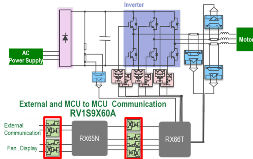
Figure 1. Inverter circuit of the general-purpose inverter.
