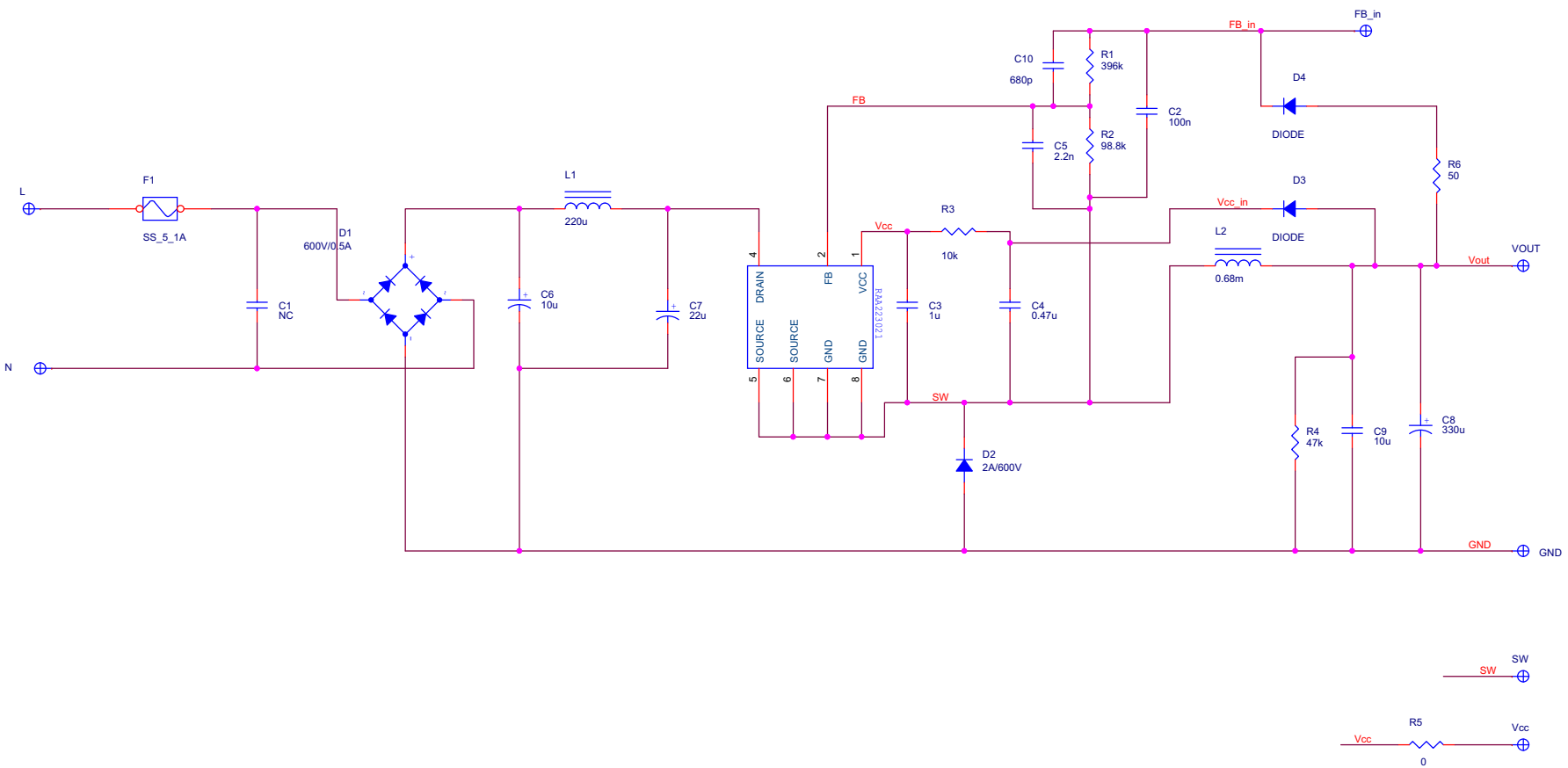
Figure 6. Schematic
