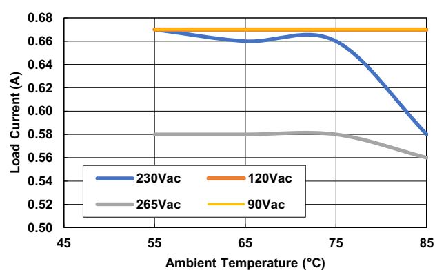
Figure 13. 3.3V Output Power Derating
