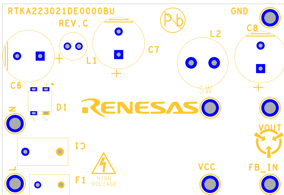
Figure 7. Top Layer
