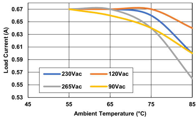
Figure 15. 9V Output Power Derating
