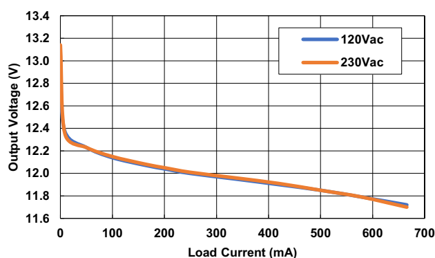
Figure 10. Load Regulation
