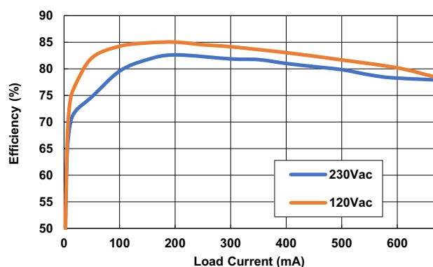
Figure 9. Efficiency
