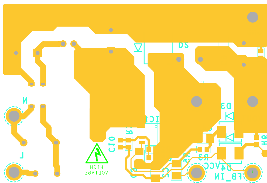
Figure 8. Bottom Layer
