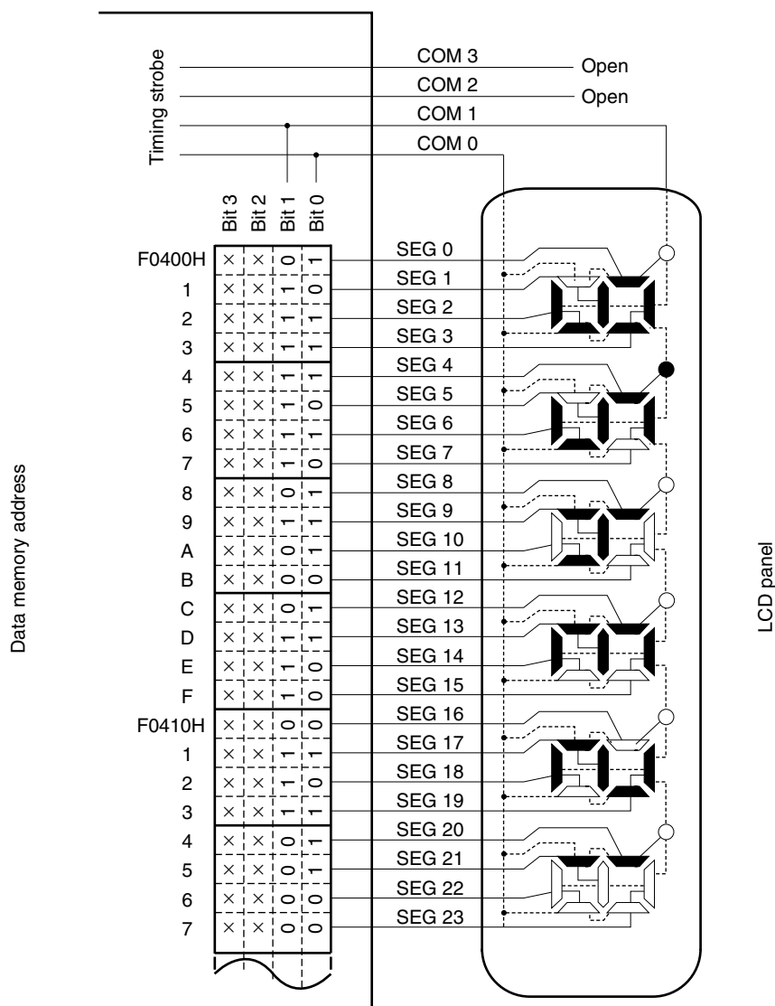
Figure 14-31. Example of Connecting Two-Time-Slice LCD Panel
