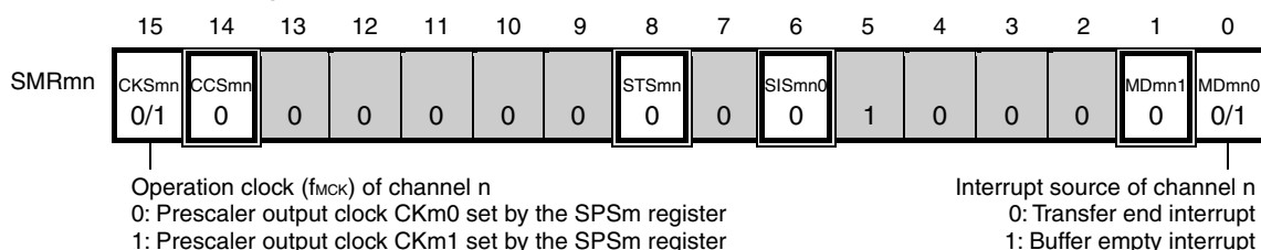
Figure 12-39. Example of Contents of Registers for Master Transmission/Reception of 3-Wire Serial I/O (CSI00, CSI01) (1/2)
