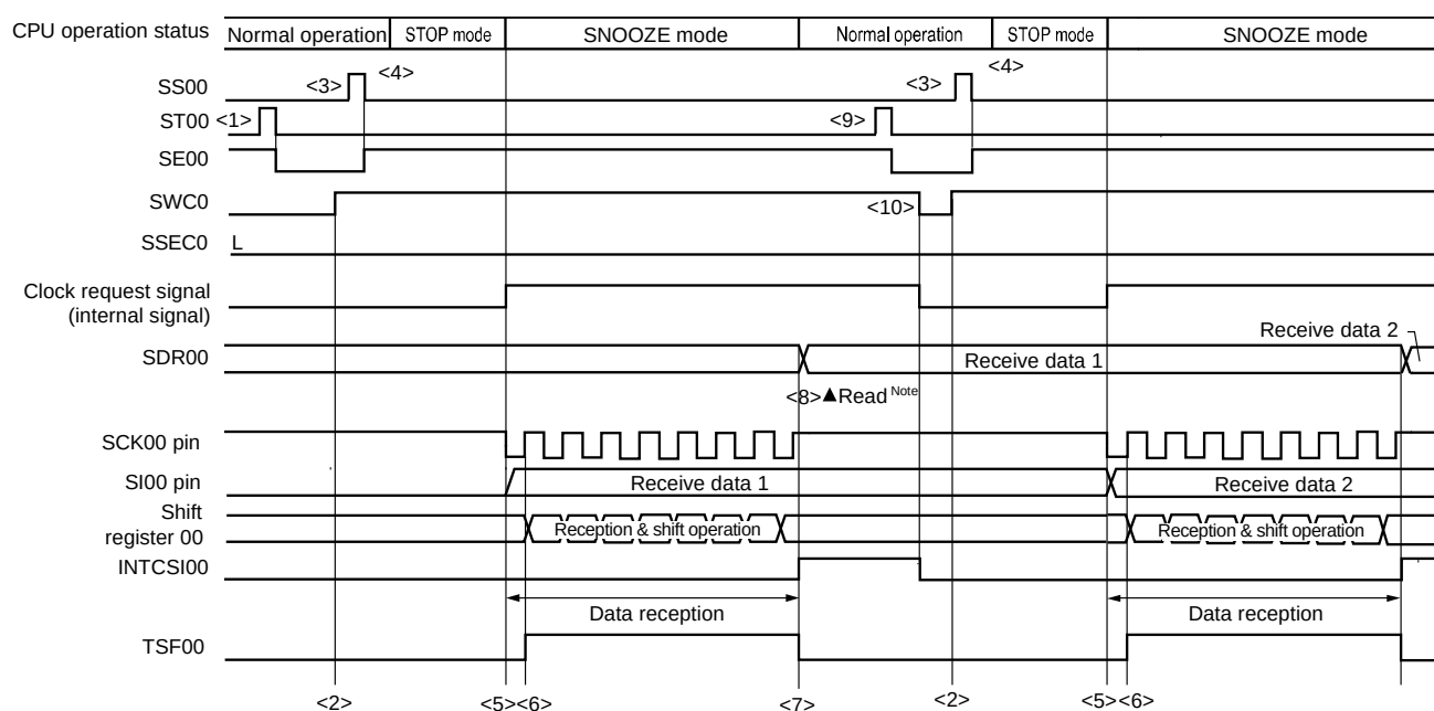
&lt;R&gt; Figure 12-71. Timing Chart of SNOOZE Mode Operation (continuous startup) (Type 1: DAPmn = 0, CKPmn = 0)
