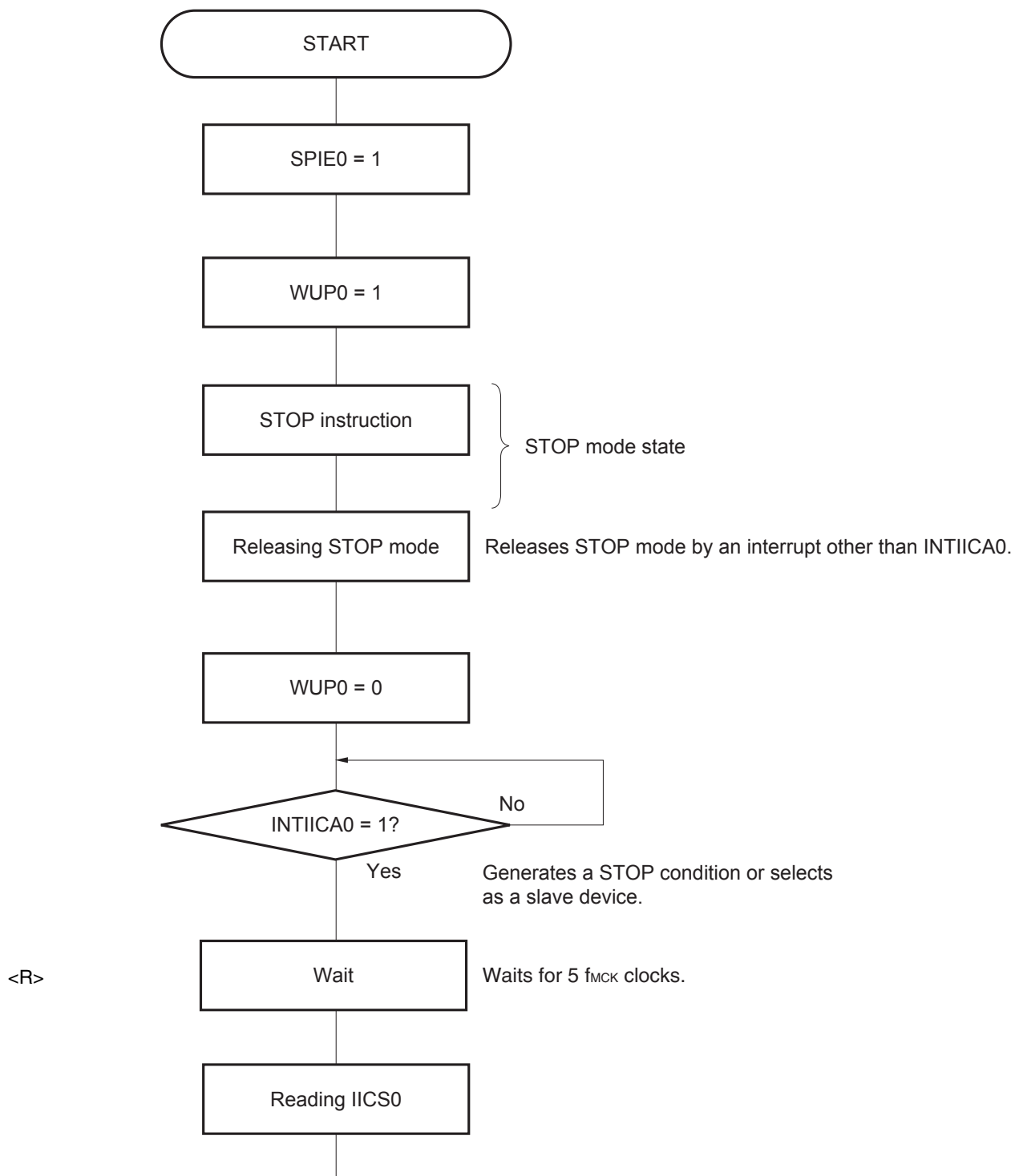
Figure 13-24. When Operating as Master Device after Releasing STOP Mode other than by INTIICA0
