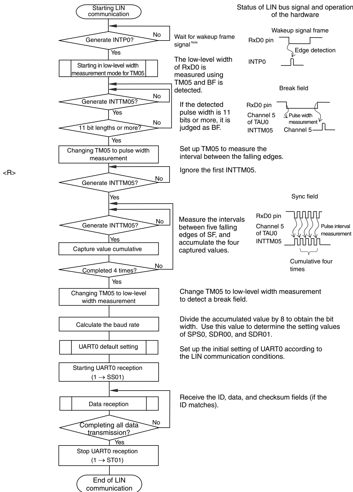
Figure 12-99. Flowchart for LIN Reception
