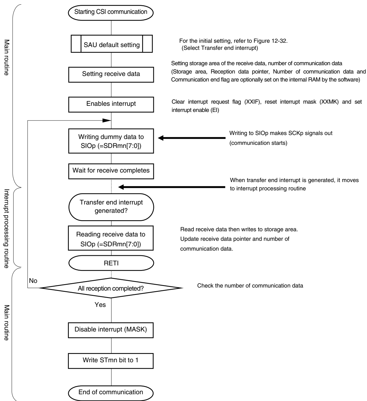
Figure 12-36. Flowchart of Master Reception (in Single-Reception Mode)
