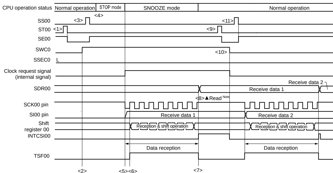
&lt;R&gt; Figure 12-69. Timing Chart of SNOOZE Mode Operation (once startup) (Type 1: DAPmn = 0, CKPmn = 0)
