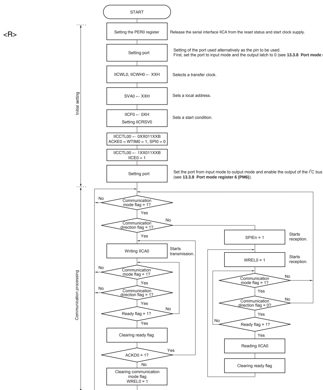
Figure 13-30. Slave Operation Flowchart (1)
