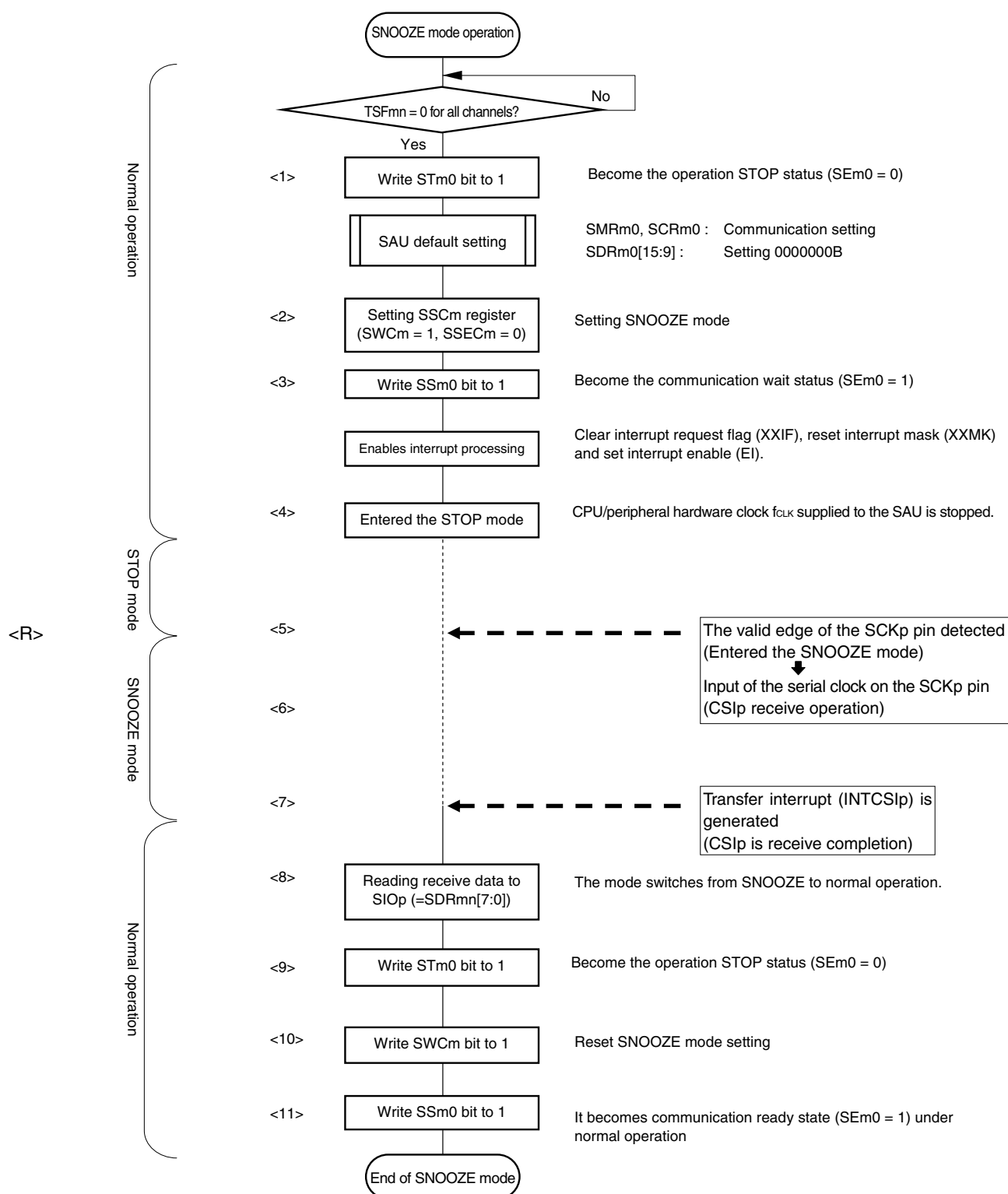
Figure 12-70. Flowchart of SNOOZE Mode Operation (once startup)
