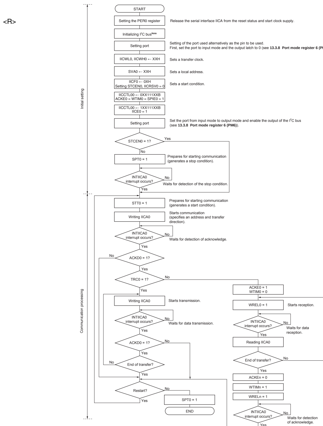
Figure 13-28. Master Operation in Single-Master System
