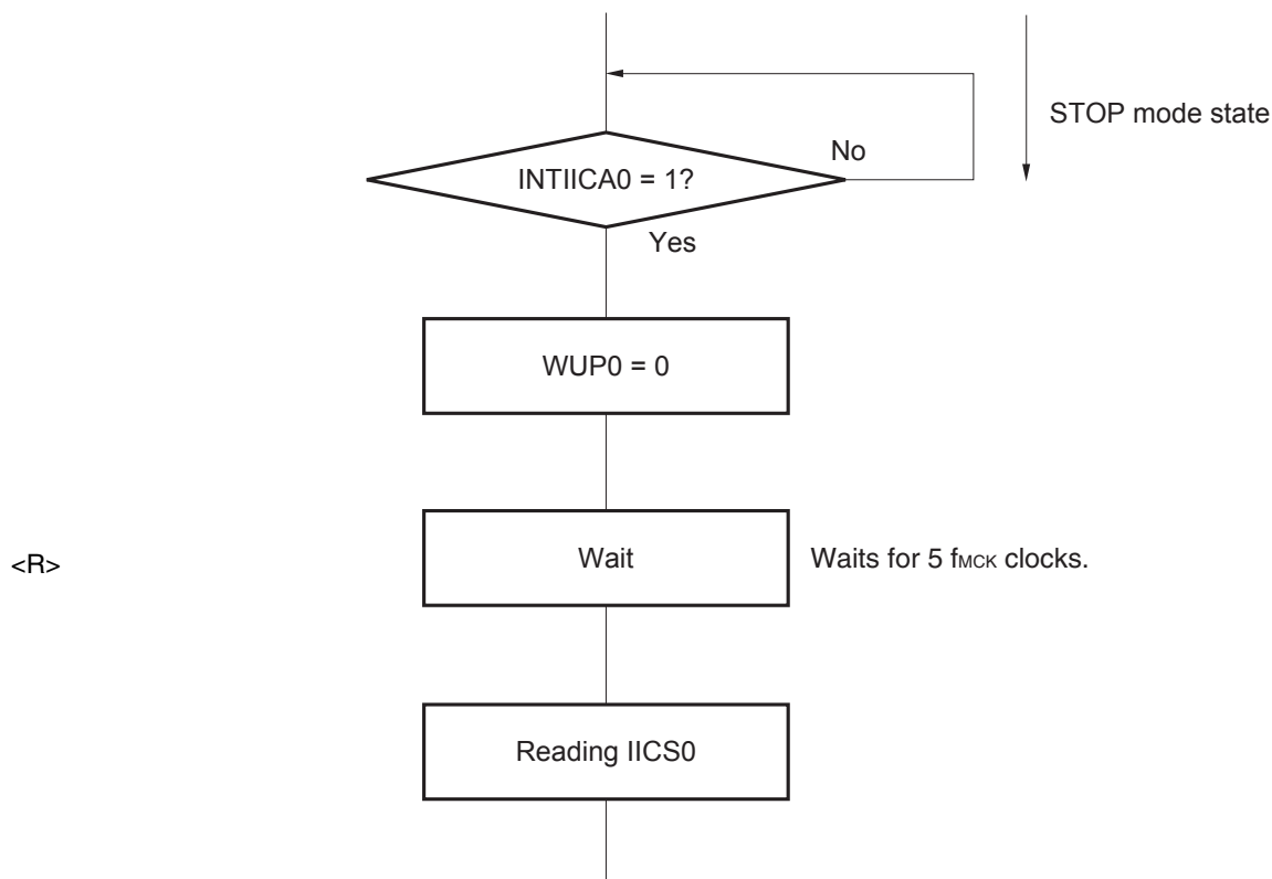
Figure 13-23. Flow When Setting WUP0 = 0 upon Address Match (Including Extension Code Reception)
