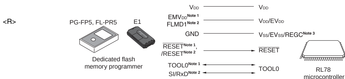
Figure 26-2. Communication with Dedicated Flash Memory Programmer
