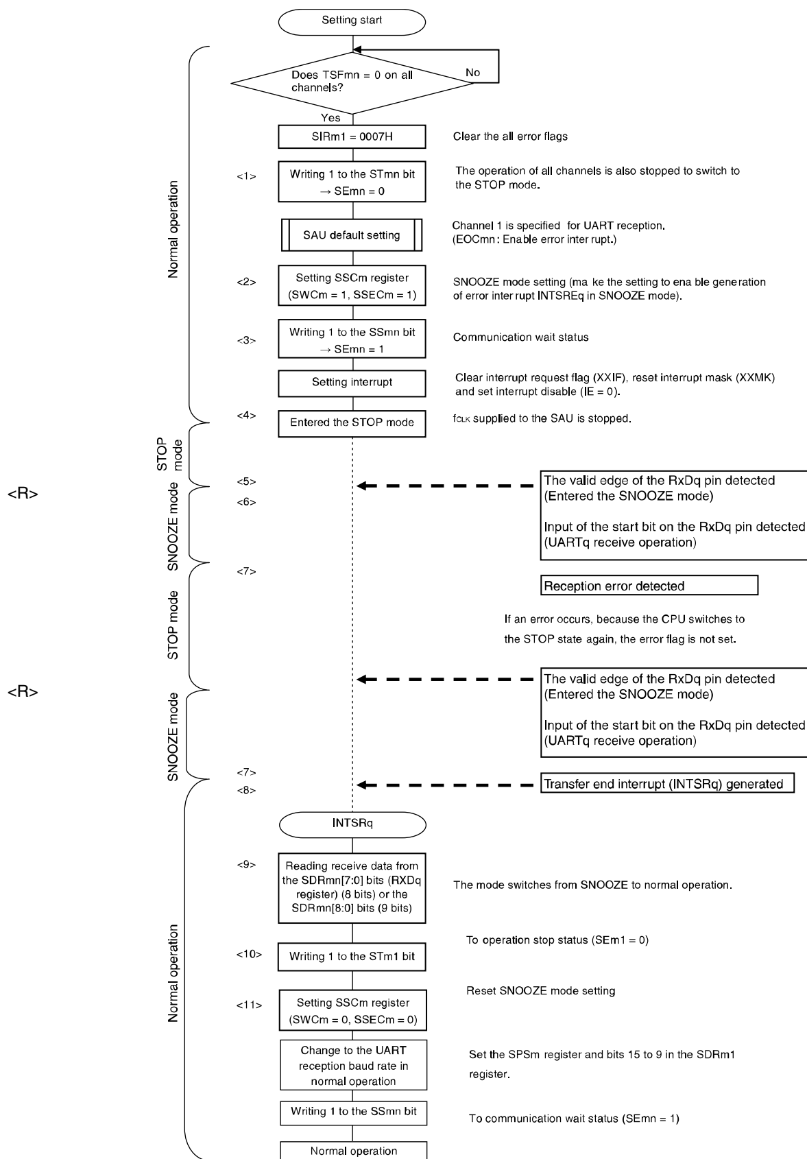
Figure 12-92. Flowchart of SNOOZE Mode Operation (EOCm1 = 1, SSECm = 1)
