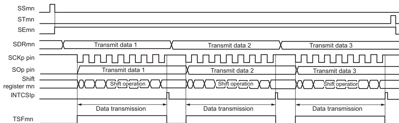
Figure 12-51. Timing Chart of Slave Transmission (in Single-Transmission Mode)
