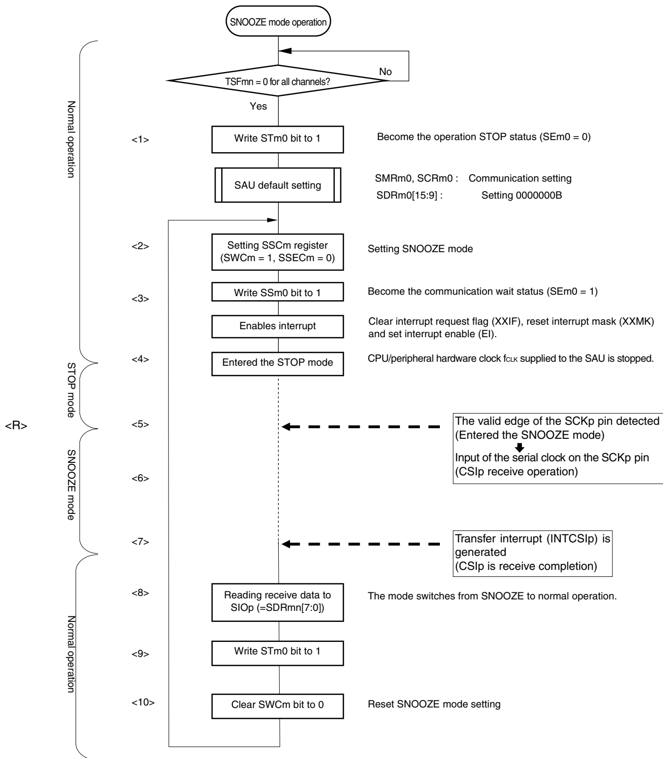
Figure 12-72. Flowchart of SNOOZE Mode Operation (continuous startup)
