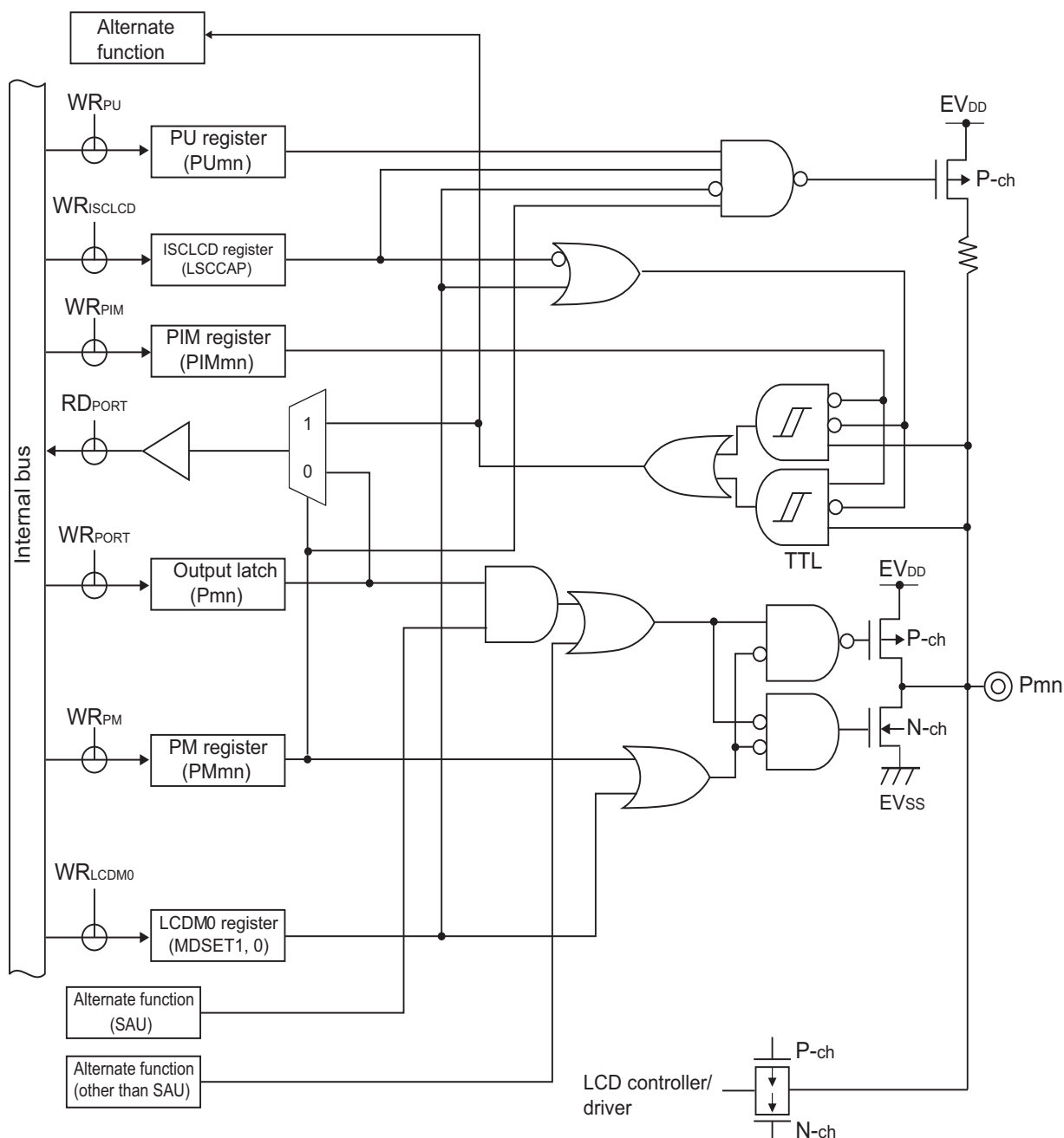
Figure 2-11. Pin Block Diagram for Pin Type 8-5-2
