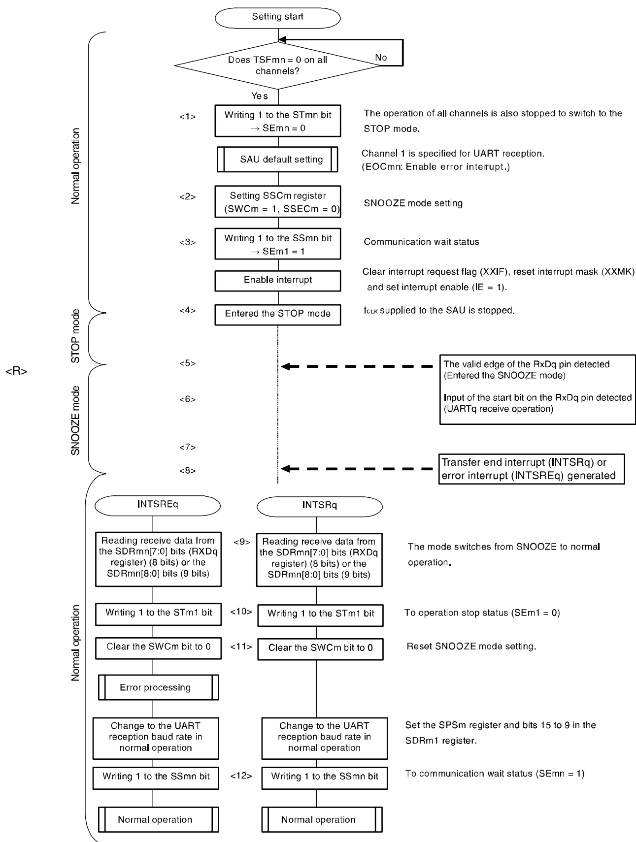
Figure 12-90. Flowchart of SNOOZE Mode Operation (EOCm1 = 0, SSECm = 0/1 or EOCm1 = 1, SSECm = 0)
