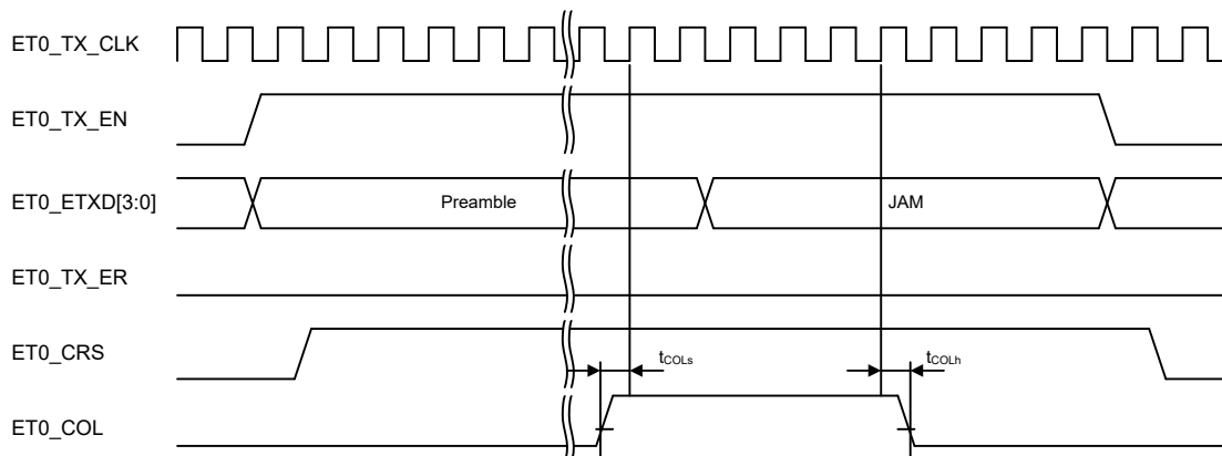
Figure 53.70 MII transmission timing when a conflict occurs
