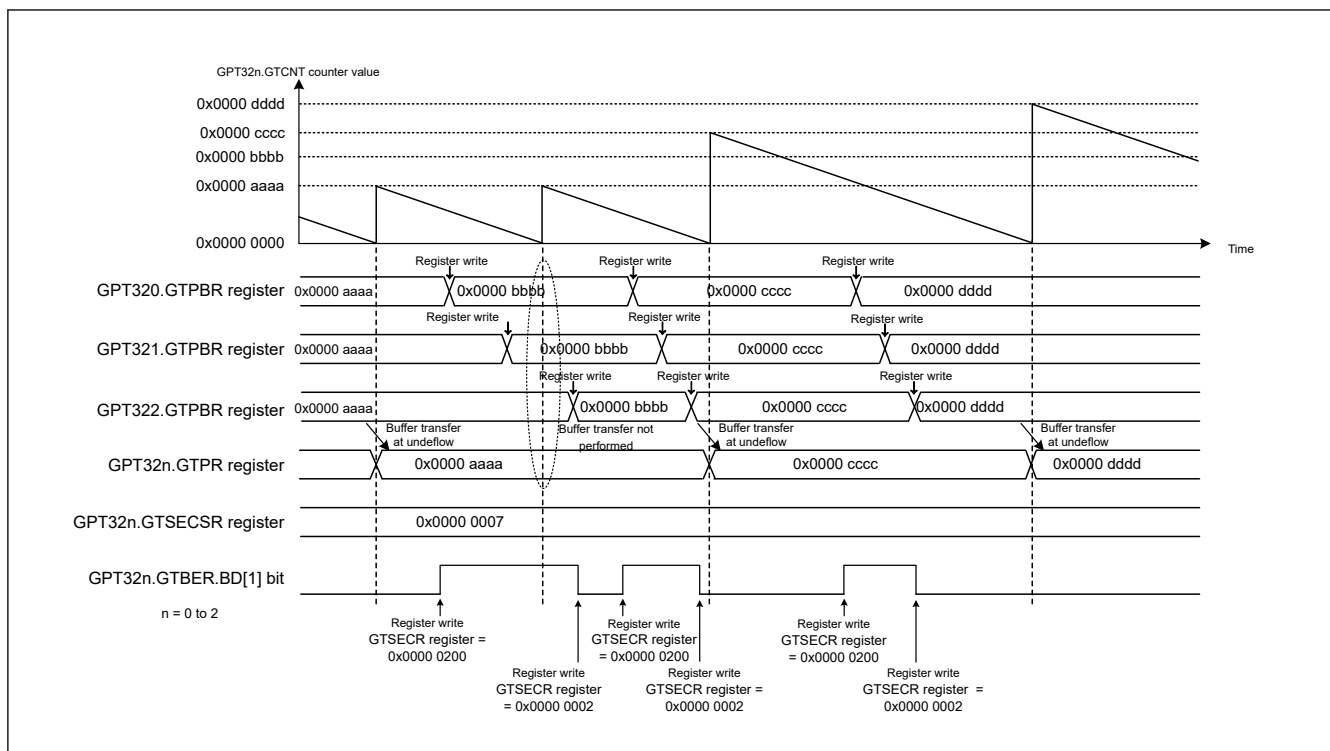
Figure 21.65 Example of Multiple Channel Operation for Disabling Buffer Operation (Saw Waves, Single Buffer Operation)
