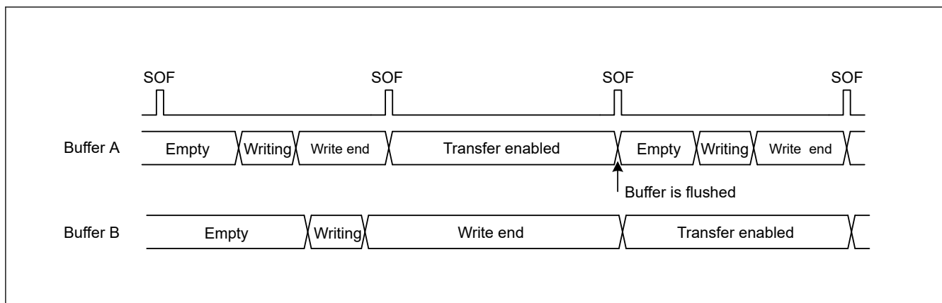
Figure 29.17 Example buffer flush operation
