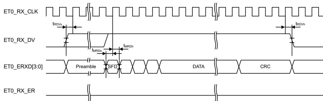
Figure 53.71 MII reception timing in normal operation
