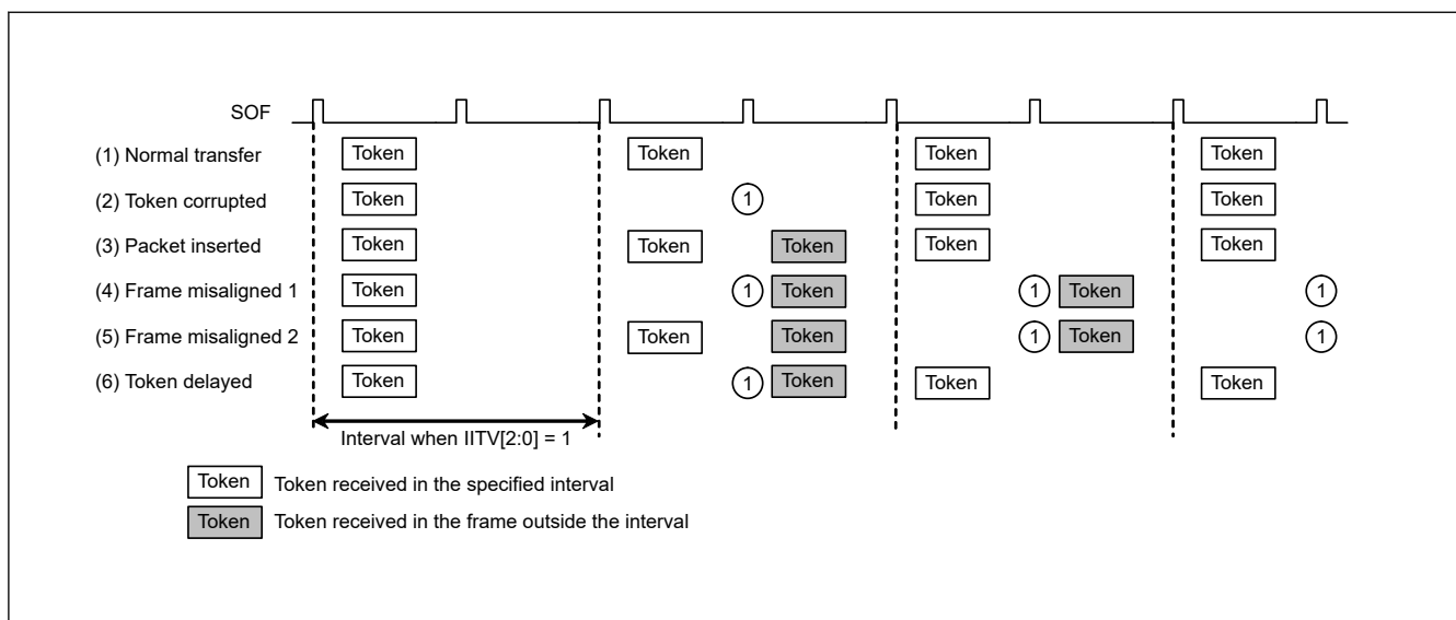
Figure 29.18 Example interval error occurrence when PIPEPERI.IITV[2:0] = 1
