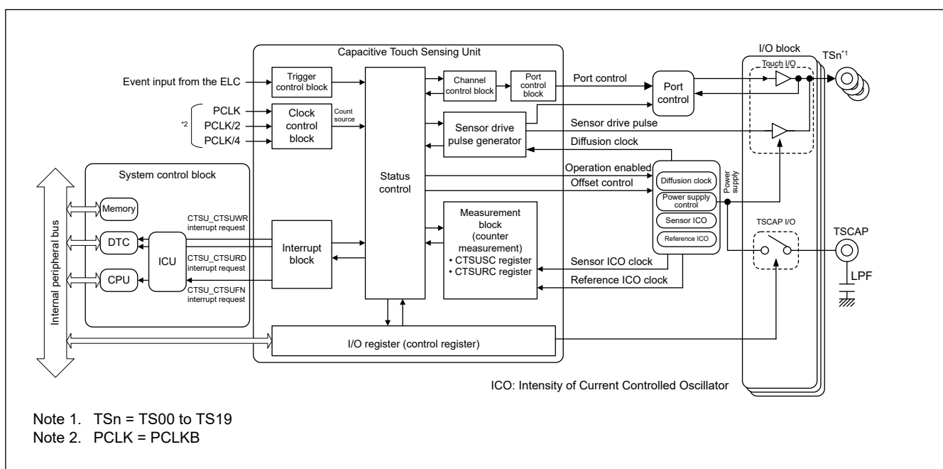
Figure 46.3 CTSU block diagram
