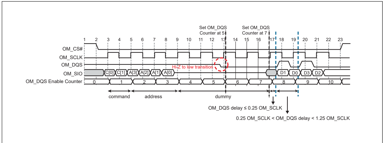
Figure 36.20 Timing example of OM_DQS clock input transitions from Hi-Z to Low (Flash DQPI mode, dummy cycle number = 4, OM_DQS pre-cycle on)
