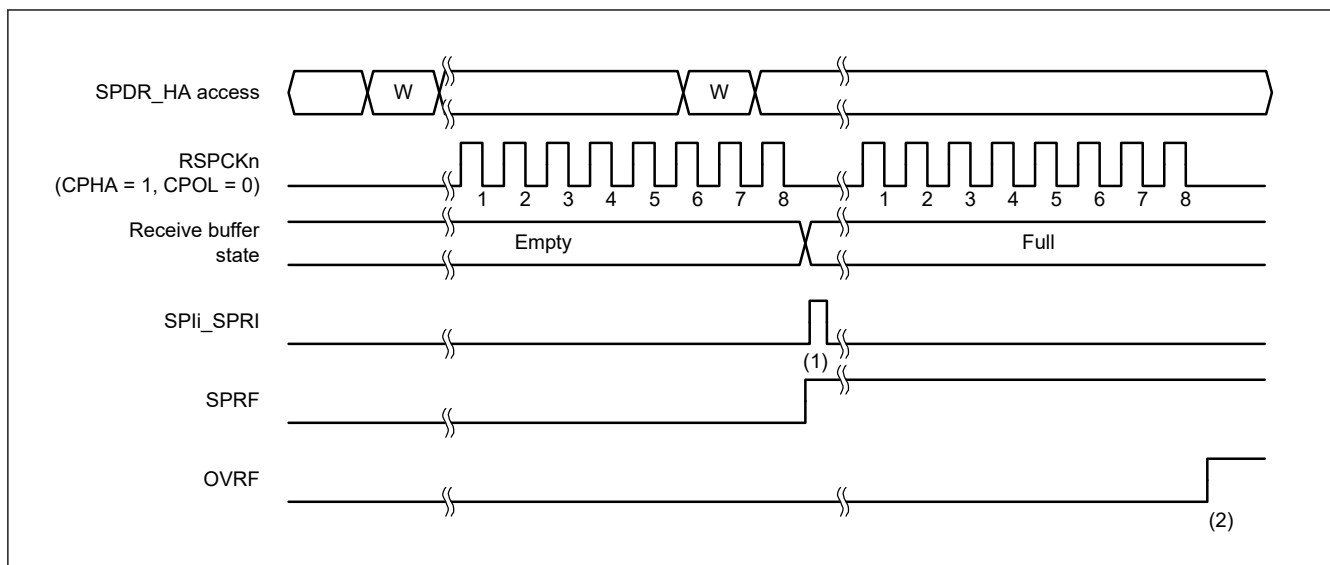
Figure 34.26 Operation example when SPCR3.ETXMD = 0 and SPCR.TXMD = 0
