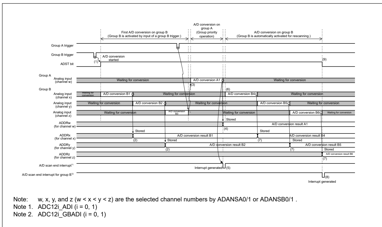
Figure 43.19 Example of group priority operation 1-1: Group A trigger input during group B scanning when rescanning is enabled (when ADGSPCR.GBRSCN = 1, ADGSPCR.GBRP = 0, and ADGSPCR.LGRRS = 0)
