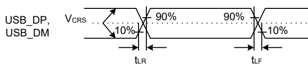
Figure 53.74 USB_DP and USB_DM output timing in low-speed mode
