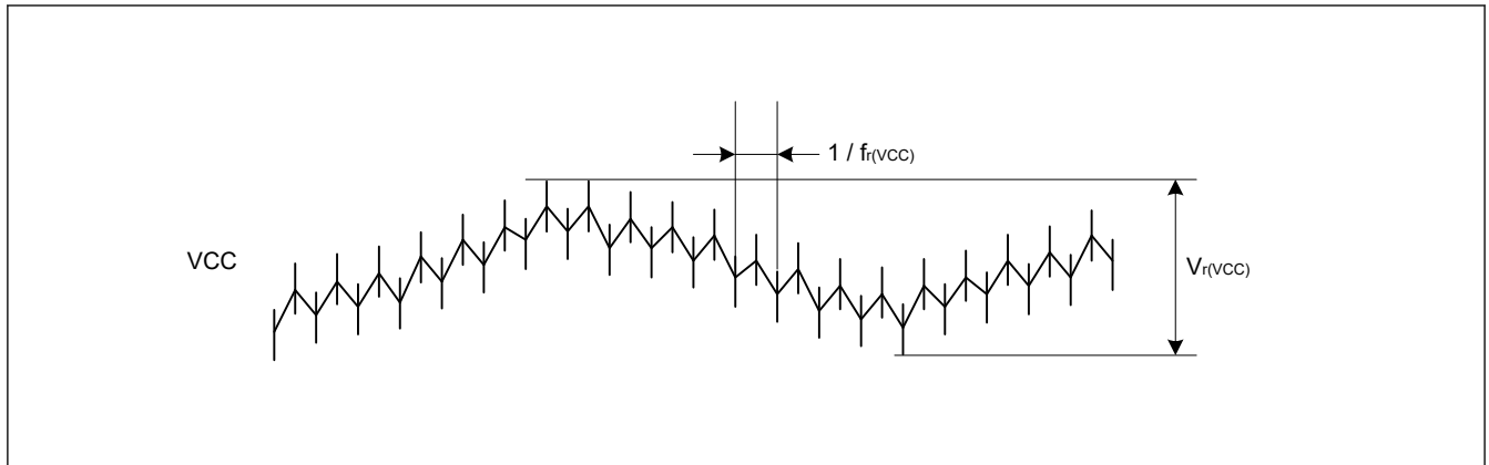
Figure 53.6 Ripple waveform
