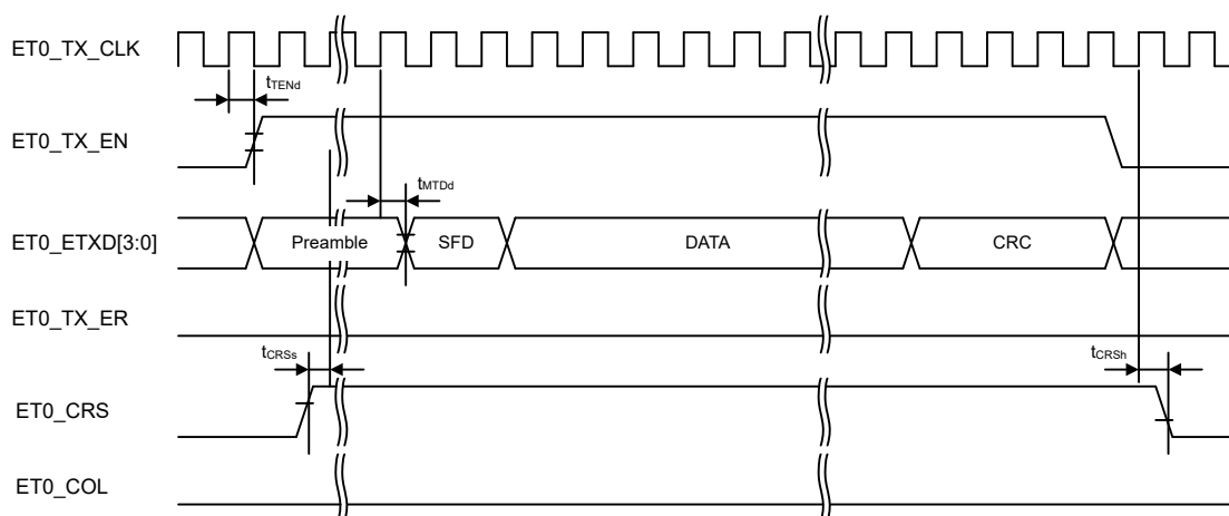
Figure 53.69 MII transmission timing in normal operation
