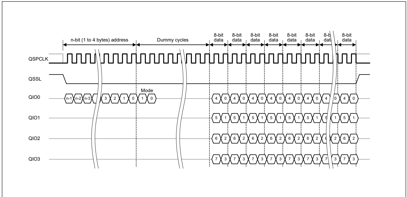
Figure 35.26 Fast Read Quad Output bus cycle in XIP mode (with extended SPI protocol)
