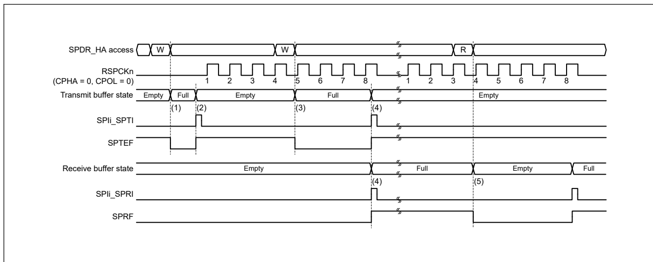
Figure 34.29 Operation example of the SPI1_SPTI and SPI1_SPRI interrupts when CPHA = 0 and CPOL = 0 in master mode
