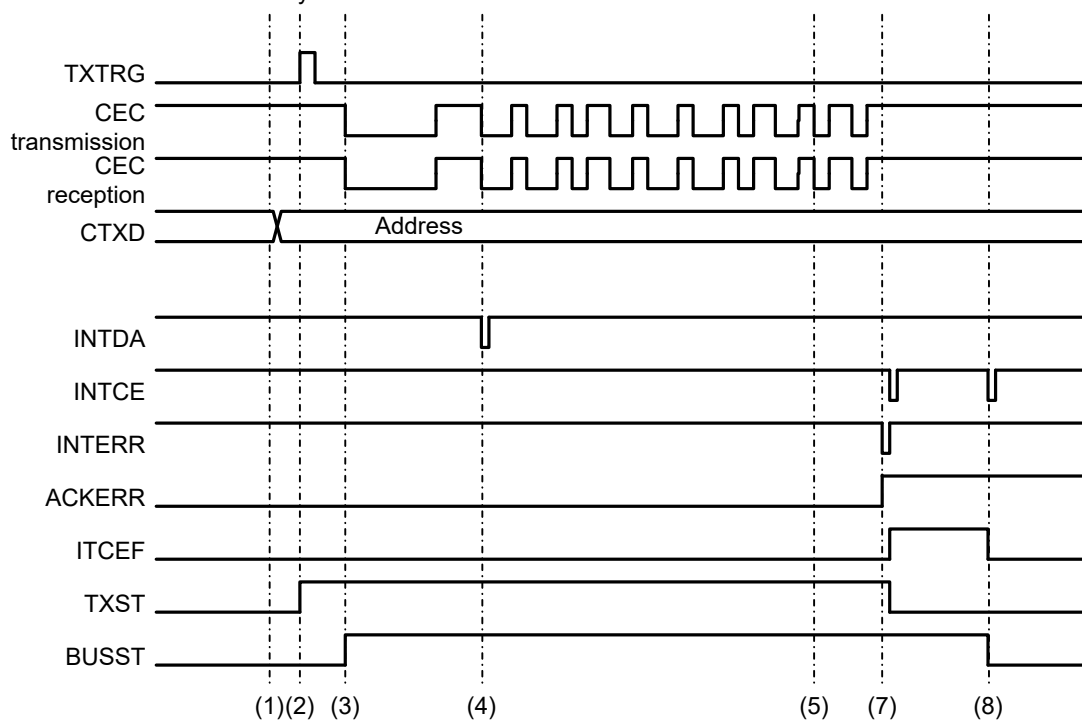
Figure 37.15 Logical allocation (CECCTL1.CESEL[1:0] = 00b)
