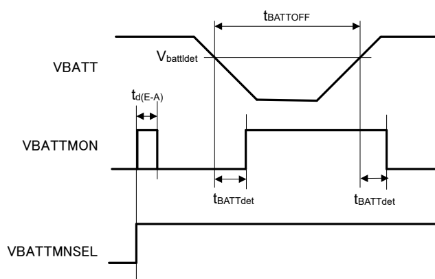
Figure 2.93 Battery backup function characteristics
