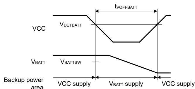
Figure 2.92 Battery backup function characteristics
