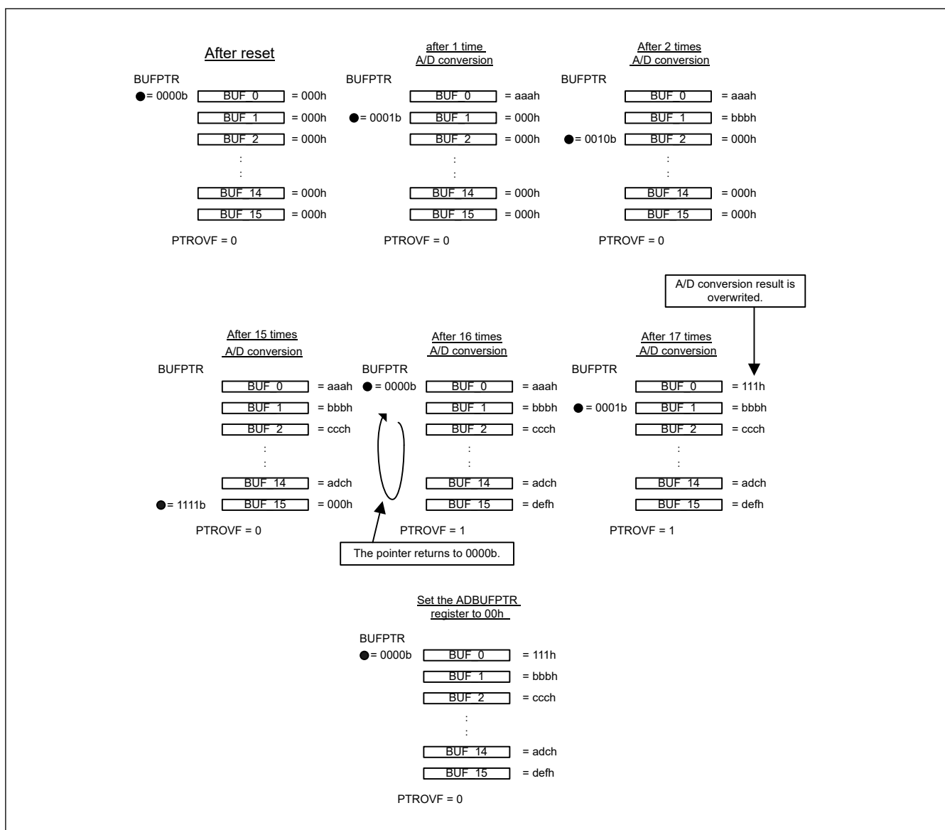
Figure 37.37 Data Buffers, Pointer, and Overflow Flag Operations
