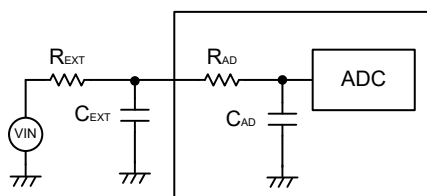
Figure 37.40 Sample and hold circuit simplified diagram
