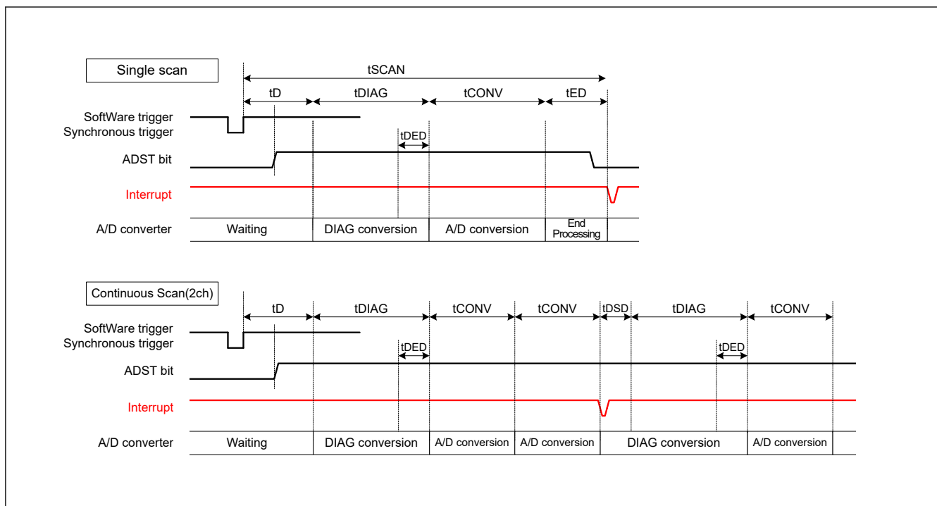
Figure 37.31 Scan conversion timing when activated by software or a synchronous trigger input (ELC)
