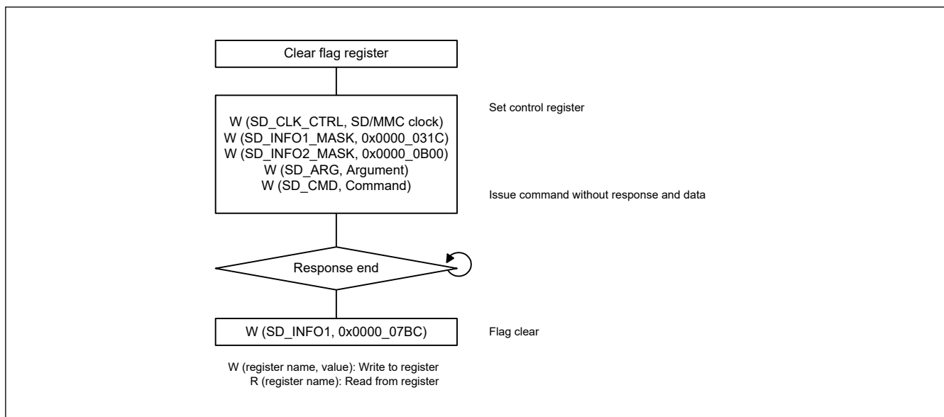
Figure 33.9 Example flow of command without response or data
