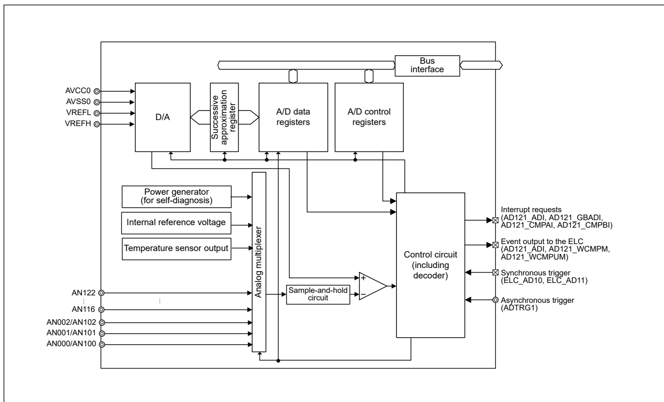
Figure 37.2 ADC12 block diagram (unit 1)
