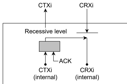
Figure 29.8 Connection when self-test mode 1 is selected ( i = 0, 1 )
