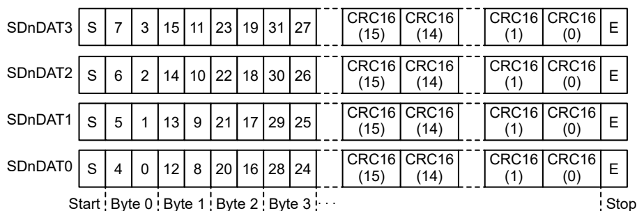
Figure 33.3 SDnDAT in 4-bit width mode
