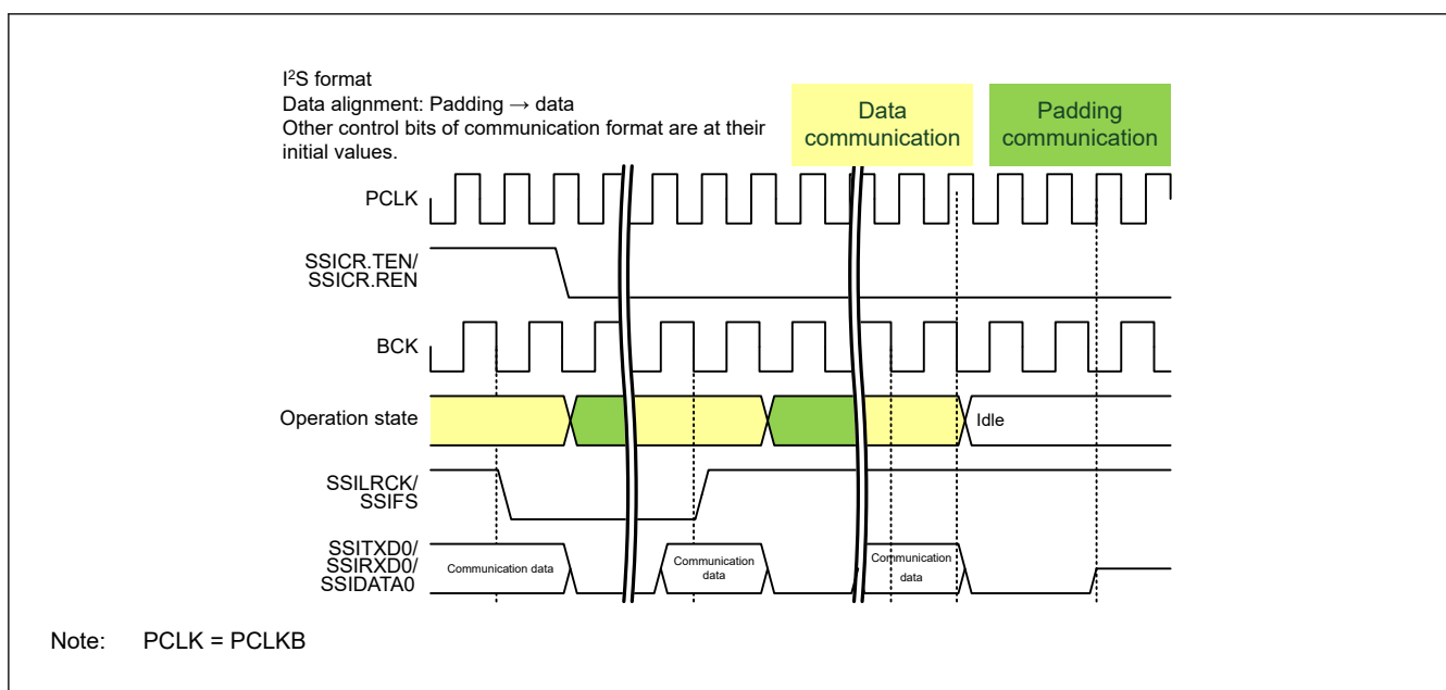
Figure 32.50 Halt from data communication (with padding bits)
