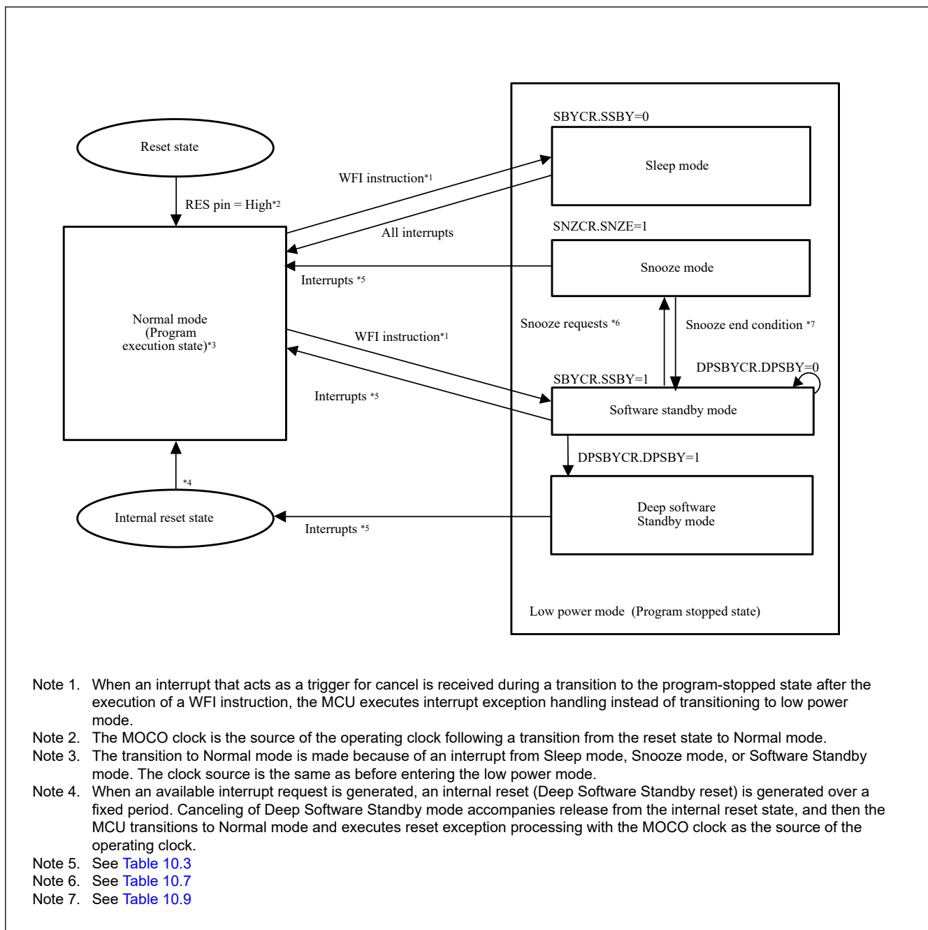
Figure 10.1 Mode Transitions
