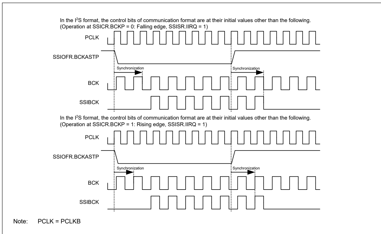
Figure 32.45 Example of stopping SSIBCK with SSIOFR.BCKASTP
