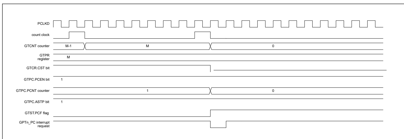
Figure 21.46 Example of the Timig of Operations for PWM Cycle Count Function (Saw-Wave One-Shot Pulse mode, Up-Counting)
