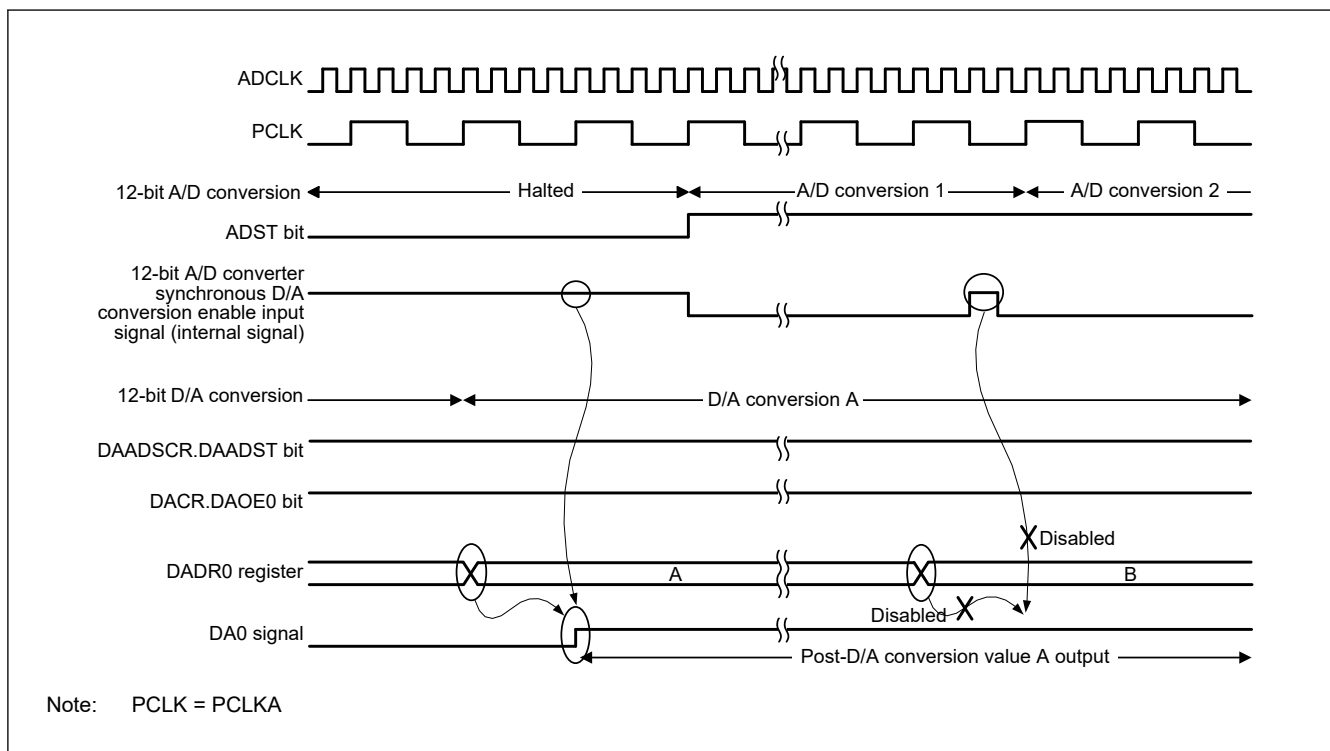
Figure 38.4 Example when the DAC12 cannot capture the synchronous D/A conversion enable input signal from the ADC12 (unit 1)
