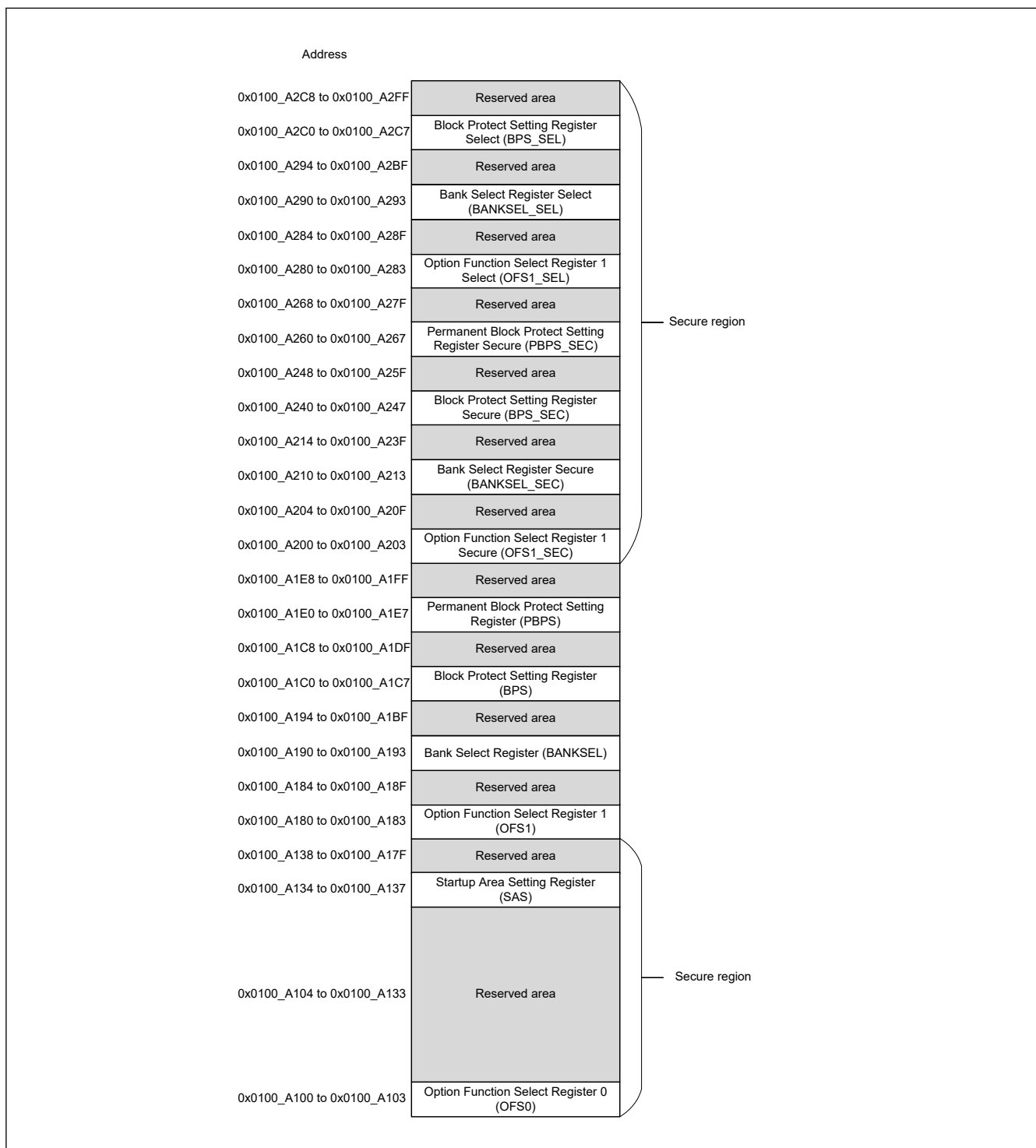
Figure 6.1 Option-setting memory area
