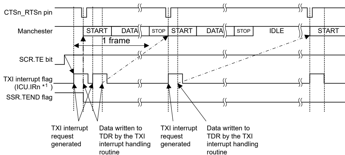
Figure 27.57 Example of Start-of-Transmission Operation for Serial Transmission in Manchester Mode (Without Preface but with the CTS Function)
