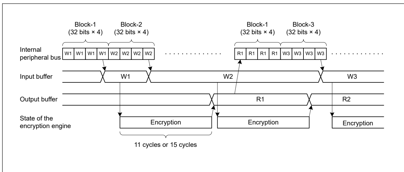
Figure 36.3 Encryption and decryption timing (AES)
