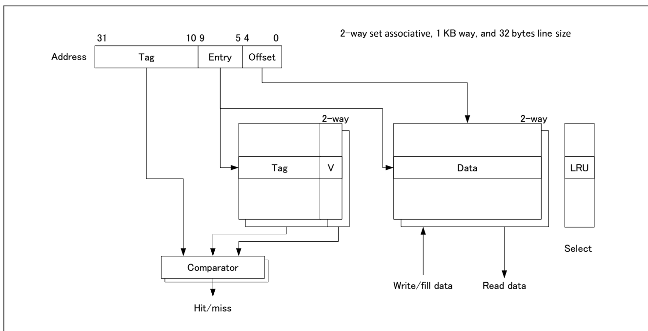
Figure 14.5 Cache structure for 2-way set associative of 2 KB capacity and 32 bytes line size
