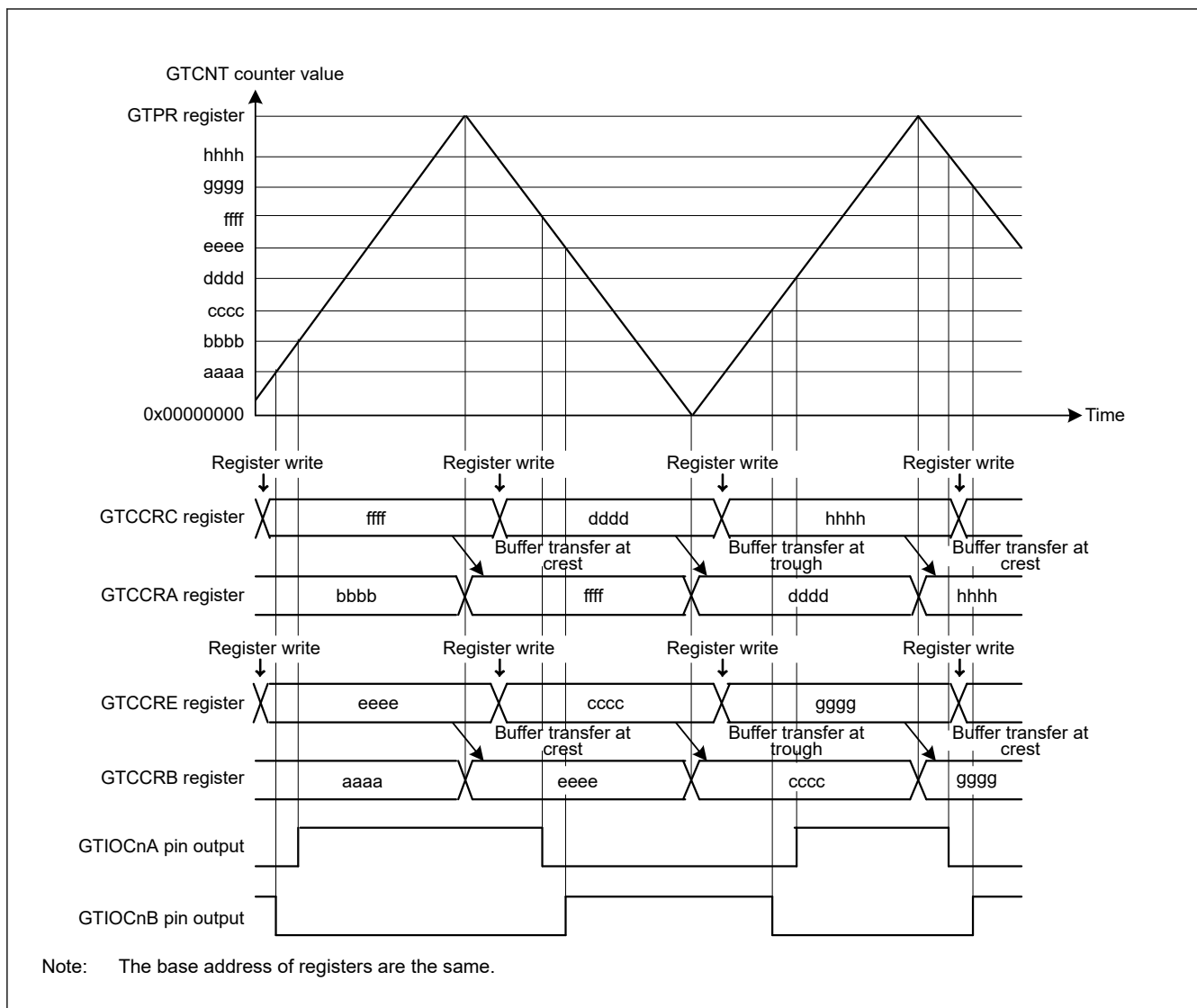
Figure 21.22 Example of triangle-wave PWM mode 2 operation with buffer operation, low output from the GTIOCA pin and high output from the GTIOCB pin at count start, output toggled at GTCCRA/ GTCCRB compare match, and output retained at cycle end
