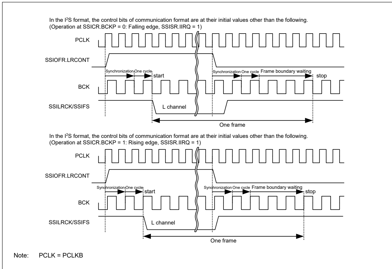
Figure 32.44 Example of disabling LR clock/frame synchronization continuation by SSIOFR.LRCONT
