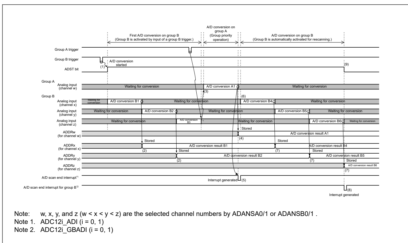
Figure 37.19 Example of group priority operation 1-1: Group A trigger input during group B scanning when rescanning is enabled (when ADGSPCR.GBRSCN = 1, ADGSPCR.GBRP = 0, and ADGSPCR.LGRRS = 0)
