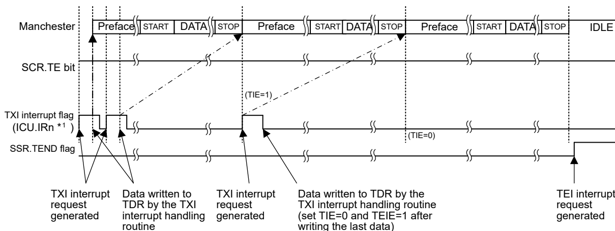
Figure 27.58 Example of End-of-Transmission Operation for Serial Transmission in Manchester Mode (with Preface but Without the CTS Function)
