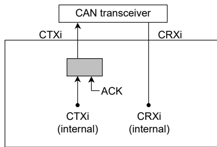
Figure 29.7 Connection when self-test mode 0 is selected ( i = 0, 1 )
