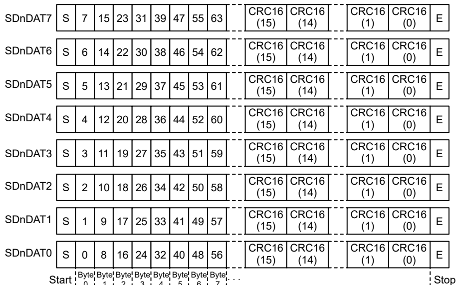
Figure 33.4 SDnDAT in 8-bit width mode
