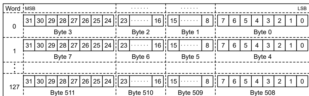
Figure 33.5 SD_BUF store data
