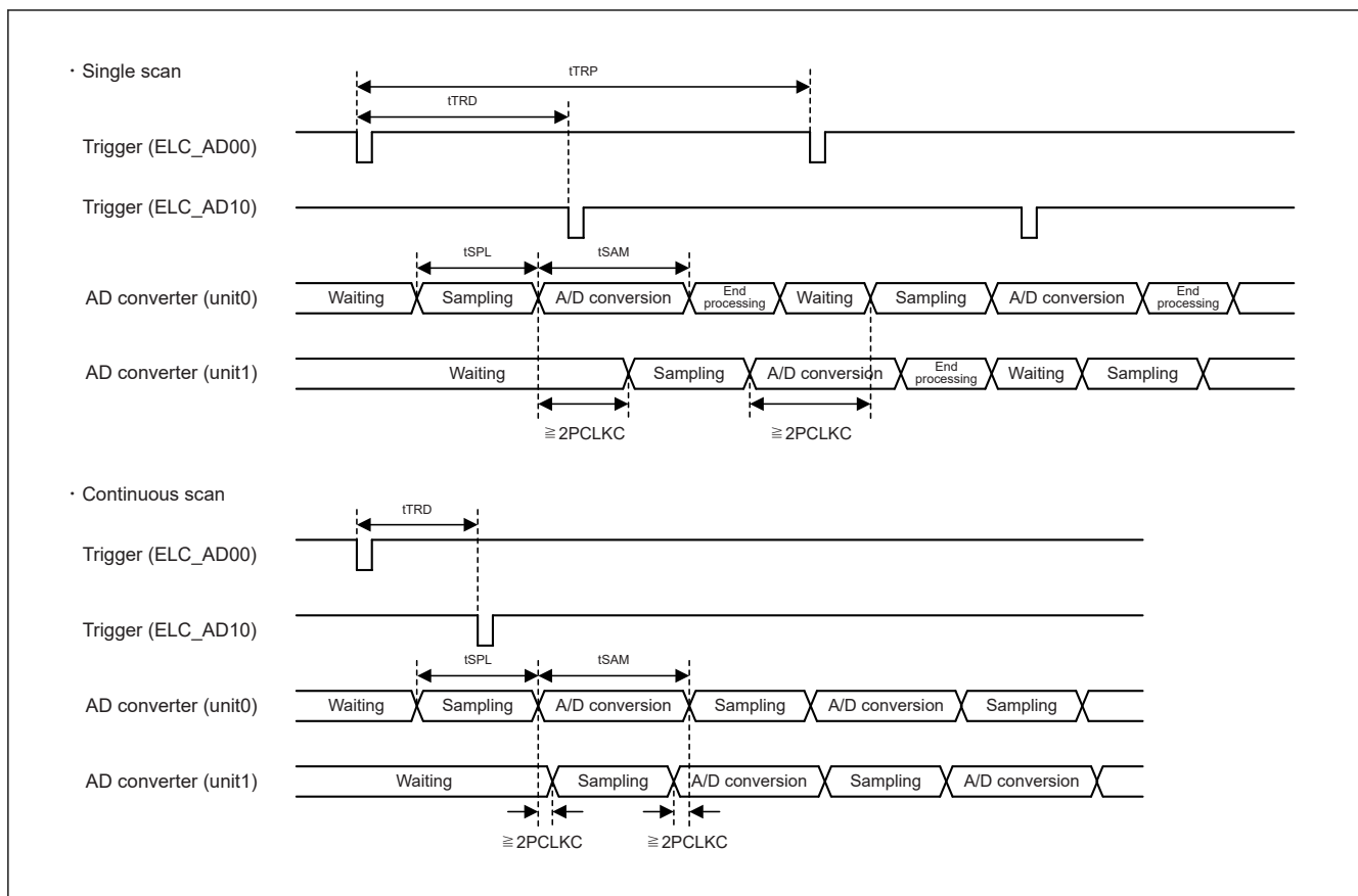
Figure 37.24 Trigger input timing in interleaved operation
