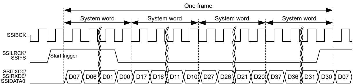
Figure 32.41 TDM format (without padding: system word length = data word length)
