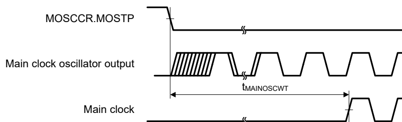
Figure 47.8 Main clock oscillation start timing
