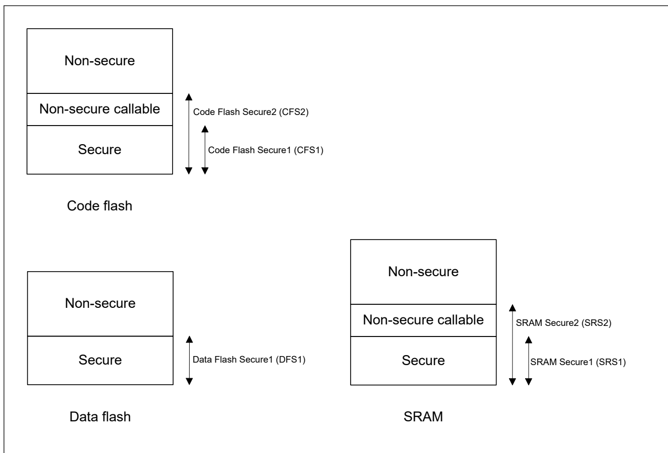
Figure 46.1 Memory mapping
