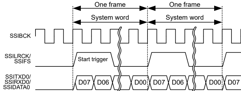
Figure 32.40 Long frame in monaural format (without padding)
