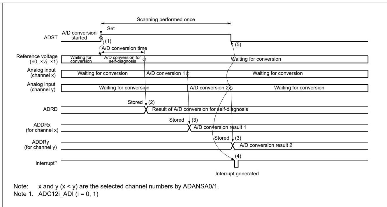
Figure 37.9 Example basic operation in single scan mode when the analog inputs (channel x and y) are selected with self-diagnosis
