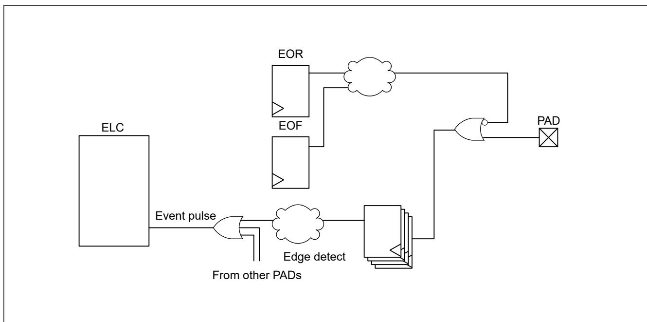
Figure 19.4 Generation of event pulse
