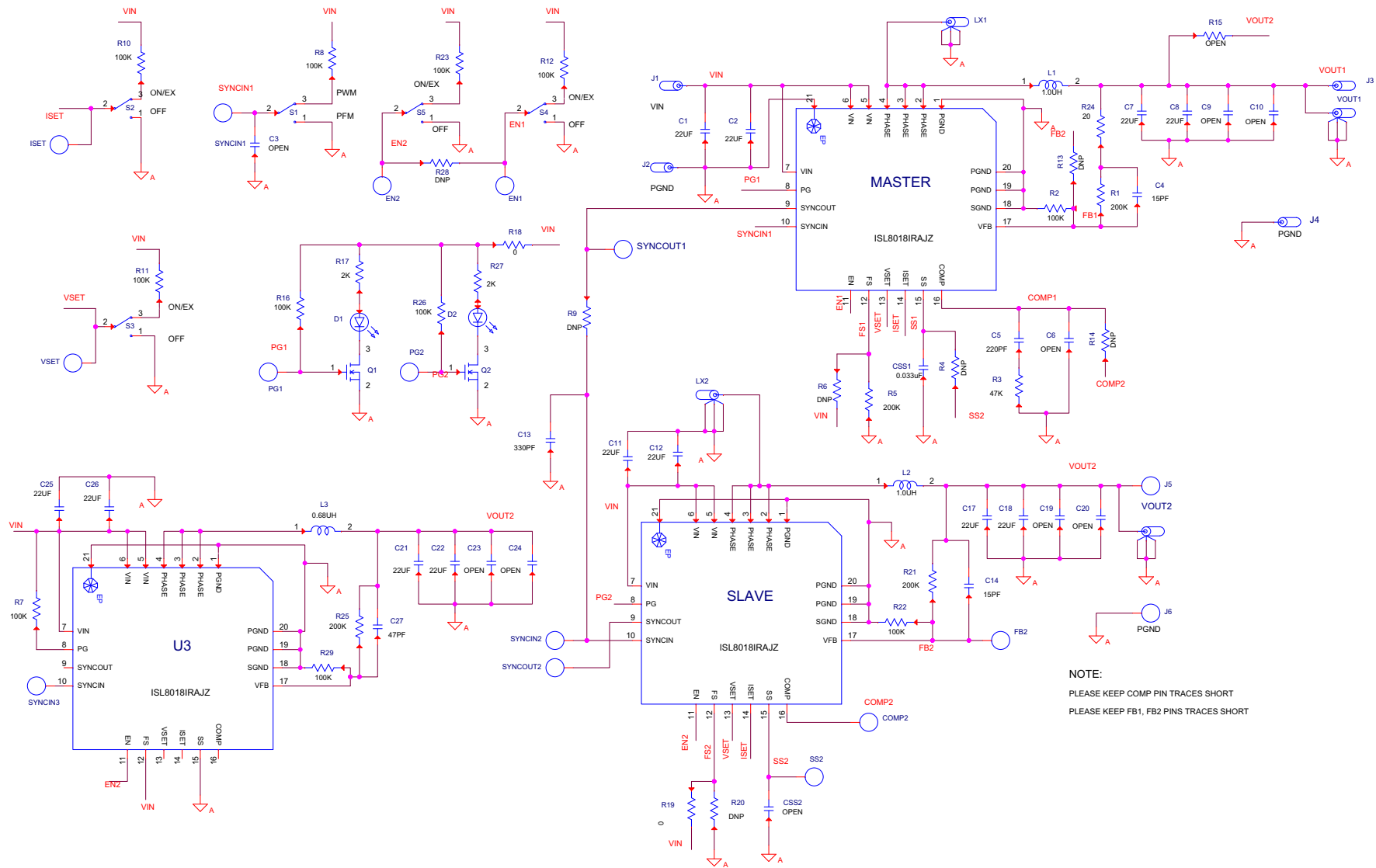
FIGURE 4. ISL8018EVAL3Z SCHEMATIC
