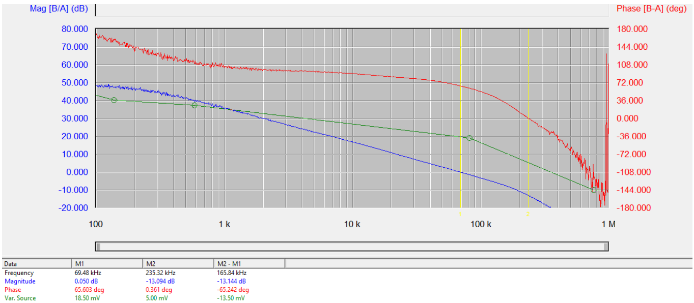
FIGURE 17. BODE PLOT 5.5V_{IN}/1.2V_{OUT} WITH FULL LOAD, R_3 = 70k , C_5 = 220pF , C_{OUT} = 144\mu F (EFFECTIVE CAPACITANCE), C_4 = 33pF , L = 1\mu H
