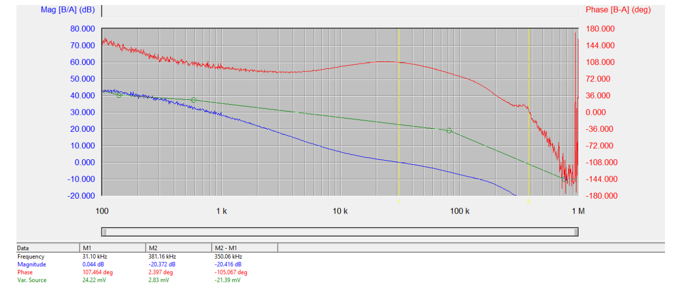
FIGURE 16. BODE PLOT 5.5V_{IN}/3.3V_{OUT} WITH FULL LOAD, R_3 = 25k , C_5 = 470pF , C_{OUT} = 100\mu F (EFFECTIVE CAPACITANCE), C_4 = 47pF , L = 2.2\mu H
