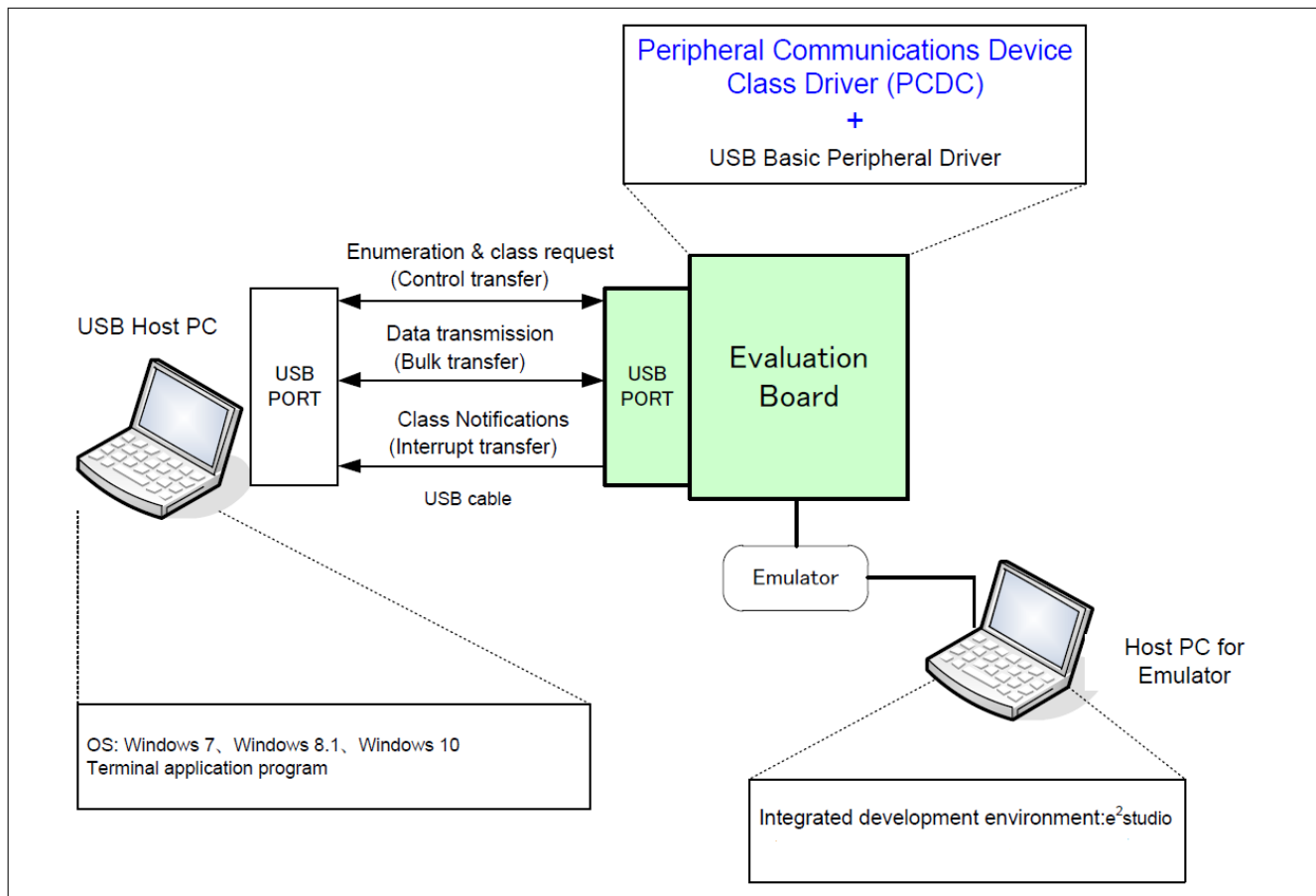
Figure 129: Example Operating Environment
