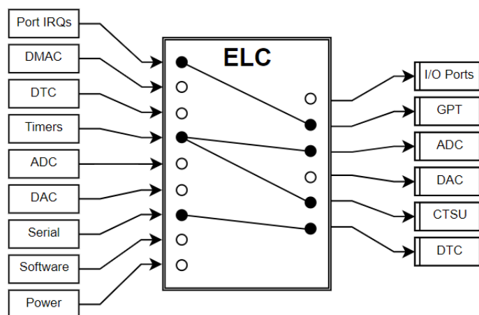
Figure 112: Event Link Controller Conceptual Diagram
