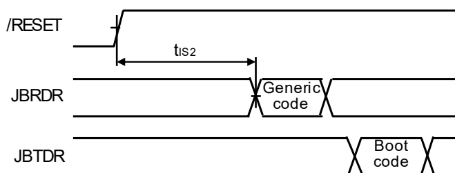
JTAG/SWD communication initial setting time
