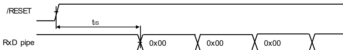
USB communication
