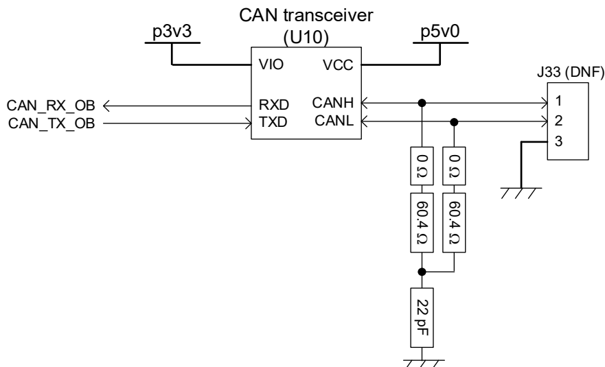
Figure 7-11 Configuration of CAN Interface Circuit
