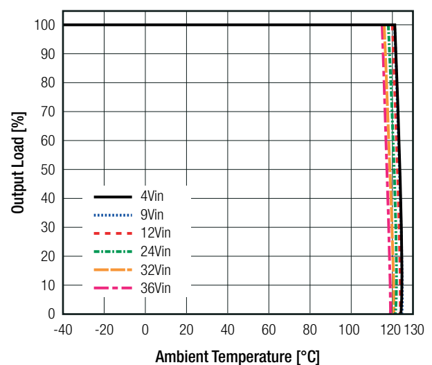
Thermal Derating
