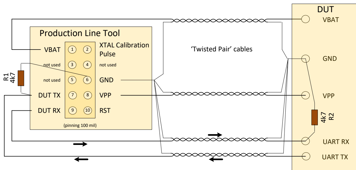
Figure 124: Location of Pull-Down Resistors
