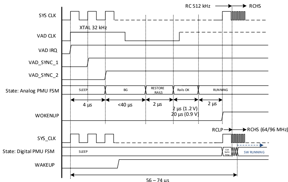
Figure 11: VAD WAKEUP Timing Diagram
