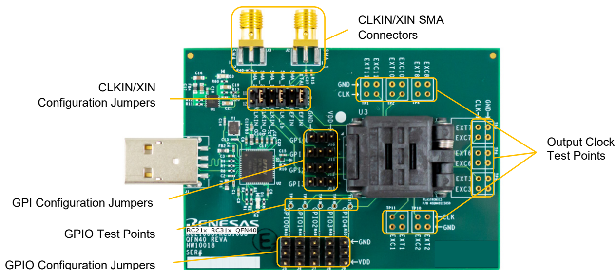
Figure 2. Programmer Board with Labels
